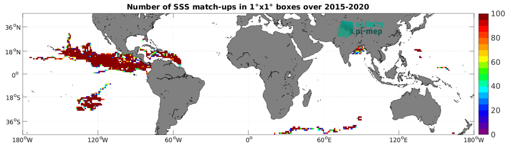
Figure 4: Number of SSS match-ups between Surface drifters SSS and the SMAP SSS L2 v5.3 (RSS) SSS product for the Mid-Low Latitudes 45N-45S Pi-MEP region over 1^\circ \times 1^\circ boxes and for the full satellite product period.
