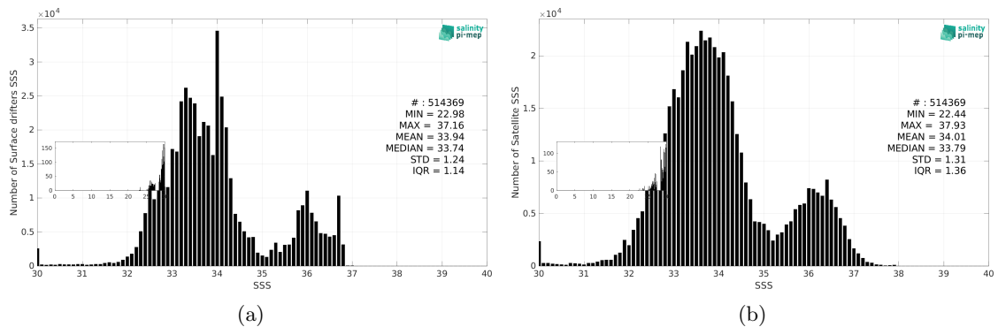
Figure 3: Histograms of SSS from Surface drifters (a) and SMAP SSS L2 v5.3 (RSS) (b) considering all match-up pairs per bins of 0.1 over the Mid-Low Latitudes 45N-45S Pi-MEP region and for the full satellite product period.
