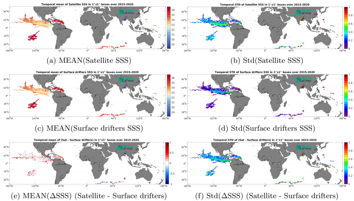
Figure 6: Temporal mean (left) and Std (right) of SSS from SMAP SSS L2 v5.3 (RSS) (top), Surface drifters (middle), and of \Delta SSS (Satellite - Surface drifters). Only match-up pairs are used to generate these maps.
