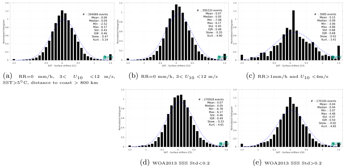
Figure 14: Normalized histogram of \Delta SSS (SMAP SSS L2 v5.3 (RSS) - Surface drifters) for 5 different subdatasets corresponding to: RR=0 mm/h, 3 < U_{10} < 12 m/s, SST>5°C, distance to coast > 800 km (a), RR=0 mm/h, 3 < U_{10} < 12 m/s (b), RR>1mm/h and U_{10} < 4 m/s (c), WOA2013 SSS Std<0.2 (d), WOA2013 SSS Std>0.2 (e).
