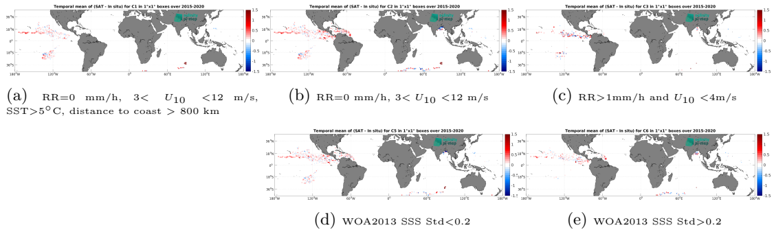
Figure 13: Temporal mean gridded over spatial boxes of size 1^\circ \times 1^\circ of \Delta SSS (SMAP SSS L2 v5.3 (RSS) - Surface drifters) for 5 different subdatasets corresponding to:RR=0 mm/h, 3 < U_{10} < 12 m/s, SST>5°C, distance to coast > 800 km (a), RR=0 mm/h, 3 < U_{10} < 12 m/s (b), RR>1mm/h and U_{10} < 4 m/s (c), WOA2013 SSS Std<0.2 (d), WOA2013 SSS Std>0.2 (e).
