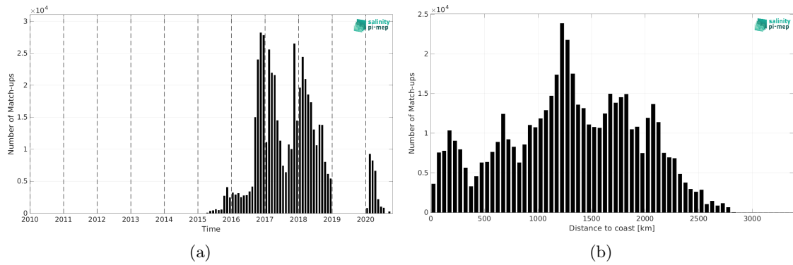
Figure 2: Number of match-ups between Surface drifters and SMAP SSS L2 v5.3 (RSS) SSS as a function of time (a) and as function of the distance to coast (b) over the Mid-Low Latitudes 45N-45S Pi-MEP region and for the full satellite product period.
