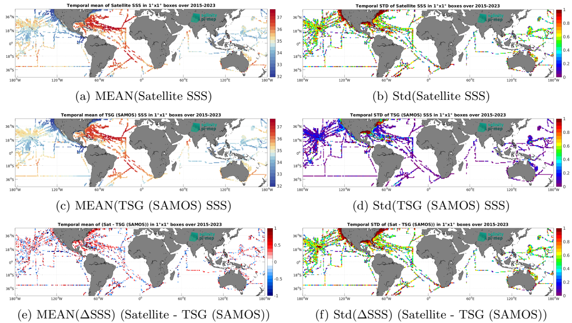
Figure 7: Temporal mean (left) and Std (right) of SSS from SMAP SSS L2 v5.3 - 40 km (RSS) (top), TSG (SAMOS) (middle), and of \Delta SSS (Satellite - TSG (SAMOS)). Only match-up pairs are used to generate these maps.
