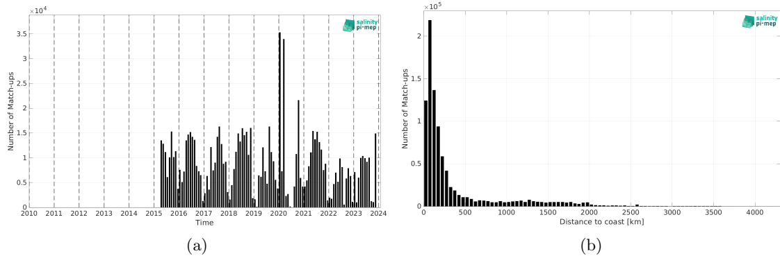
Figure 2: Number of match-ups between TSG (SAMOS) and SMAP SSS L2 v5.3 - 40 km (RSS) SSS as a function of time (a) and as function of the distance to coast (b) over the Mid-Low Latitudes 45N-45S Pi-MEP region and for the full satellite product period.
