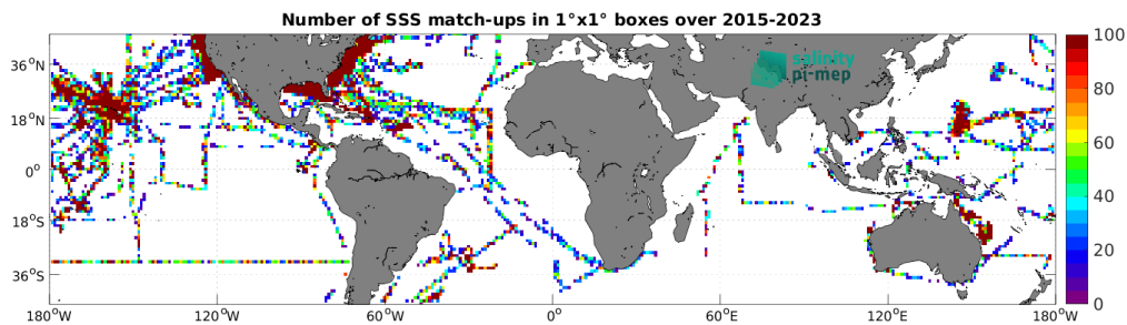
Figure 5: Number of SSS match-ups between TSG (SAMOS) SSS and the SMAP SSS L2 v5.3 - 40 km (RSS) SSS product for the Mid-Low Latitudes 45N-45S Pi-MEP region over 1^\circ \times 1^\circ boxes and for the full satellite product period.
