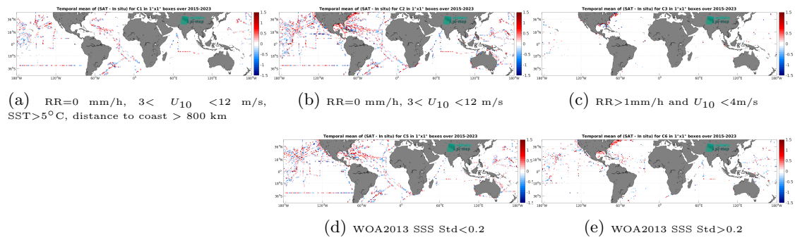
Figure 14: Temporal mean gridded over spatial boxes of size 1^\circ \times 1^\circ of \Delta SSS (SMAP SSS L2 v5.3 - 40 km (RSS) - TSG (SAMOS)) for 5 different subdatasets corresponding to: RR=0 mm/h, 3 < U_{10} < 12 m/s, SST > 5°C, distance to coast > 800 km (a), RR=0 mm/h, 3 < U_{10} < 12 m/s (b), RR > 1mm/h and U_{10} < 4 m/s (c), WOA2013 SSS Std < 0.2 (d), WOA2013 SSS Std > 0.2 (e).
