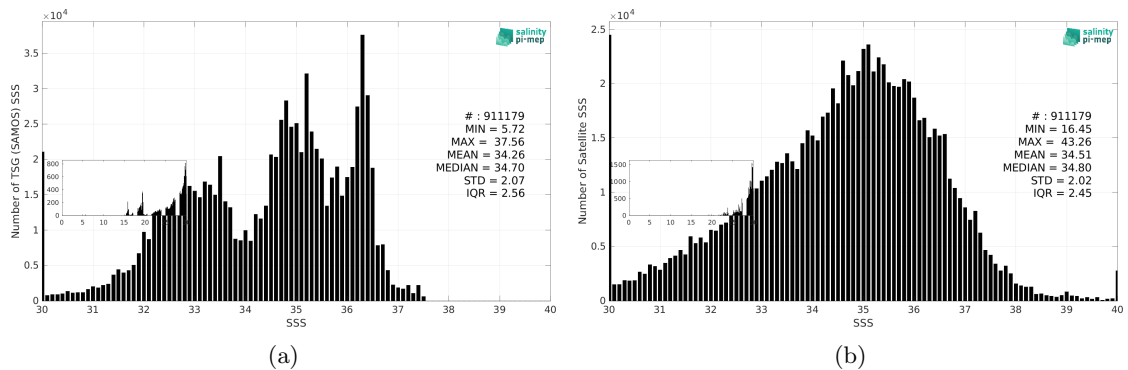
Figure 3: Histograms of SSS from TSG (SAMOS) (a) and SMAP SSS L2 v5.3 - 40 km (RSS) (b) considering all match-up pairs per bins of 0.1 over the Mid-Low Latitudes 45N-45S Pi-MEP region and for the full satellite product period.
