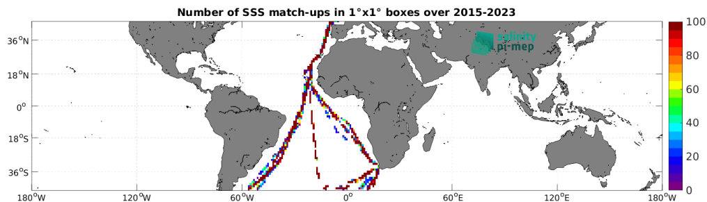
Figure 5: Number of SSS match-ups between TSG (Polarstern) SSS and the SMAP SSS L2 v5.3 - 40 km (RSS) SSS product for the Mid-Low Latitudes 45N-45S Pi-MEP region over 1^\circ \times 1^\circ boxes and for the full satellite product period.
