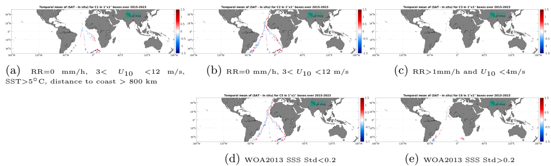
Figure 14: Temporal mean gridded over spatial boxes of size 1^\circ \times 1^\circ of \Delta\text{SSS} (SMAP SSS L2 v5.3 - 40 km (RSS) - TSG (Polarstern)) for 5 different subdatasets corresponding to:RR=0 mm/h, 3 < U_{10} < 12 m/s, SST>5°C, distance to coast > 800 km (a), RR=0 mm/h, 3 < U_{10} < 12 m/s (b), RR>1mm/h and U_{10} < 4 m/s (c), WOA2013 SSS Std<0.2 (d), WOA2013 SSS Std>0.2 (e).
