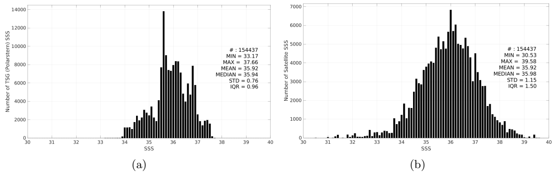
Figure 3: Histograms of SSS from TSG (Polarstern) (a) and SMAP SSS L2 v5.3 - 40 km (RSS) (b) considering all match-up pairs per bins of 0.1 over the Mid-Low Latitudes 45N-45S Pi-MEP region and for the full satellite product period.
