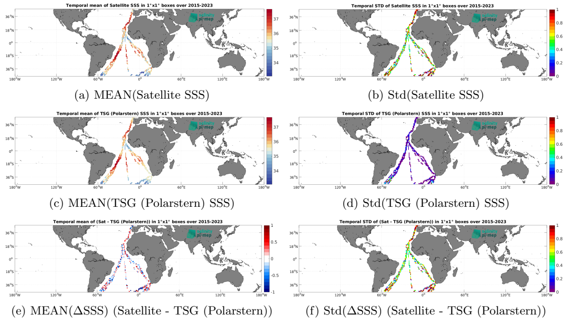
Figure 7: Temporal mean (left) and Std (right) of SSS from SMAP SSS L2 v5.3 - 40 km (RSS) (top), TSG (Polarstern) (middle), and of \Delta SSS (Satellite - TSG (Polarstern)). Only match-up pairs are used to generate these maps.
