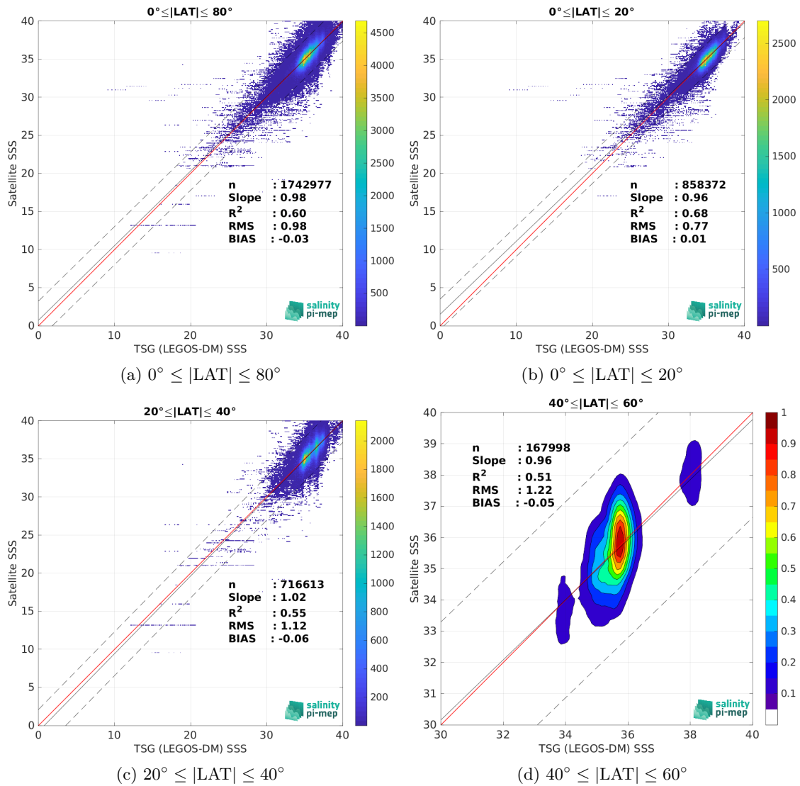
Figure 10: Contour maps of the concentration of SMAP SSS L2 v5.3 - 40 km (RSS) SSS (y-axis) versus TSG (LEGOS-DM) SSS (x-axis) at match-up pairs for different latitude bands. For each plot, the red line shows x=y . The black thin and dashed lines indicate a linear fit through the data cloud and the \pm 95\% confidence levels, respectively. The number match-up pairs n , the slope and R^2 coefficient of the linear fit, the root mean square (RMS) and the mean bias between satellite and in situ data are indicated for each latitude band in each plots.
