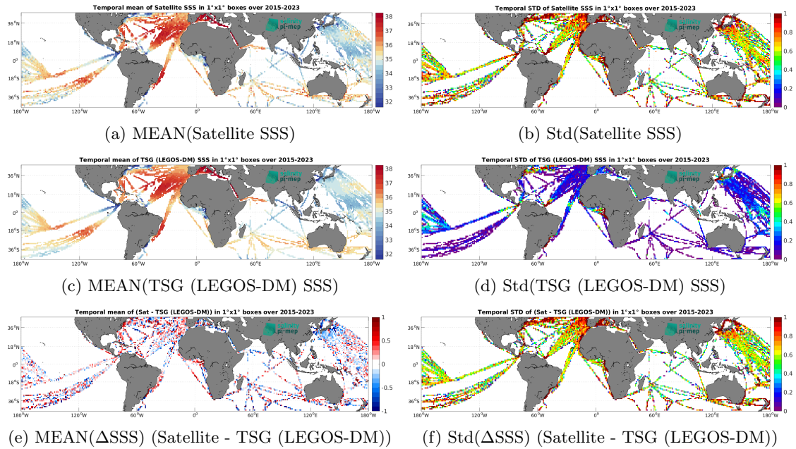
Figure 7: Temporal mean (left) and Std (right) of SSS from SMAP SSS L2 v5.3 - 40 km (RSS) (top), TSG (LEGOS-DM) (middle), and of \Delta SSS (Satellite - TSG (LEGOS-DM)). Only match-up pairs are used to generate these maps.
