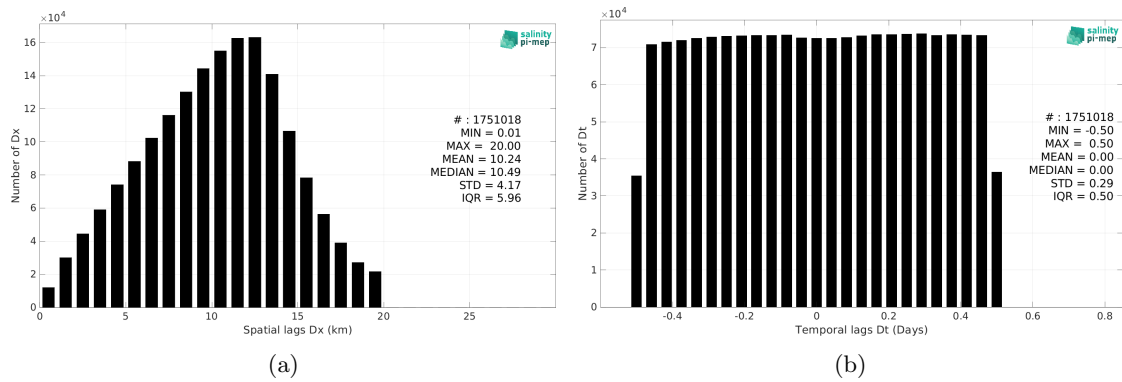
Figure 6: Histograms of the spatial (a) and temporal (b) lags between the location/time of the TSG (LEGOS-DM) measurement and the date of the corresponding SMAP SSS L2 v5.3 - 40 km (RSS) SSS pixel.
