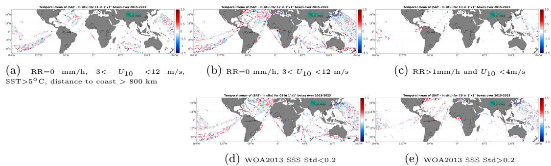
Figure 14: Temporal mean gridded over spatial boxes of size 1^\circ \times 1^\circ of \Delta SSS (SMAP SSS L2 v5.3 - 40 km (RSS) - TSG (LEGOS-DM)) for 5 different subdatasets corresponding to:RR=0 mm/h, 3 < U_{10} < 12 m/s, SST >5^\circ\text{C} , distance to coast > 800 km (a), RR=0 mm/h, 3 < U_{10} < 12 m/s (b), RR >1 mm/h and U_{10} < 4 m/s (c), WOA2013 SSS Std <0.2 (d), WOA2013 SSS Std >0.2 (e).
