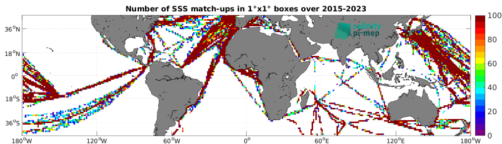
Figure 5: Number of SSS match-ups between TSG (LEGOS-DM) SSS and the SMAP SSS L2 v5.3 - 40 km (RSS) SSS product for the Mid-Low Latitudes 45N-45S Pi-MEP region over 1^\circ \times 1^\circ boxes and for the full satellite product period.
