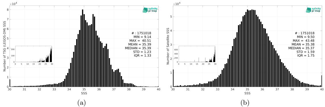
Figure 3: Histograms of SSS from TSG (LEGOS-DM) (a) and SMAP SSS L2 v5.3 - 40 km (RSS) (b) considering all match-up pairs per bins of 0.1 over the Mid-Low Latitudes 45N-45S Pi-MEP region and for the full satellite product period.
