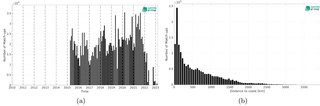
Figure 2: Number of match-ups between TSG (LEGOS-DM) and SMAP SSS L2 v5.3 - 40 km (RSS) SSS as a function of time (a) and as function of the distance to coast (b) over the Mid-Low Latitudes 45N-45S Pi-MEP region and for the full satellite product period.
