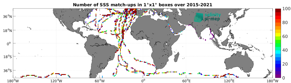
Figure 5: Number of SSS match-ups between TSG (GOSUD-Sailing-ship) SSS and the SMAP SSS L2 v5.3 - 40 km (RSS) SSS product for the Mid-Low Latitudes 45N-45S Pi-MEP region over 1^\circ \times 1^\circ boxes and for the full satellite product period.
