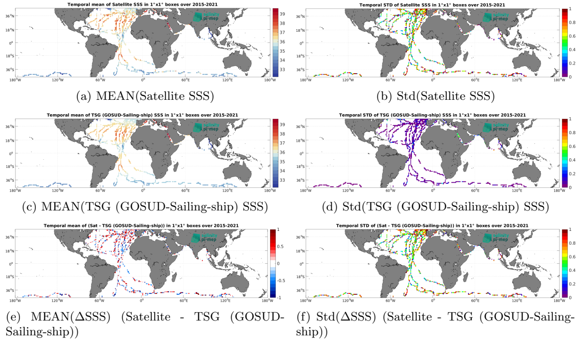
Figure 7: Temporal mean (left) and Std (right) of SSS from SMAP SSS L2 v5.3 - 40 km (RSS) (top), TSG (GOSUD-Sailing-ship) (middle), and of \Delta SSS (Satellite - TSG (GOSUD-Sailing-ship)). Only match-up pairs are used to generate these maps.
