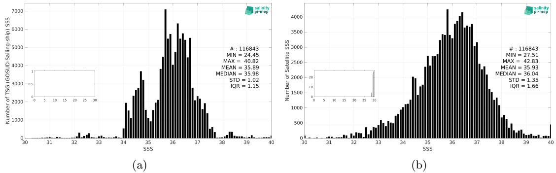
Figure 3: Histograms of SSS from TSG (GOSUD-Sailing-ship) (a) and SMAP SSS L2 v5.3 - 40 km (RSS) (b) considering all match-up pairs per bins of 0.1 over the Mid-Low Latitudes 45N-45S Pi-MEP region and for the full satellite product period.
