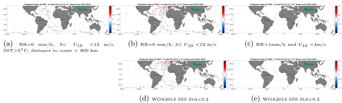
Figure 14: Temporal mean gridded over spatial boxes of size 1^\circ \times 1^\circ of \Delta\text{SSS} (SMAP SSS L2 v5.3 - 40 km (RSS) - TSG (GOSUD-Sailing-ship)) for 5 different subdatasets corresponding to: RR=0 mm/h, 3 < U_{10} < 12 m/s, SST > 5°C, distance to coast > 800 km (a), RR=0 mm/h, 3 < U_{10} < 12 m/s (b), RR > 1mm/h and U_{10} < 4 m/s (c), WOA2013 SSS Std < 0.2 (d), WOA2013 SSS Std > 0.2 (e).
