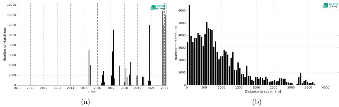
Figure 2: Number of match-ups between TSG (GOSUD-Sailing-ship) and SMAP SSS L2 v5.3 - 40 km (RSS) SSS as a function of time (a) and as function of the distance to coast (b) over the Mid-Low Latitudes 45N-45S Pi-MEP region and for the full satellite product period.
