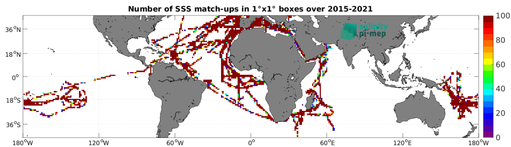
Figure 5: Number of SSS match-ups between TSG (GOSUD-Research-vessel) SSS and the SMAP SSS L2 v5.3 - 40 km (RSS) SSS product for the Mid-Low Latitudes 45N-45S Pi-MEP region over 1^\circ \times 1^\circ boxes and for the full satellite product period.
