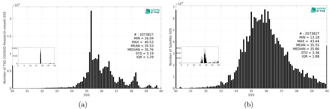
Figure 3: Histograms of SSS from TSG (GOSUD-Research-vessel) (a) and SMAP SSS L2 v5.3 - 40 km (RSS) (b) considering all match-up pairs per bins of 0.1 over the Mid-Low Latitudes 45N-45S Pi-MEP region and for the full satellite product period.
