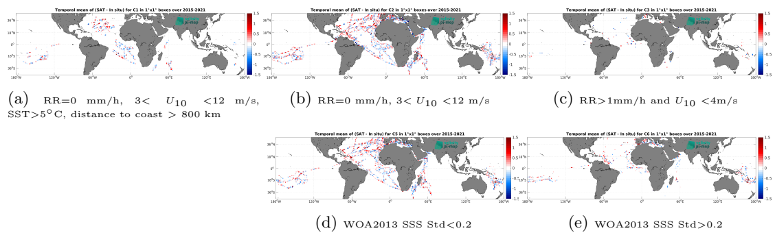
Figure 14: Temporal mean gridded over spatial boxes of size 1^\circ \times 1^\circ of \Delta\text{SSS} (SMAP SSS L2 v5.3 - 40 km (RSS) - TSG (GOSUD-Research-vessel)) for 5 different subdatasets corresponding to:RR=0 mm/h, 3 < U_{10} < 12 m/s, SST >5^\circ\text{C} , distance to coast > 800 km (a), RR=0 mm/h, 3 < U_{10} < 12 m/s (b), RR >1 mm/h and U_{10} < 4 m/s (c), WOA2013 SSS Std <0.2 (d), WOA2013 SSS Std >0.2 (e).
