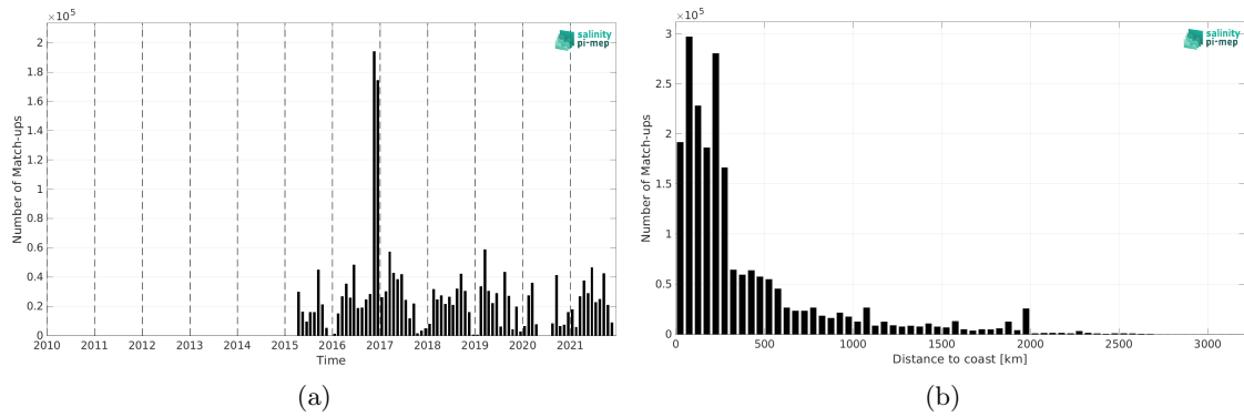
Figure 2: Number of match-ups between TSG (GOSUD-Research-vessel) and SMAP SSS L2 v5.3 - 40 km (RSS) SSS as a function of time (a) and as function of the distance to coast (b) over the Mid-Low Latitudes 45N-45S Pi-MEP region and for the full satellite product period.
