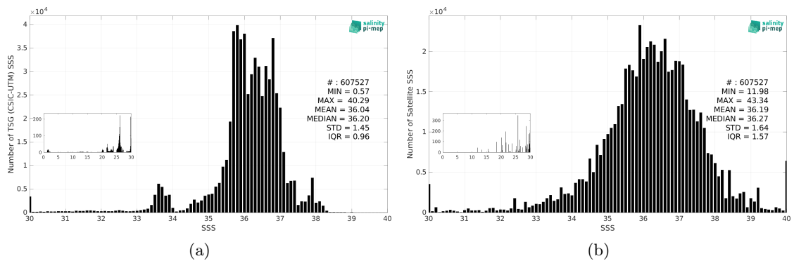
Figure 3: Histograms of SSS from TSG (CSIC-UTM) (a) and SMAP SSS L2 v5.3 - 40 km (RSS) (b) considering all match-up pairs per bins of 0.1 over the Mid-Low Latitudes 45N-45S Pi-MEP region and for the full satellite product period.
