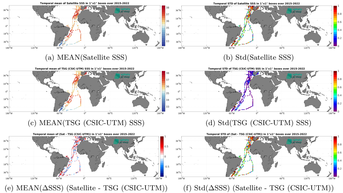
Figure 7: Temporal mean (left) and Std (right) of SSS from SMAP SSS L2 v5.3 - 40 km (RSS) (top), TSG (CSIC-UTM) (middle), and of \Delta SSS (Satellite - TSG (CSIC-UTM)). Only match-up pairs are used to generate these maps.
