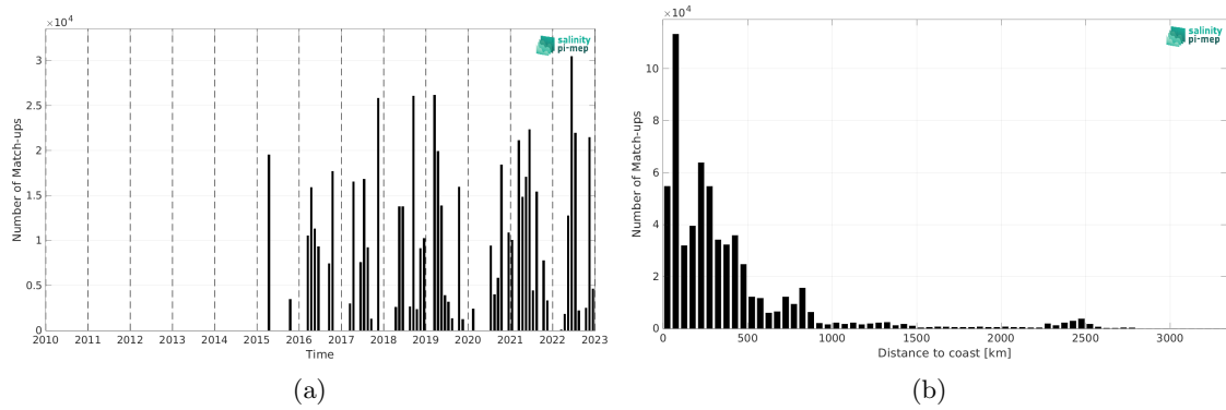
Figure 2: Number of match-ups between TSG (CSIC-UTM) and SMAP SSS L2 v5.3 - 40 km (RSS) SSS as a function of time (a) and as function of the distance to coast (b) over the Mid-Low Latitudes 45N-45S Pi-MEP region and for the full satellite product period.
