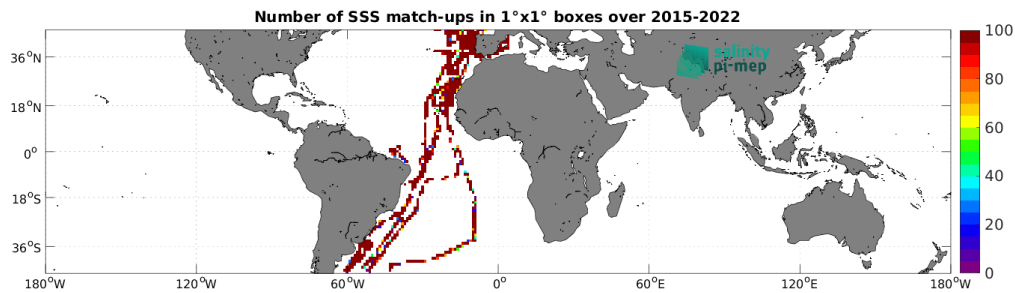
Figure 5: Number of SSS match-ups between TSG (CSIC-UTM) SSS and the SMAP SSS L2 v5.3 - 40 km (RSS) SSS product for the Mid-Low Latitudes 45N-45S Pi-MEP region over 1^\circ \times 1^\circ boxes and for the full satellite product period.
