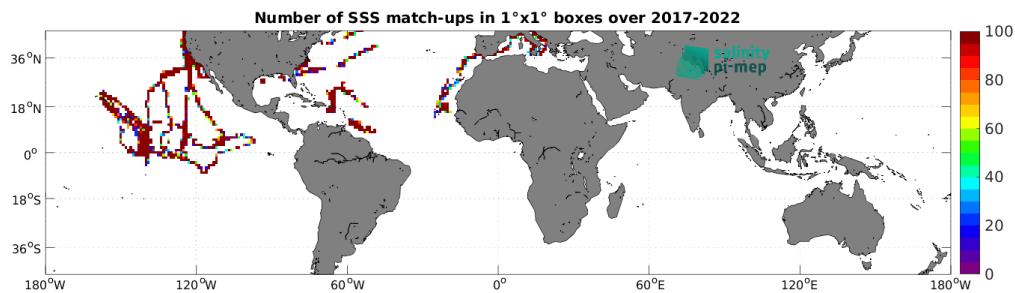
Figure 5: Number of SSS match-ups between Saildrone SSS and the SMAP SSS L2 v5.3 - 40 km (RSS) SSS product for the Mid-Low Latitudes 45N-45S Pi-MEP region over 1^\circ \times 1^\circ boxes and for the full satellite product period.
