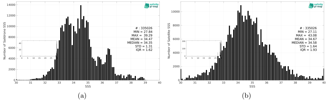
Figure 3: Histograms of SSS from Saildrone (a) and SMAP SSS L2 v5.3 - 40 km (RSS) (b) considering all match-up pairs per bins of 0.1 over the Mid-Low Latitudes 45N-45S Pi-MEP region and for the full satellite product period.
