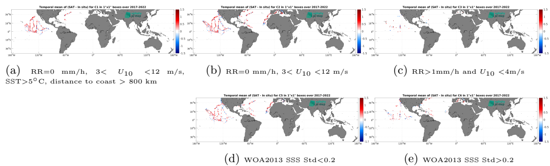
Figure 14: Temporal mean gridded over spatial boxes of size 1^\circ \times 1^\circ of \Delta\text{SSS} (SMAP SSS L2 v5.3 - 40 km (RSS) - Sairdrone) for 5 different subdatasets corresponding to: RR=0 mm/h, 3 < U_{10} < 12 m/s, SST > 5°C, distance to coast > 800 km (a), RR=0 mm/h, 3 < U_{10} < 12 m/s (b), RR > 1mm/h and U_{10} < 4 m/s (c), WOA2013 SSS Std < 0.2 (d), WOA2013 SSS Std > 0.2 (e).
