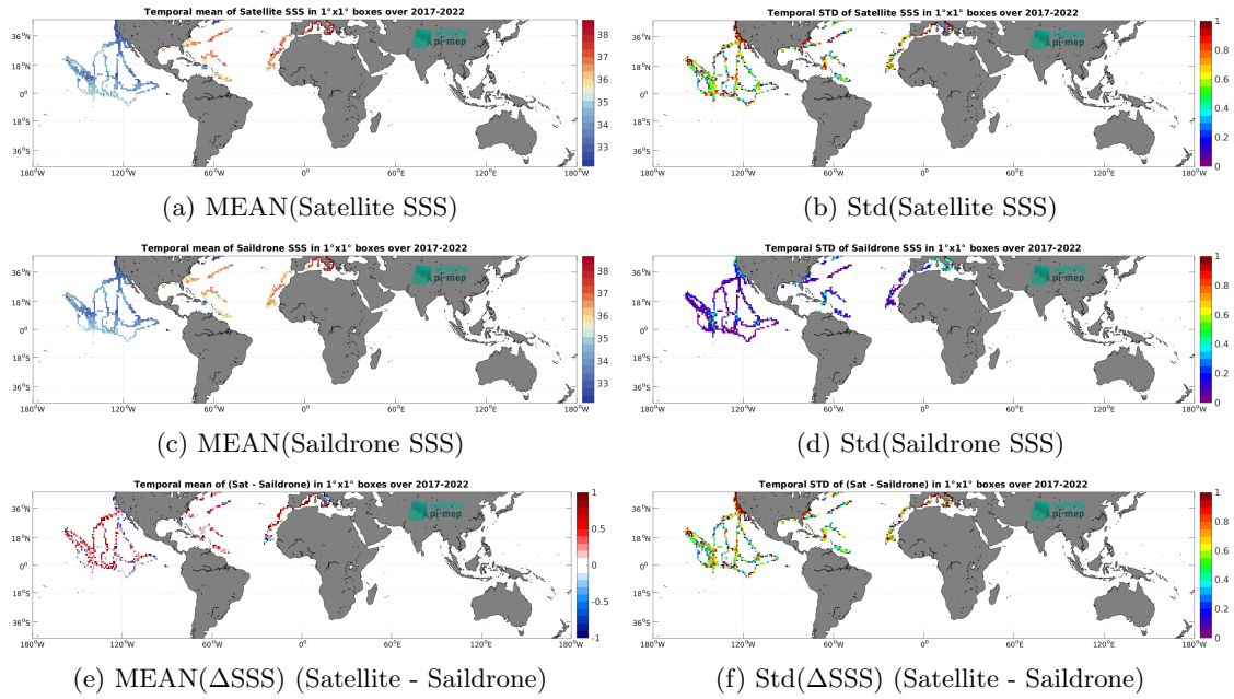
Figure 7: Temporal mean (left) and Std (right) of SSS from SMAP SSS L2 v5.3 - 40 km (RSS) (top), Saildrone (middle), and of \Delta SSS (Satellite - Saildrone). Only match-up pairs are used to generate these maps.
