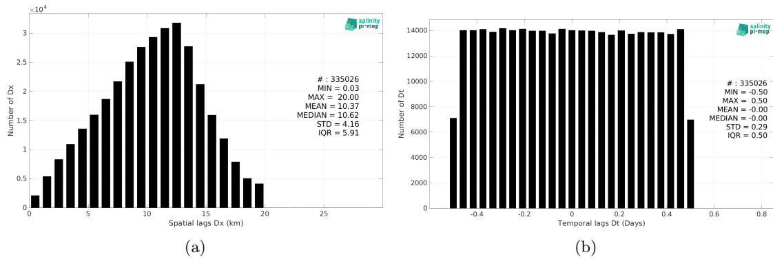
Figure 6: Histograms of the spatial (a) and temporal (b) lags between the location/time of the Saildrone measurement and the date of the corresponding SMAP SSS L2 v5.3 - 40 km (RSS) SSS pixel.
