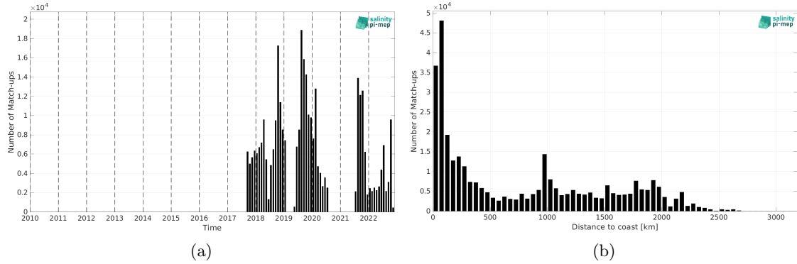
Figure 2: Number of match-ups between Saildrone and SMAP SSS L2 v5.3 - 40 km (RSS) SSS as a function of time (a) and as function of the distance to coast (b) over the Mid-Low Latitudes 45N-45S Pi-MEP region and for the full satellite product period.
