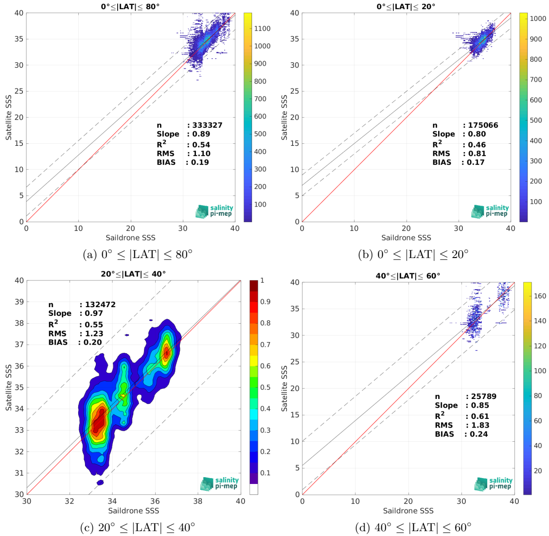
Figure 10: Contour maps of the concentration of SMAP SSS L2 v5.3 - 40 km (RSS) SSS (y-axis) versus Sairdrone SSS (x-axis) at match-up pairs for different latitude bands. For each plot, the red line shows x=y . The black thin and dashed lines indicate a linear fit through the data cloud and the \pm 95\% confidence levels, respectively. The number match-up pairs n , the slope and R^2 coefficient of the linear fit, the root mean square (RMS) and the mean bias between satellite and in situ data are indicated for each latitude band in each plots.
