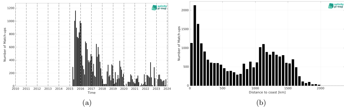
Figure 2: Number of match-ups between Marine mammals and SMAP SSS L2 v5.3 - 40 km (RSS) SSS as a function of time (a) and as function of the distance to coast (b) over the Mid-Low Latitudes 45N-45S Pi-MEP region and for the full satellite product period.
