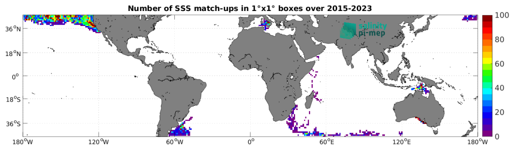
Figure 5: Number of SSS match-ups between Marine mammals SSS and the SMAP SSS L2 v5.3 - 40 km (RSS) SSS product for the Mid-Low Latitudes 45N-45S Pi-MEP region over 1^\circ \times 1^\circ boxes and for the full satellite product period.
