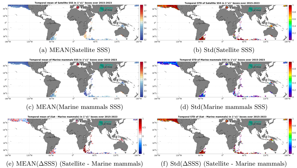
Figure 7: Temporal mean (left) and Std (right) of SSS from SMAP SSS L2 v5.3 - 40 km (RSS) (top), Marine mammals (middle), and of \Delta SSS (Satellite - Marine mammals). Only match-up pairs are used to generate these maps.
