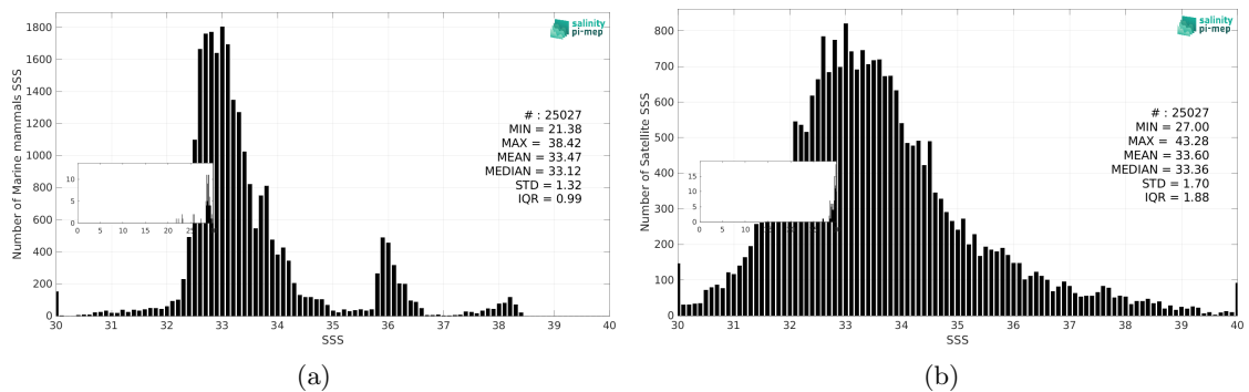
Figure 3: Histograms of SSS from Marine mammals (a) and SMAP SSS L2 v5.3 - 40 km (RSS) (b) considering all match-up pairs per bins of 0.1 over the Mid-Low Latitudes 45N-45S Pi-MEP region and for the full satellite product period.
