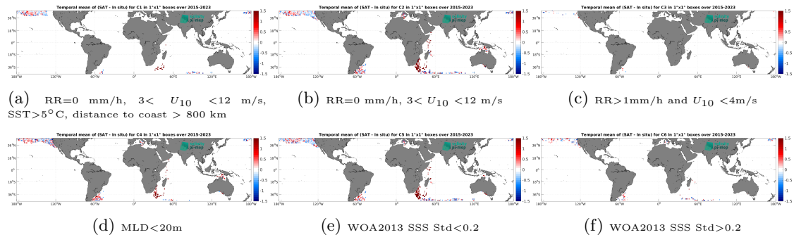
Figure 14: Temporal mean gridded over spatial boxes of size 1^\circ \times 1^\circ of \Delta SSS (SMAP SSS L2 v5.3 - 40 km (RSS) - Marine mammals) for 6 different subdatasets corresponding to:RR=0 mm/h, 3 < U_{10} < 12 m/s, SST > 5°C, distance to coast > 800 km (a), RR=0 mm/h, 3 < U_{10} < 12 m/s (b), RR > 1mm/h and U_{10} < 4 m/s (c),MLD < 20m (d),WOA2013 SSS Std < 0.2 (e),WOA2013 SSS Std > 0.2 (f).
