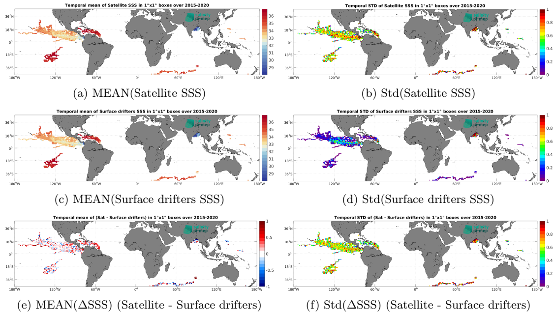
Figure 6: Temporal mean (left) and Std (right) of SSS from SMAP SSS L2 v5.3 - 40 km (RSS) (top), Surface drifters (middle), and of \Delta SSS (Satellite - Surface drifters). Only match-up pairs are used to generate these maps.
