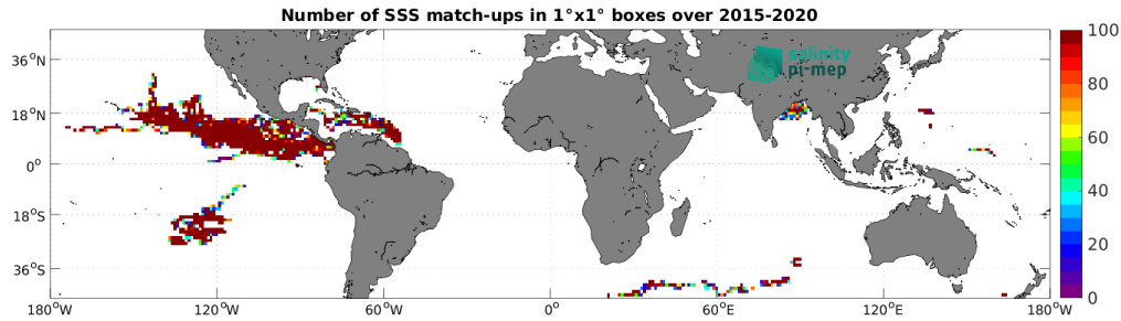
Figure 4: Number of SSS match-ups between Surface drifters SSS and the SMAP SSS L2 v5.3 - 40 km (RSS) SSS product for the Mid-Low Latitudes 45N-45S Pi-MEP region over 1^\circ \times 1^\circ boxes and for the full satellite product period.
