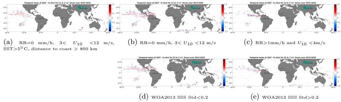
Figure 13: Temporal mean gridded over spatial boxes of size 1^\circ \times 1^\circ of \Delta SSS (SMAP SSS L2 v5.3 - 40 km (RSS) - Surface drifters) for 5 different subdatasets corresponding to:RR=0 mm/h, 3 < U_{10} < 12 m/s, SST >5^\circ\text{C} , distance to coast > 800 km (a), RR=0 mm/h, 3 < U_{10} < 12 m/s (b), RR >1 mm/h and U_{10} < 4 m/s (c), WOA2013 SSS Std <0.2 (d), WOA2013 SSS Std >0.2 (e).
