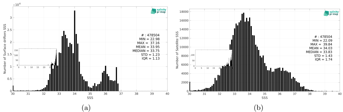
Figure 3: Histograms of SSS from Surface drifters (a) and SMAP SSS L2 v5.3 - 40 km (RSS) (b) considering all match-up pairs per bins of 0.1 over the Mid-Low Latitudes 45N-45S Pi-MEP region and for the full satellite product period.
