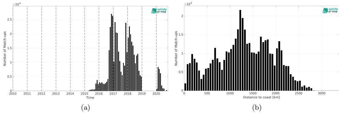
Figure 2: Number of match-ups between Surface drifters and SMAP SSS L2 v5.3 - 40 km (RSS) SSS as a function of time (a) and as function of the distance to coast (b) over the Mid-Low Latitudes 45N-45S Pi-MEP region and for the full satellite product period.
