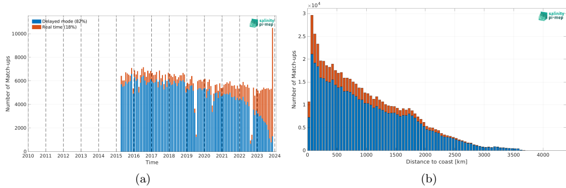
Figure 2: Number of match-ups between Argo and SMAP SSS L2 v5.3 - 40 km (RSS) SSS as a function of time (a) and as function of the distance to coast (b) over the Mid-Low Latitudes 45N-45S Pi-MEP region and for the full satellite product period.
