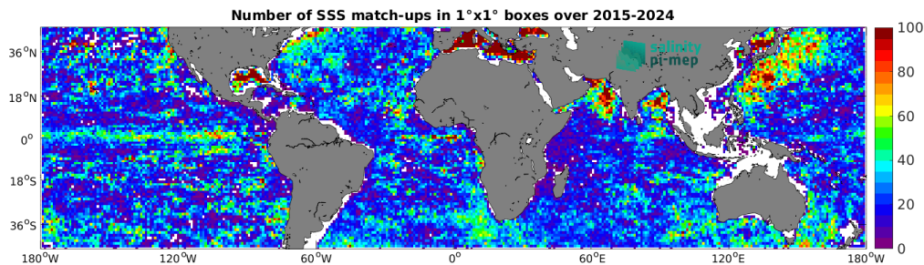
Figure 5: Number of SSS match-ups between Argo SSS and the SMAP SSS L2 v5.3 - 40 km (RSS) SSS product for the Mid-Low Latitudes 45N-45S Pi-MEP region over 1^\circ \times 1^\circ boxes and for the full satellite product period.
