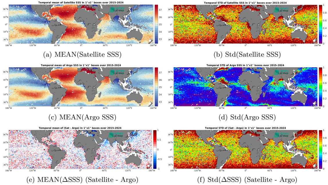
Figure 7: Temporal mean (left) and Std (right) of SSS from SMAP SSS L2 v5.3 - 40 km (RSS) (top), Argo (middle), and of \Delta SSS (Satellite - Argo). Only match-up pairs are used to generate these maps.
