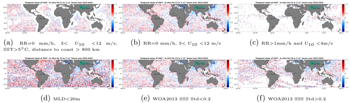
Figure 14: Temporal mean gridded over spatial boxes of size 1^\circ \times 1^\circ of \Delta SSS (SMAP SSS L2 v5.3 - 40 km (RSS) - Argo) for 6 different subdatasets corresponding to:RR=0 mm/h, 3 < U_{10} < 12 m/s, SST>5°C, distance to coast > 800 km (a), RR=0 mm/h, 3 < U_{10} < 12 m/s (b), RR>1mm/h and U_{10} < 4 m/s (c),MLD<20m (d),WOA2013 SSS Std<0.2 (e),WOA2013 SSS Std>0.2 (f).
