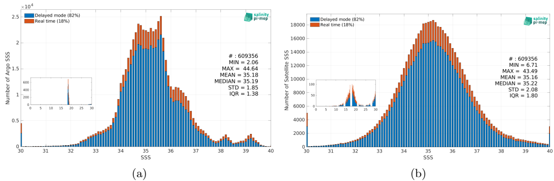
Figure 3: Histograms of SSS from Argo (a) and SMAP SSS L2 v5.3 - 40 km (RSS) (b) considering all match-up pairs per bins of 0.1 over the Mid-Low Latitudes 45N-45S Pi-MEP region and for the full satellite product period.
