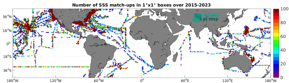
Figure 4: Number of SSS match-ups between TSG (SAMOS) SSS and the SMAP SSS L2 v5 - 40 km (RSS) SSS product for the Mid-Low Latitudes 45N-45S Pi-MEP region over 1^\circ \times 1^\circ boxes and for the full satellite product period.
