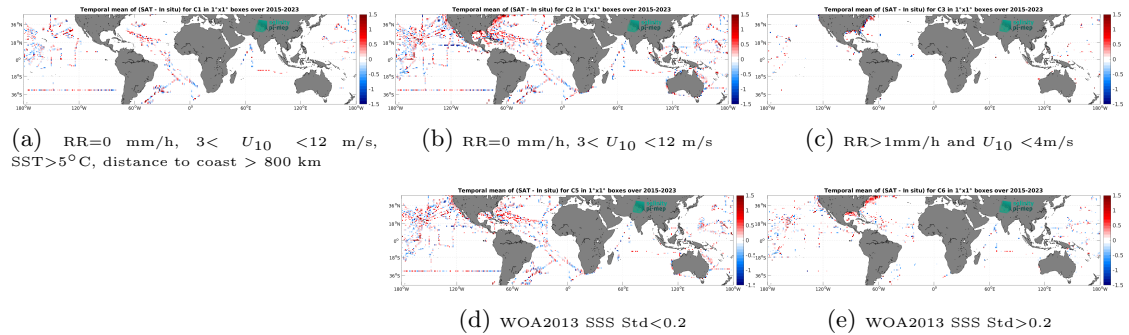
Figure 12: Temporal mean gridded over spatial boxes of size 1^\circ \times 1^\circ of \Delta SSS (SMAP SSS L2 v5 - 40 km (RSS) - TSG (SAMOS)) for 5 different subdatasets corresponding to:RR=0 mm/h, 3 < U_{10} < 12 m/s, SST>5°C, distance to coast > 800 km (a), RR=0 mm/h, 3 < U_{10} < 12 m/s (b), RR>1mm/h and U_{10} < 4 m/s (c), WOA2013 SSS Std<0.2 (d), WOA2013 SSS Std>0.2 (e).
