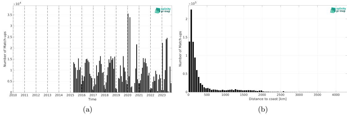
Figure 1: Number of match-ups between TSG (SAMOS) and SMAP SSS L2 v5 - 40 km (RSS) SSS as a function of time (a) and as function of the distance to coast (b) over the Mid-Low Latitudes 45N-45S Pi-MEP region and for the full satellite product period.
