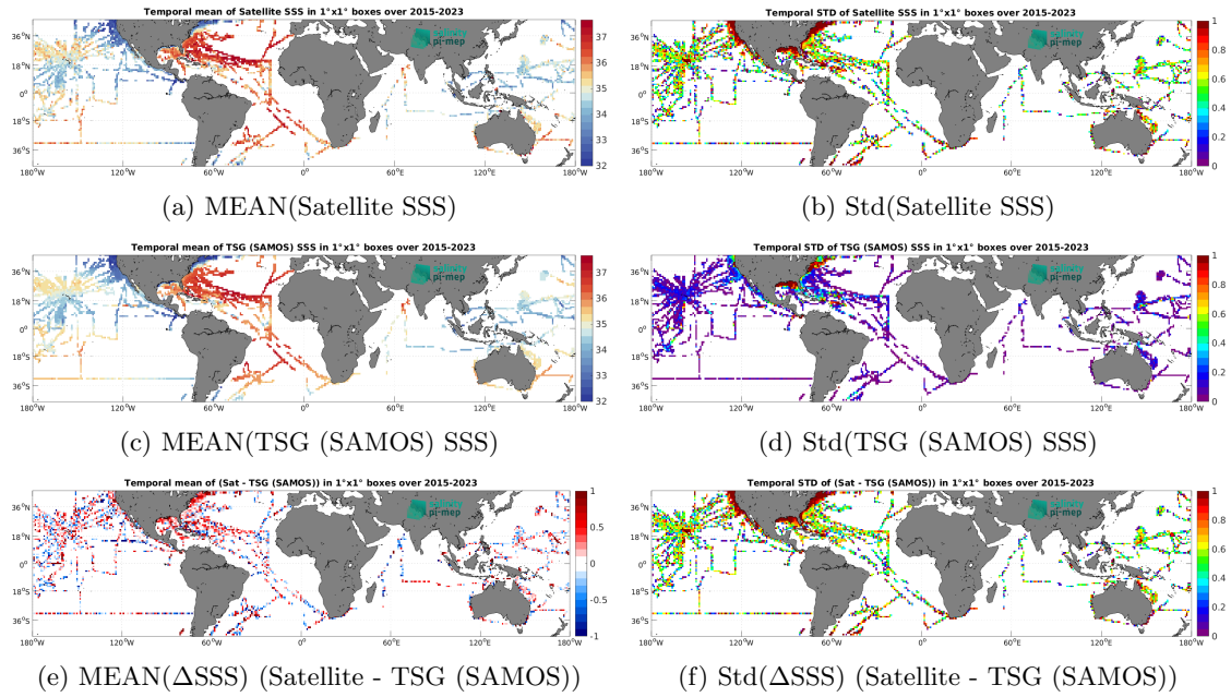
Figure 6: Temporal mean (left) and Std (right) of SSS from SMAP SSS L2 v5 - 40 km (RSS) (top), TSG (SAMOS) (middle), and of \Delta SSS (Satellite - TSG (SAMOS)). Only match-up pairs are used to generate these maps.
