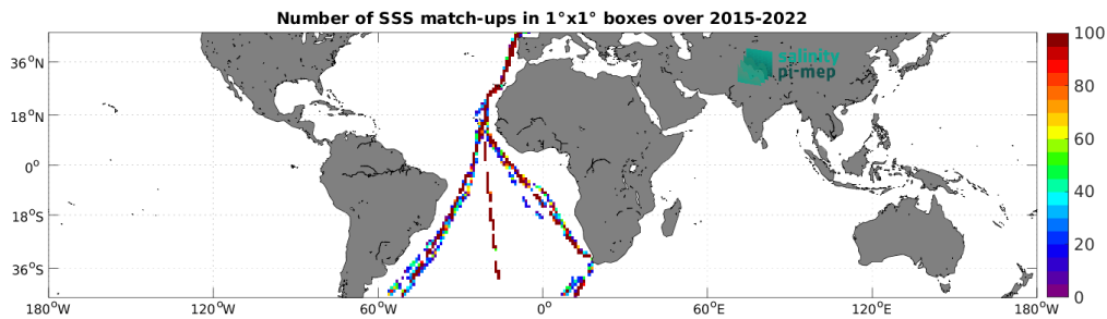
Figure 4: Number of SSS match-ups between TSG (Polarstern) SSS and the SMAP SSS L2 v5 - 40 km (RSS) SSS product for the Mid-Low Latitudes 45N-45S Pi-MEP region over 1^\circ \times 1^\circ boxes and for the full satellite product period.
