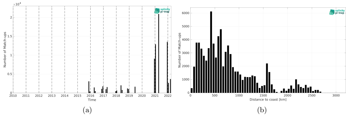
Figure 1: Number of match-ups between TSG (Polarstern) and SMAP SSS L2 v5 - 40 km (RSS) SSS as a function of time (a) and as function of the distance to coast (b) over the Mid-Low Latitudes 45N-45S Pi-MEP region and for the full satellite product period.
