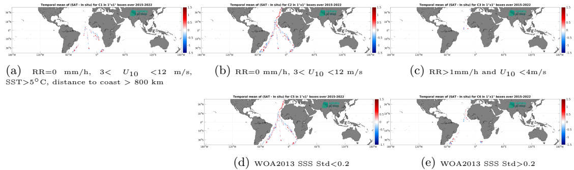
Figure 12: Temporal mean gridded over spatial boxes of size 1^\circ \times 1^\circ of \Delta SSS (SMAP SSS L2 v5 - 40 km (RSS) - TSG (Polarstern)) for 5 different subdatasets corresponding to:RR=0 mm/h, 3 < U_{10} < 12 m/s, SST >5^\circ\text{C} , distance to coast > 800 km (a), RR=0 mm/h, 3 < U_{10} < 12 m/s (b), RR >1 mm/h and U_{10} < 4 m/s (c), WOA2013 SSS Std <0.2 (d), WOA2013 SSS Std >0.2 (e).
