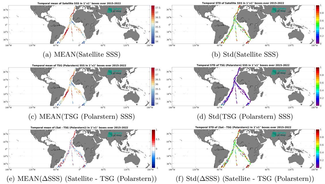
Figure 6: Temporal mean (left) and Std (right) of SSS from SMAP SSS L2 v5 - 40 km (RSS) (top), TSG (Polarstern) (middle), and of \Delta SSS (Satellite - TSG (Polarstern)). Only match-up pairs are used to generate these maps.
