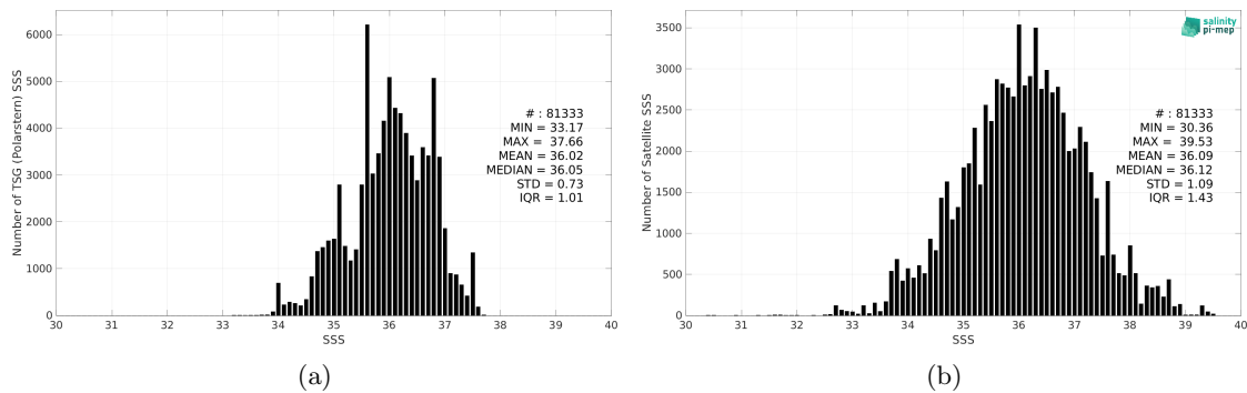
Figure 2: Histograms of SSS from TSG (Polarstern) (a) and SMAP SSS L2 v5 - 40 km (RSS) (b) considering all match-up pairs per bins of 0.1 over the Mid-Low Latitudes 45N-45S Pi-MEP region and for the full satellite product period.
