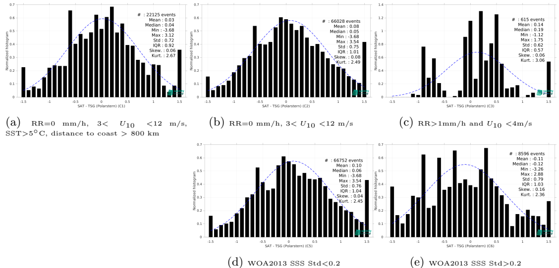
Figure 13: Normalized histogram of \Delta SSS (SMAP SSS L2 v5 - 40 km (RSS) - TSG (Polarstern)) for 5 different subdatasets corresponding to: RR=0 mm/h, 3 < U_{10} < 12 m/s, SST >5^\circ\text{C} , distance to coast > 800 km (a), RR=0 mm/h, 3 < U_{10} < 12 m/s (b), RR >1 mm/h and U_{10} < 4 m/s (c), WOA2013 SSS Std <0.2 (d), WOA2013 SSS Std >0.2 (e).
