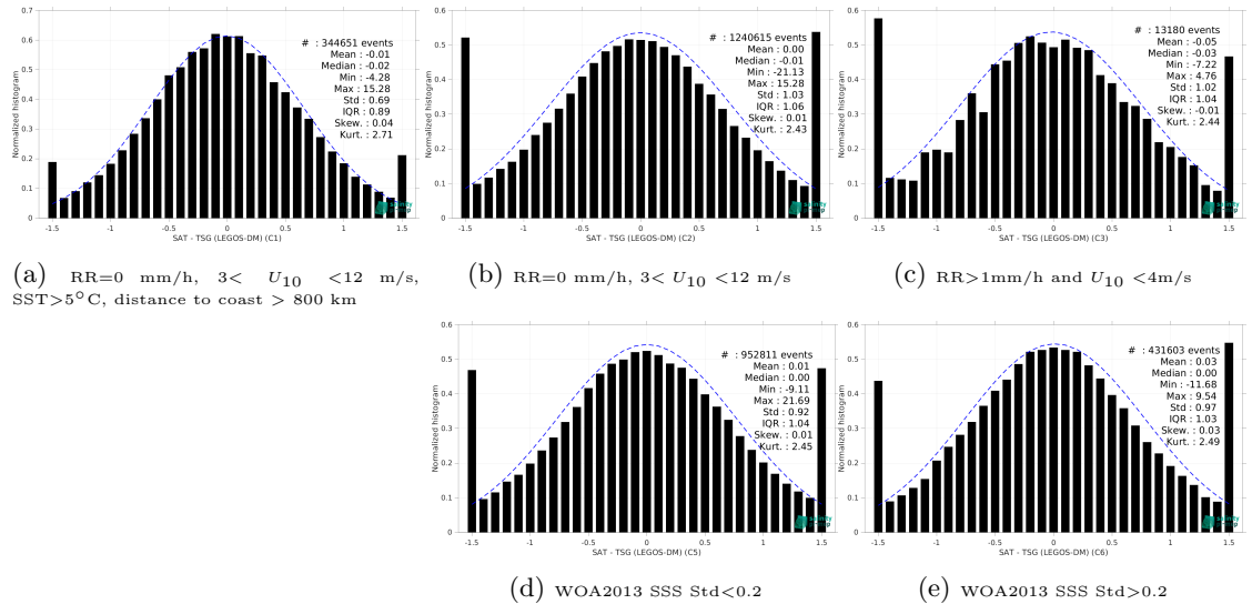
Figure 13: Normalized histogram of \Delta\text{SSS} (SMAP SSS L2 v5 - 40 km (RSS) - TSG (LEGOS-DM)) for 5 different subdatasets corresponding to: RR=0 mm/h, 3 < U_{10} < 12 m/s, SST >5^\circ\text{C} , distance to coast > 800 km (a), RR=0 mm/h, 3 < U_{10} < 12 m/s (b), RR >1 mm/h and U_{10} < 4 m/s (c), WOA2013 SSS Std <0.2 (d), WOA2013 SSS Std >0.2 (e).
