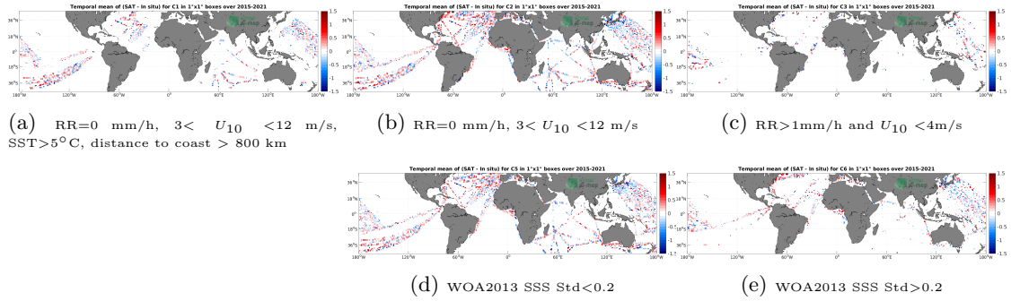
Figure 12: Temporal mean gridded over spatial boxes of size 1^\circ \times 1^\circ of \Delta SSS (SMAP SSS L2 v5 - 40 km (RSS) - TSG (LEGOS-DM)) for 5 different subdatasets corresponding to:RR=0 mm/h, 3 < U_{10} < 12 m/s, SST >5^\circ\text{C} , distance to coast > 800 km (a), RR=0 mm/h, 3 < U_{10} < 12 m/s (b), RR >1 mm/h and U_{10} < 4 m/s (c), WOA2013 SSS Std <0.2 (d), WOA2013 SSS Std >0.2 (e).
