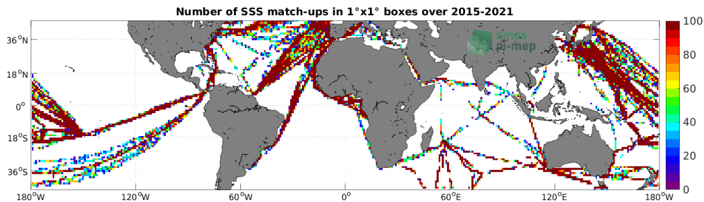
Figure 4: Number of SSS match-ups between TSG (LEGOS-DM) SSS and the SMAP SSS L2 v5 - 40 km (RSS) SSS product for the Mid-Low Latitudes 45N-45S Pi-MEP region over 1^\circ \times 1^\circ boxes and for the full satellite product period.
