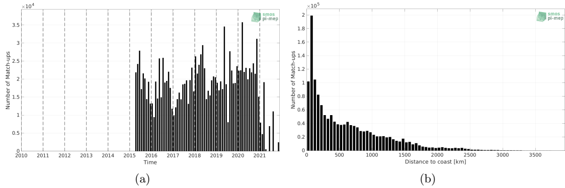
Figure 1: Number of match-ups between TSG (LEGOS-DM) and SMAP SSS L2 v5 - 40 km (RSS) SSS as a function of time (a) and as function of the distance to coast (b) over the Mid-Low Latitudes 45N-45S Pi-MEP region and for the full satellite product period.
