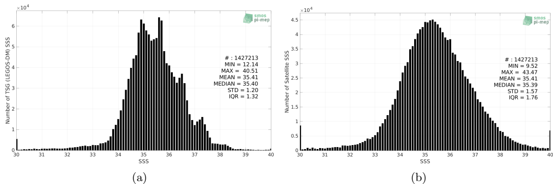
Figure 2: Histograms of SSS from TSG (LEGOS-DM) (a) and SMAP SSS L2 v5 - 40 km (RSS) (b) considering all match-up pairs per bins of 0.1 over the Mid-Low Latitudes 45N-45S Pi-MEP region and for the full satellite product period.
