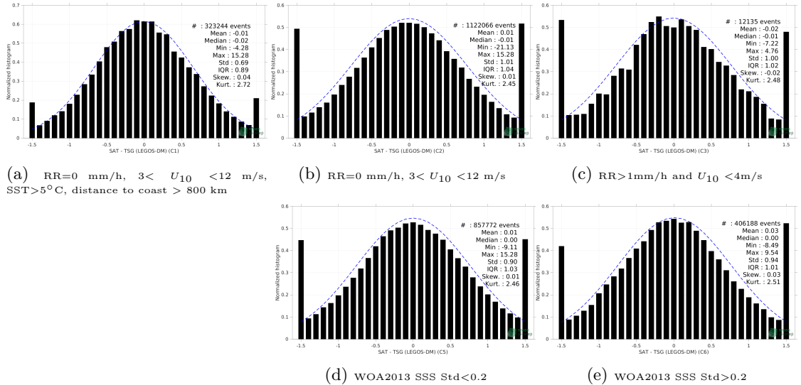
Figure 13: Normalized histogram of \Delta SSS (SMAP SSS L2 v5 - 40 km (RSS) - TSG (LEGOS-DM)) for 5 different subdatasets corresponding to: RR=0 mm/h, 3 < U_{10} < 12 m/s, SST >5^\circ\text{C} , distance to coast > 800 km (a), RR=0 mm/h, 3 < U_{10} < 12 m/s (b), RR >1 mm/h and U_{10} < 4 m/s (c), WOA2013 SSS Std <0.2 (d), WOA2013 SSS Std >0.2 (e).
