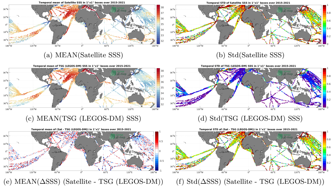
Figure 6: Temporal mean (left) and Std (right) of SSS from SMAP SSS L2 v5 - 40 km (RSS) (top), TSG (LEGOS-DM) (middle), and of \Delta SSS (Satellite - TSG (LEGOS-DM)). Only match-up pairs are used to generate these maps.
