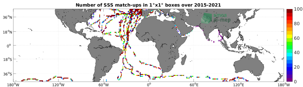
Figure 4: Number of SSS match-ups between TSG (GOSUD-Sailing-ship) SSS and the SMAP SSS L2 v5 - 40 km (RSS) SSS product for the Mid-Low Latitudes 45N-45S Pi-MEP region over 1^\circ \times 1^\circ boxes and for the full satellite product period.
