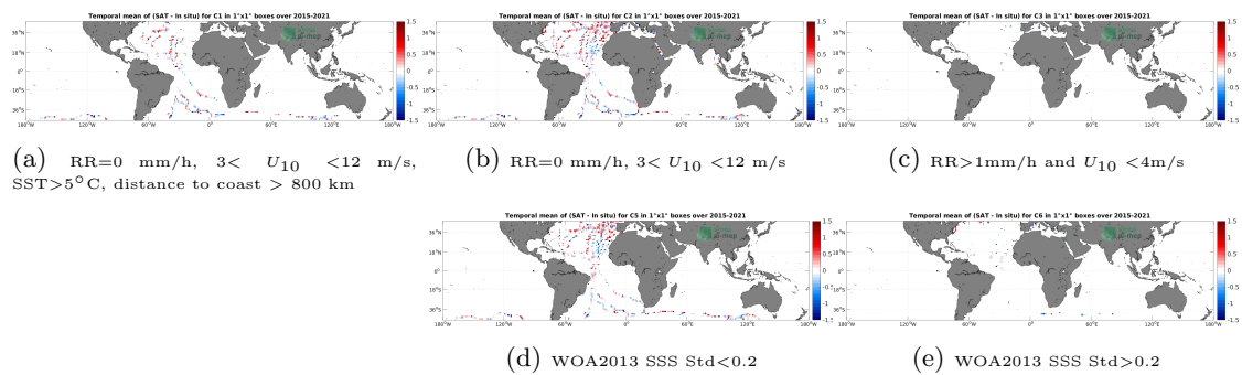
Figure 12: Temporal mean gridded over spatial boxes of size 1^\circ \times 1^\circ of \Delta\text{SSS} (SMAP SSS L2 v5 - 40 km (RSS) - TSG (GOSUD-Sailing-ship)) for 5 different subdatasets corresponding to: RR=0 mm/h, 3 < U_{10} < 12 m/s, SST > 5°C, distance to coast > 800 km (a), RR=0 mm/h, 3 < U_{10} < 12 m/s (b), RR > 1mm/h and U_{10} < 4 m/s (c), WOA2013 SSS Std < 0.2 (d), WOA2013 SSS Std > 0.2 (e).
