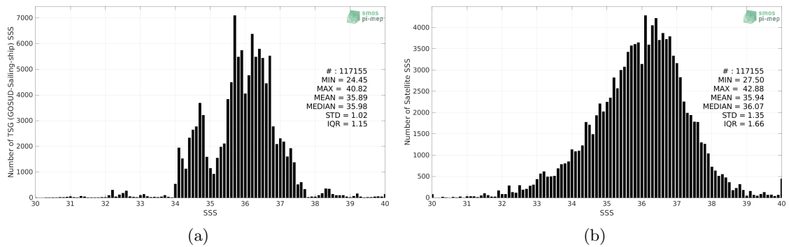
Figure 2: Histograms of SSS from TSG (GOSUD-Sailing-ship) (a) and SMAP SSS L2 v5 - 40 km (RSS) (b) considering all match-up pairs per bins of 0.1 over the Mid-Low Latitudes 45N-45S Pi-MEP region and for the full satellite product period.
