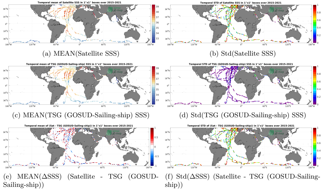
Figure 6: Temporal mean (left) and Std (right) of SSS from SMAP SSS L2 v5 - 40 km (RSS) (top), TSG (GOSUD-Sailing-ship) (middle), and of \Delta SSS (Satellite - TSG (GOSUD-Sailing-ship)). Only match-up pairs are used to generate these maps.
