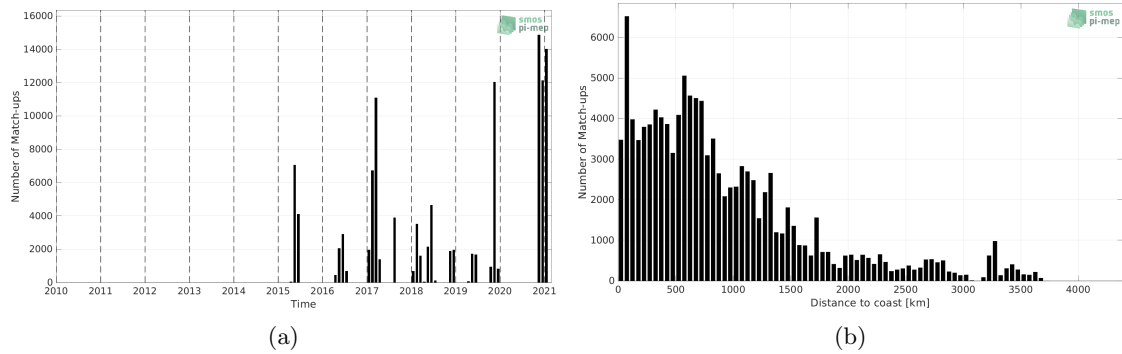
Figure 1: Number of match-ups between TSG (GOSUD-Sailing-ship) and SMAP SSS L2 v5 - 40 km (RSS) SSS as a function of time (a) and as function of the distance to coast (b) over the Mid-Low Latitudes 45N-45S Pi-MEP region and for the full satellite product period.
