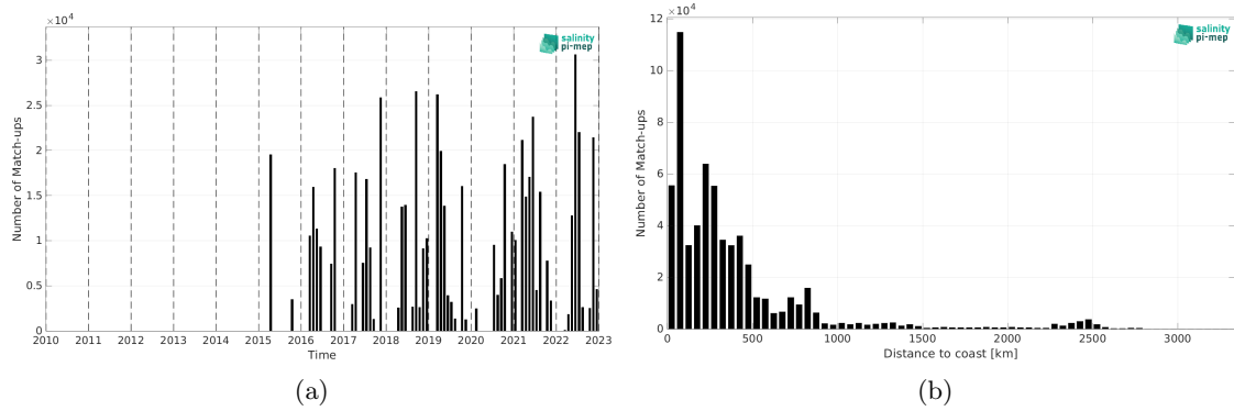
Figure 1: Number of match-ups between TSG (CSIC-UTM) and SMAP SSS L2 v5 - 40 km (RSS) SSS as a function of time (a) and as function of the distance to coast (b) over the Mid-Low Latitudes 45N-45S Pi-MEP region and for the full satellite product period.
