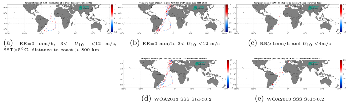
Figure 12: Temporal mean gridded over spatial boxes of size 1^\circ \times 1^\circ of \Delta\text{SSS} (SMAP SSS L2 v5 - 40 km (RSS) - TSG (CSIC-UTM)) for 5 different subdatasets corresponding to: RR=0 mm/h, 3 < U_{10} < 12 m/s, SST > 5^\circ\text{C} , distance to coast > 800 km (a), RR=0 mm/h, 3 < U_{10} < 12 m/s (b), RR > 1\text{mm/h} and U_{10} < 4\text{m/s} (c), WOA2013 SSS Std < 0.2 (d), WOA2013 SSS Std > 0.2 (e).
