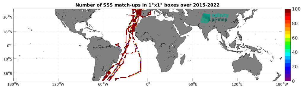
Figure 4: Number of SSS match-ups between TSG (CSIC-UTM) SSS and the SMAP SSS L2 v5 - 40 km (RSS) SSS product for the Mid-Low Latitudes 45N-45S Pi-MEP region over 1^\circ \times 1^\circ boxes and for the full satellite product period.
