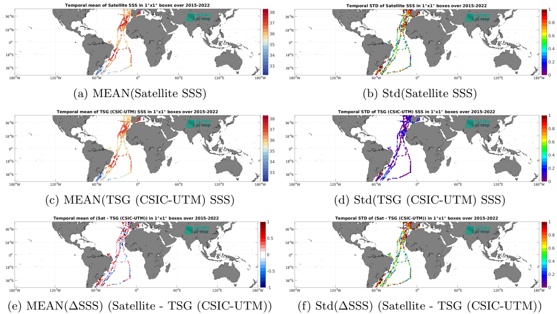
Figure 6: Temporal mean (left) and Std (right) of SSS from SMAP SSS L2 v5 - 40 km (RSS) (top), TSG (CSIC-UTM) (middle), and of \Delta SSS (Satellite - TSG (CSIC-UTM)). Only match-up pairs are used to generate these maps.
