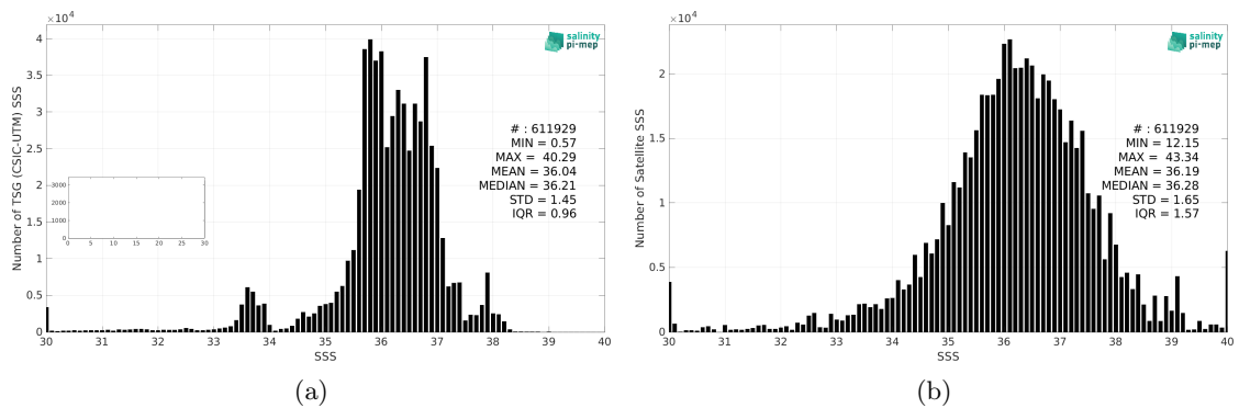
Figure 2: Histograms of SSS from TSG (CSIC-UTM) (a) and SMAP SSS L2 v5 - 40 km (RSS) (b) considering all match-up pairs per bins of 0.1 over the Mid-Low Latitudes 45N-45S Pi-MEP region and for the full satellite product period.
