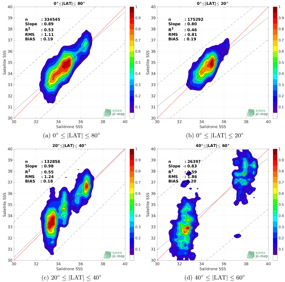
Figure 9: Contour maps of the concentration of SMAP SSS L2 v5 - 40 km (RSS) SSS (y-axis) versus Saildrone SSS (x-axis) at match-up pairs for different latitude bands. For each plot, the red line shows x=y . The black thin and dashed lines indicate a linear fit through the data cloud and the \pm 95\% confidence levels, respectively. The number match-up pairs n , the slope and R^2 coefficient of the linear fit, the root mean square (RMS) and the mean bias between satellite and in situ data are indicated for each latitude band in each plots.
