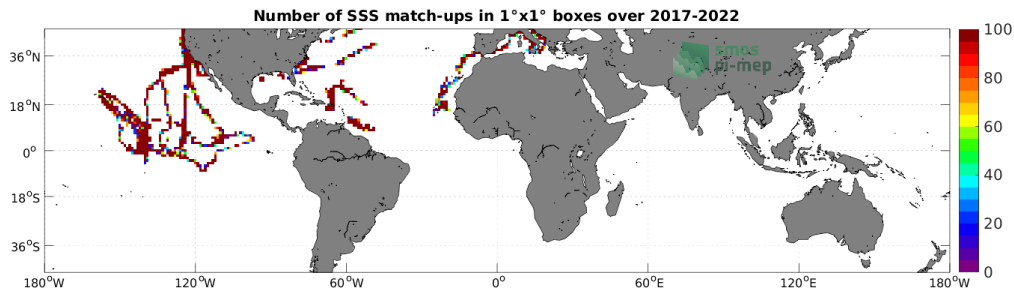
Figure 4: Number of SSS match-ups between Saildrone SSS and the SMAP SSS L2 v5 - 40 km (RSS) SSS product for the Mid-Low Latitudes 45N-45S Pi-MEP region over 1^\circ \times 1^\circ boxes and for the full satellite product period.
