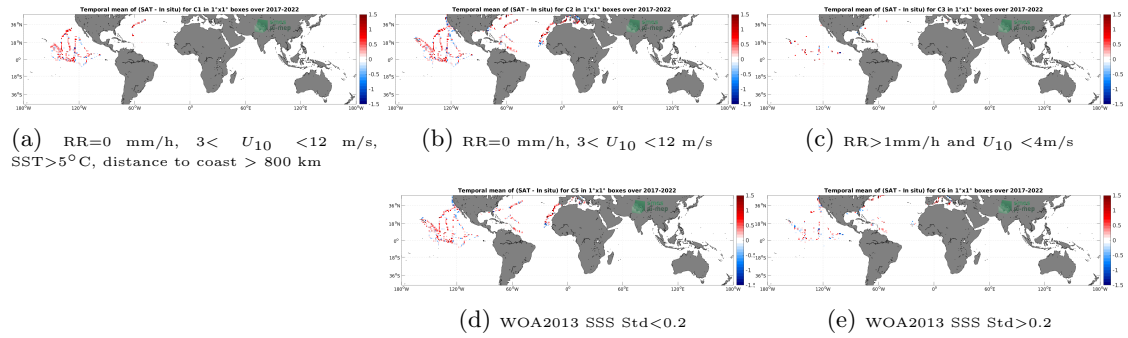
Figure 12: Temporal mean gridded over spatial boxes of size 1^\circ \times 1^\circ of \Delta SSS (SMAP SSS L2 v5 - 40 km (RSS) - Saldrone) for 5 different subdatasets corresponding to: RR=0 mm/h, 3 < U_{10} < 12 m/s, SST >5^\circ\text{C} , distance to coast > 800 km (a), RR=0 mm/h, 3 < U_{10} < 12 m/s (b), RR >1 mm/h and U_{10} < 4 m/s (c), WOA2013 SSS Std <0.2 (d), WOA2013 SSS Std >0.2 (e).
