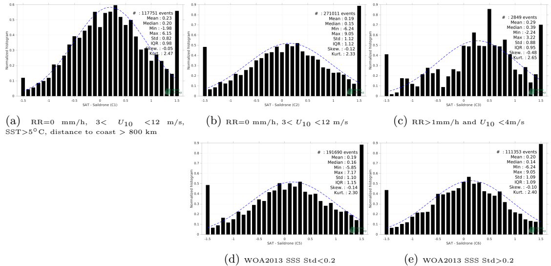
Figure 13: Normalized histogram of \Delta SSS (SMAP SSS L2 v5 - 40 km (RSS) - Saldrone) for 5 different subdatasets corresponding to: RR=0 mm/h, 3 < U_{10} < 12 m/s, SST >5^\circ\text{C} , distance to coast > 800 km (a), RR=0 mm/h, 3 < U_{10} < 12 m/s (b), RR >1 mm/h and U_{10} < 4 m/s (c), WOA2013 SSS Std <0.2 (d), WOA2013 SSS Std >0.2 (e).
