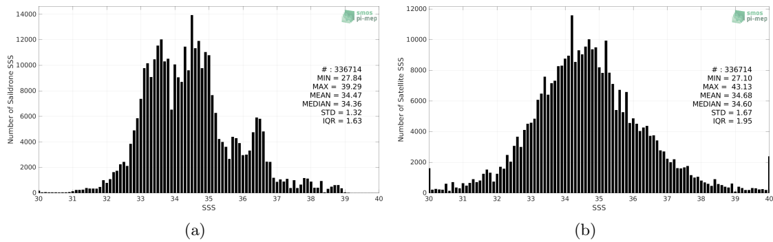
Figure 2: Histograms of SSS from Saildrone (a) and SMAP SSS L2 v5 - 40 km (RSS) (b) considering all match-up pairs per bins of 0.1 over the Mid-Low Latitudes 45N-45S Pi-MEP region and for the full satellite product period.
