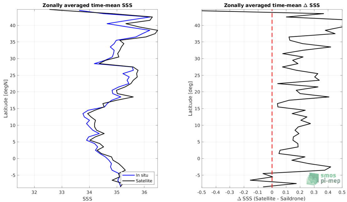
Figure 8: Left panel: Zonal mean SSS from SMAP SSS L2 v5 - 40 km (RSS) satellite product (black) and from Saildrone (blue). Right panel: Zonal mean of \Delta SSS (Satellite - Saildrone) for all the collected Pi-MEP match-up pairs estimated over the full satellite product period.
