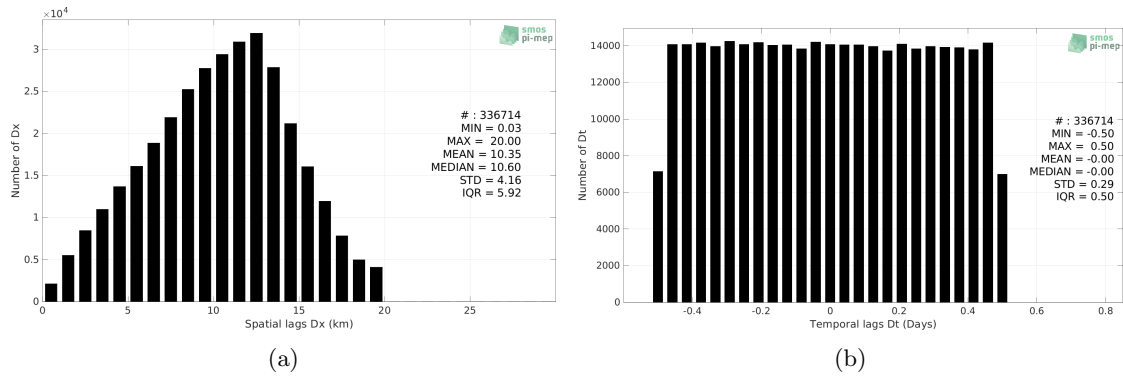
Figure 5: Histograms of the spatial (a) and temporal (b) lags between the location/time of the Saildrone measurement and the date of the corresponding SMAP SSS L2 v5 - 40 km (RSS) SSS pixel.
