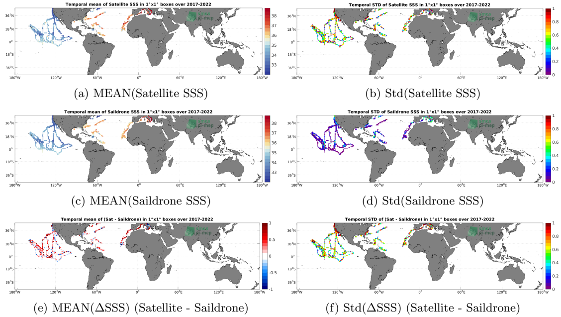
Figure 6: Temporal mean (left) and Std (right) of SSS from SMAP SSS L2 v5 - 40 km (RSS) (top), Saildrone (middle), and of \Delta SSS (Satellite - Saildrone). Only match-up pairs are used to generate these maps.
