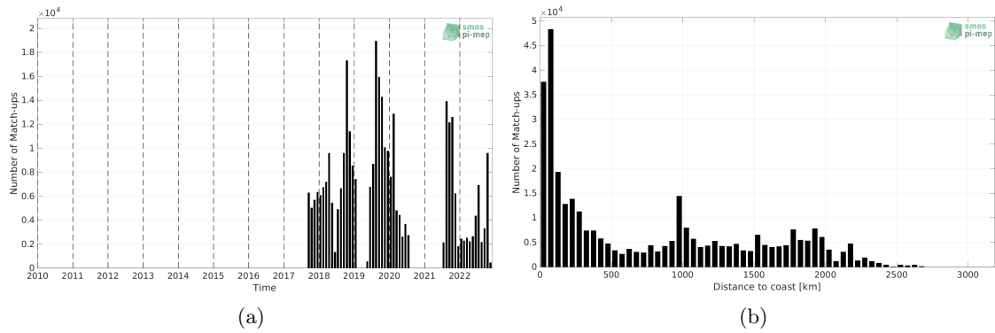
Figure 1: Number of match-ups between Saildrone and SMAP SSS L2 v5 - 40 km (RSS) SSS as a function of time (a) and as function of the distance to coast (b) over the Mid-Low Latitudes 45N-45S Pi-MEP region and for the full satellite product period.
