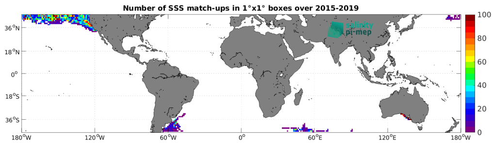
Figure 4: Number of SSS match-ups between Marine mammals SSS and the SMAP SSS L2 v5 - 40 km (RSS) SSS product for the Mid-Low Latitudes 45N-45S Pi-MEP region over 1^\circ \times 1^\circ boxes and for the full satellite product period.
