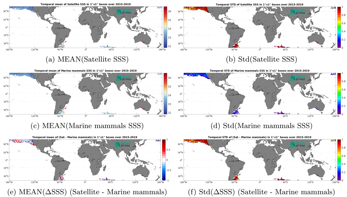
Figure 6: Temporal mean (left) and Std (right) of SSS from SMAP SSS L2 v5 - 40 km (RSS) (top), Marine mammals (middle), and of \Delta SSS (Satellite - Marine mammals). Only match-up pairs are used to generate these maps.
