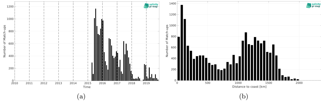
Figure 1: Number of match-ups between Marine mammals and SMAP SSS L2 v5 - 40 km (RSS) SSS as a function of time (a) and as function of the distance to coast (b) over the Mid-Low Latitudes 45N-45S Pi-MEP region and for the full satellite product period.
