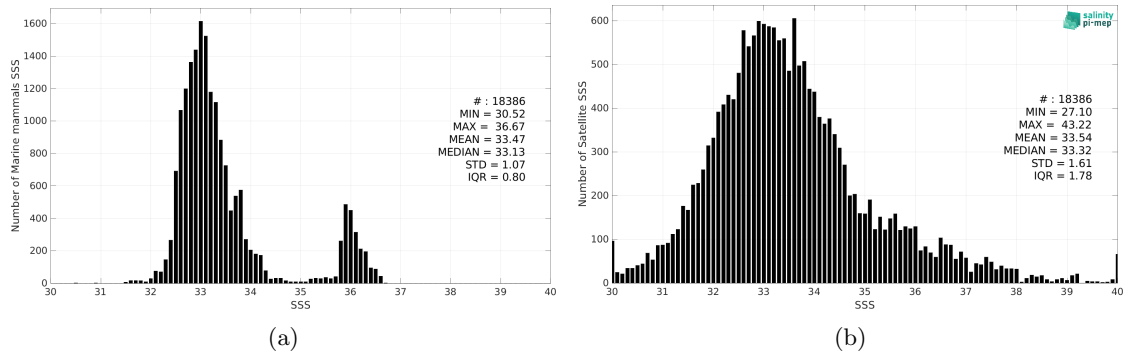
Figure 2: Histograms of SSS from Marine mammals (a) and SMAP SSS L2 v5 - 40 km (RSS) (b) considering all match-up pairs per bins of 0.1 over the Mid-Low Latitudes 45N-45S Pi-MEP region and for the full satellite product period.
