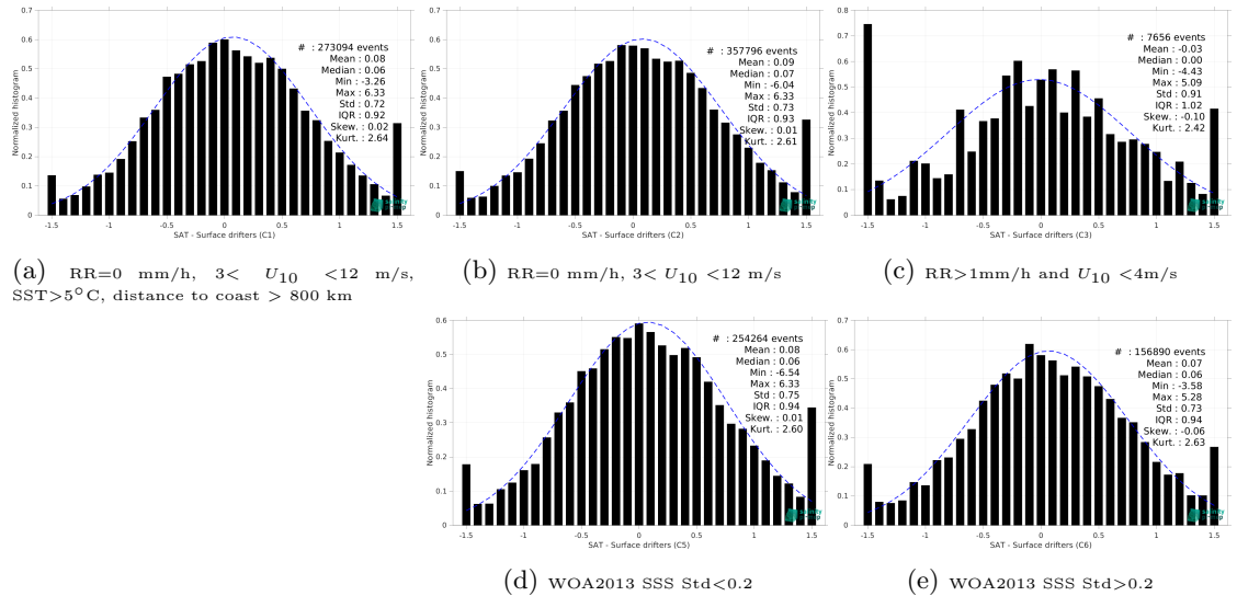
Figure 12: Normalized histogram of \Delta SSS (SMAP SSS L2 v5 - 40 km (RSS) - Surface drifters) for 5 different subdatasets corresponding to: RR=0 mm/h, 3 < U_{10} < 12 m/s, SST >5^\circ C, distance to coast > 800 km (a), RR=0 mm/h, 3 < U_{10} < 12 m/s (b), RR >1 mm/h and U_{10} < 4 m/s (c), WOA2013 SSS Std <0.2 (d), WOA2013 SSS Std >0.2 (e).
