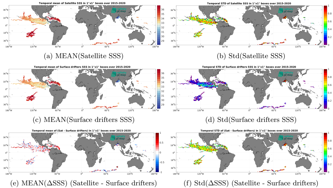
Figure 5: Temporal mean (left) and Std (right) of SSS from SMAP SSS L2 v5 - 40 km (RSS) (top), Surface drifters (middle), and of \Delta SSS (Satellite - Surface drifters). Only match-up pairs are used to generate these maps.
