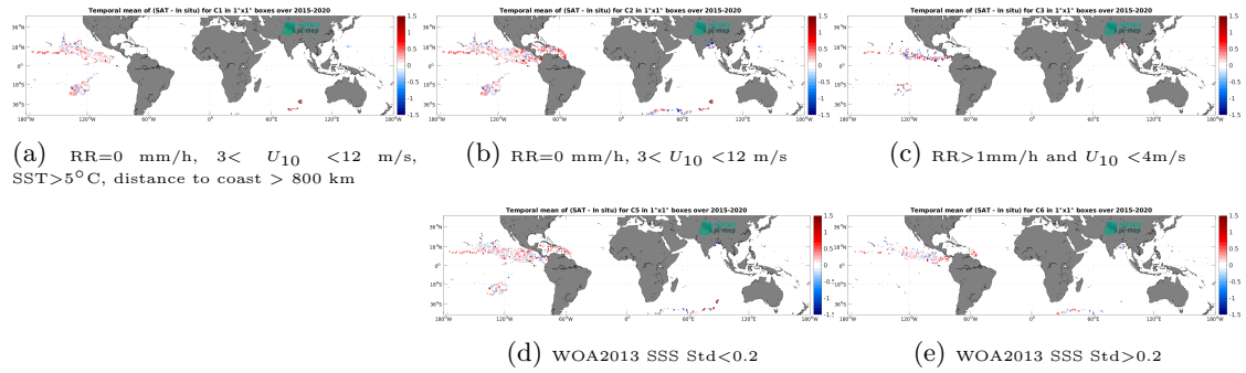
Figure 11: Temporal mean gridded over spatial boxes of size 1^\circ \times 1^\circ of \Delta SSS (SMAP SSS L2 v5 - 40 km (RSS) - Surface drifters) for 5 different subdatasets corresponding to:RR=0 mm/h, 3 < U_{10} < 12 m/s, SST >5^\circ C, distance to coast > 800 km (a), RR=0 mm/h, 3 < U_{10} < 12 m/s (b), RR >1 mm/h and U_{10} < 4 m/s (c), WOA2013 SSS Std <0.2 (d), WOA2013 SSS Std >0.2 (e).
