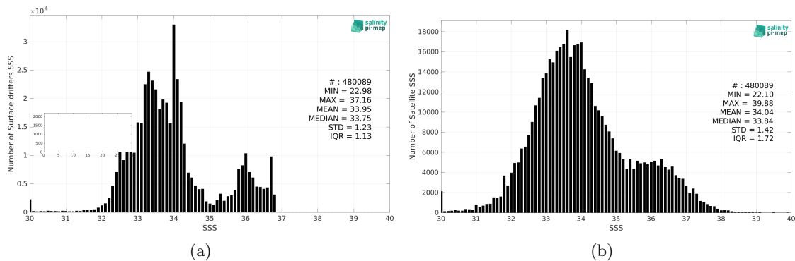
Figure 2: Histograms of SSS from Surface drifters (a) and SMAP SSS L2 v5 - 40 km (RSS) (b) considering all match-up pairs per bins of 0.1 over the Mid-Low Latitudes 45N-45S Pi-MEP region and for the full satellite product period.
