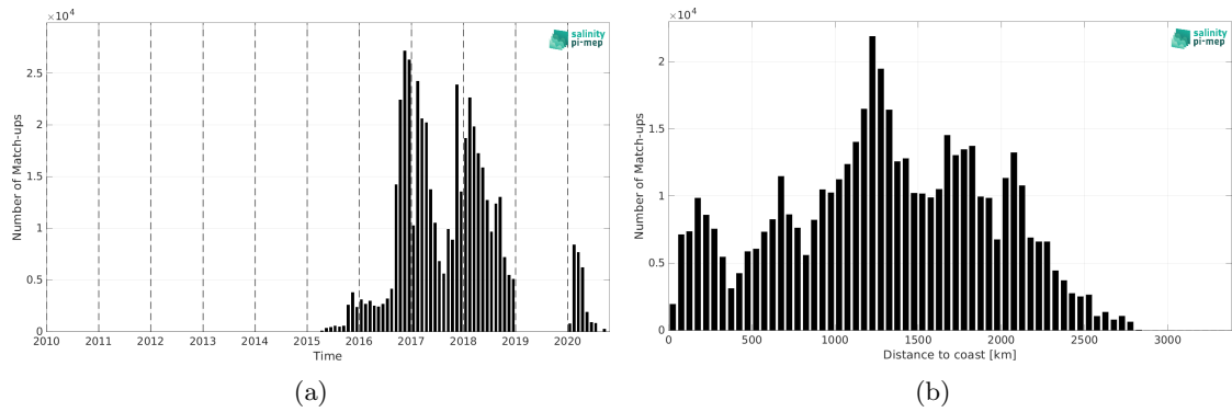
Figure 1: Number of match-ups between Surface drifters and SMAP SSS L2 v5 - 40 km (RSS) SSS as a function of time (a) and as function of the distance to coast (b) over the Mid-Low Latitudes 45N-45S Pi-MEP region and for the full satellite product period.
