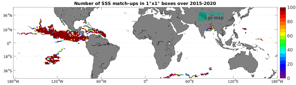
Figure 3: Number of SSS match-ups between Surface drifters SSS and the SMAP SSS L2 v5 - 40 km (RSS) SSS product for the Mid-Low Latitudes 45N-45S Pi-MEP region over 1^\circ \times 1^\circ boxes and for the full satellite product period.
