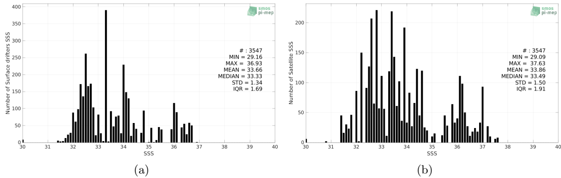
Figure 2: Histograms of SSS from Surface drifters (a) and SMAP SSS L2 v5 - 40 km (RSS) (b) considering all match-up pairs per bins of 0.1 over the Mid-Low Latitudes 45N-45S Pi-MEP region and for the full satellite product period.
