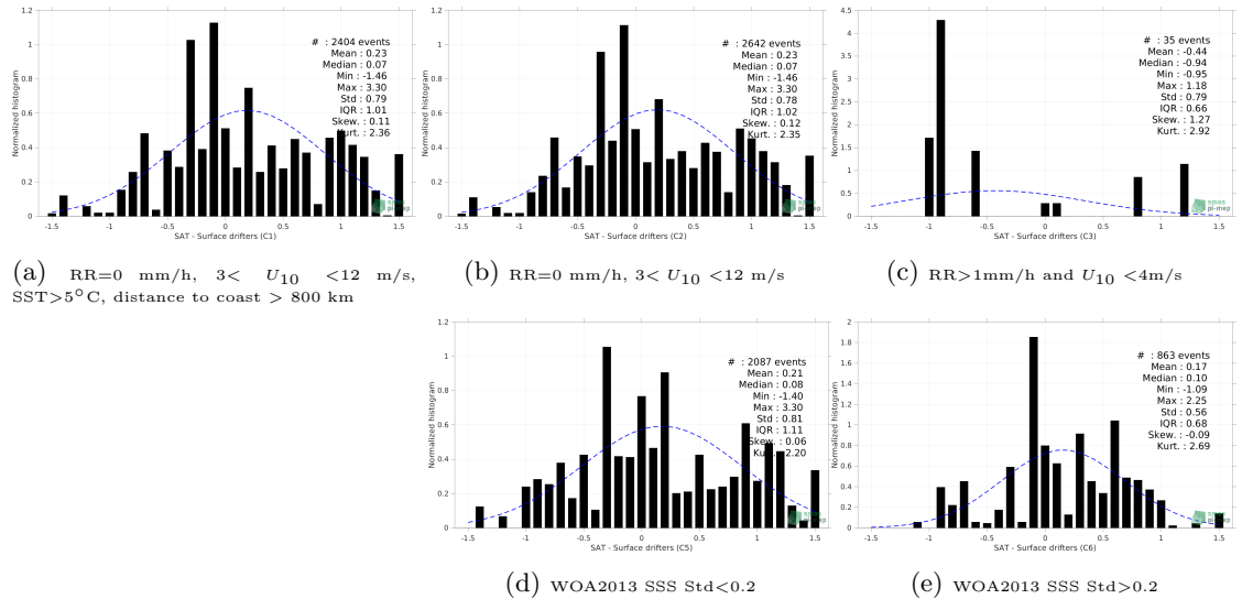
Figure 12: Normalized histogram of \Delta SSS (SMAP SSS L2 v5 - 40 km (RSS) - Surface drifters) for 5 different subdatasets corresponding to: RR=0 mm/h, 3 < U_{10} < 12 m/s, SST>5°C, distance to coast > 800 km (a), RR=0 mm/h, 3 < U_{10} < 12 m/s (b), RR>1mm/h and U_{10} < 4 m/s (c), WOA2013 SSS Std<0.2 (d), WOA2013 SSS Std>0.2 (e).
