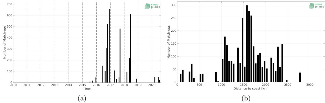
Figure 1: Number of match-ups between Surface drifters and SMAP SSS L2 v5 - 40 km (RSS) SSS as a function of time (a) and as function of the distance to coast (b) over the Mid-Low Latitudes 45N-45S Pi-MEP region and for the full satellite product period.
