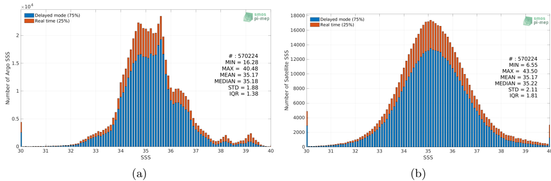
Figure 2: Histograms of SSS from Argo (a) and SMAP SSS L2 v5 - 40 km (RSS) (b) considering all match-up pairs per bins of 0.1 over the Mid-Low Latitudes 45N-45S Pi-MEP region and for the full satellite product period.
