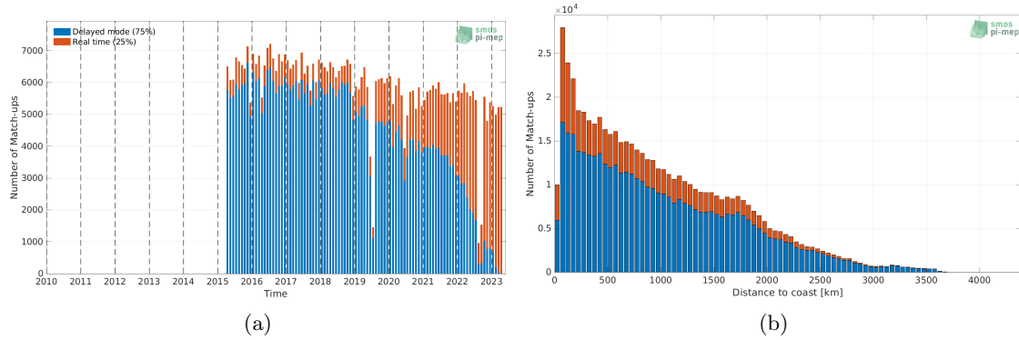
Figure 1: Number of match-ups between Argo and SMAP SSS L2 v5 - 40 km (RSS) SSS as a function of time (a) and as function of the distance to coast (b) over the Mid-Low Latitudes 45N-45S Pi-MEP region and for the full satellite product period.
