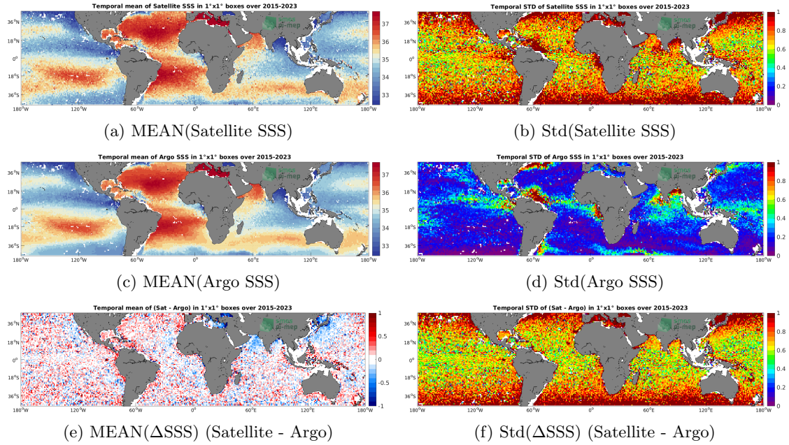
Figure 6: Temporal mean (left) and Std (right) of SSS from SMAP SSS L2 v5 - 40 km (RSS) (top), Argo (middle), and of \Delta SSS (Satellite - Argo). Only match-up pairs are used to generate these maps.
