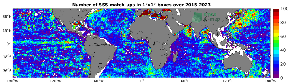
Figure 4: Number of SSS match-ups between Argo SSS and the SMAP SSS L2 v5 - 40 km (RSS) SSS product for the Mid-Low Latitudes 45N-45S Pi-MEP region over 1^\circ \times 1^\circ boxes and for the full satellite product period.
