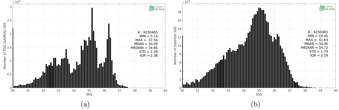
Figure 2: Histograms of SSS from TSG (SAMOS) (a) and SMAP SSS L2 v4 (RSS) (b) considering all match-up pairs per bins of 0.1 over the Mid-Low Latitudes 45N-45S Pi-MEP region and for the full satellite product period.
