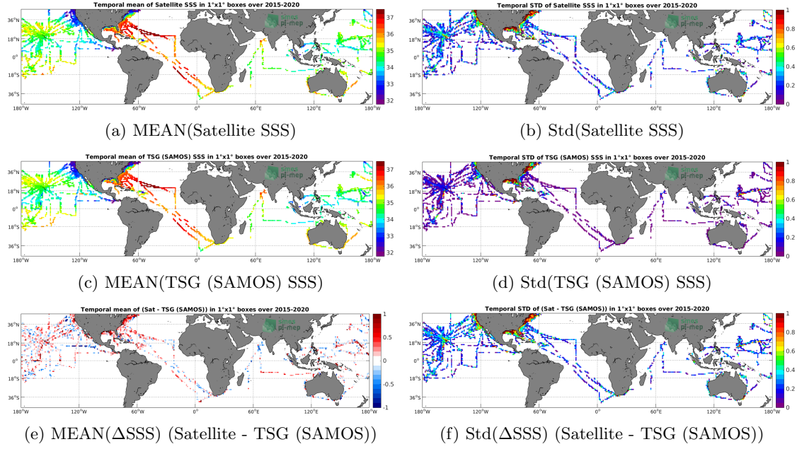
Figure 6: Temporal mean (left) and Std (right) of SSS from SMAP SSS L2 v4 (RSS) (top), TSG (SAMOS) (middle), and of \Delta SSS (Satellite - TSG (SAMOS)). Only match-up pairs are used to generate these maps.
