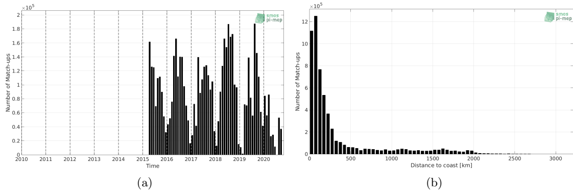
Figure 1: Number of match-ups between TSG (SAMOS) and SMAP SSS L2 v4 (RSS) SSS as a function of time (a) and as function of the distance to coast (b) over the Mid-Low Latitudes 45N-45S Pi-MEP region and for the full satellite product period.
