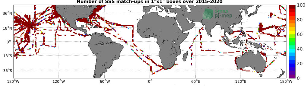
Figure 4: Number of SSS match-ups between TSG (SAMOS) SSS and the SMAP SSS L2 v4 (RSS) SSS product for the Mid-Low Latitudes 45N-45S Pi-MEP region over 1^\circ \times 1^\circ boxes and for the full satellite product period.
