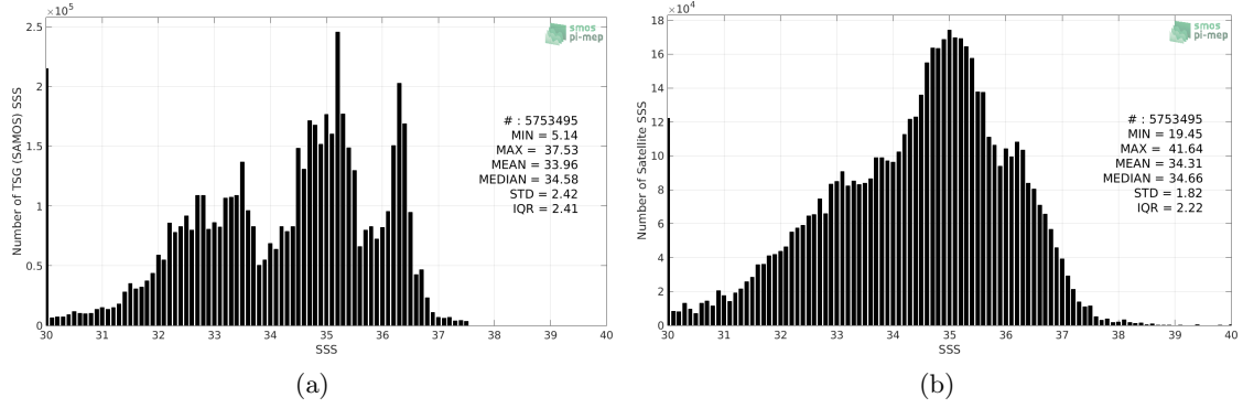
Figure 2: Histograms of SSS from TSG (SAMOS) (a) and SMAP SSS L2 v4 (RSS) (b) considering all match-up pairs per bins of 0.1 over the Mid-Low Latitudes 45N-45S Pi-MEP region and for the full satellite product period.
