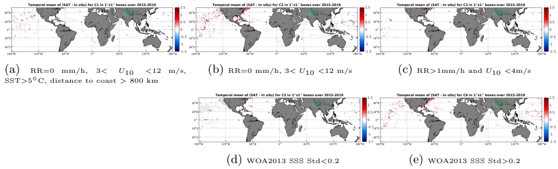
Figure 12: Temporal mean gridded over spatial boxes of size 1^\circ \times 1^\circ of \Delta SSS (SMAP-L2-RSS-V4 - TSG-SAMOS) for 5 different subdatasets corresponding to: RR=0 mm/h, 3 < U_{10} < 12 m/s, SST >5^\circ\text{C} , distance to coast > 800 km (a), RR=0 mm/h, 3 < U_{10} < 12 m/s (b), RR >1 mm/h and U_{10} < 4 m/s (c), WOA2013 SSS Std <0.2 (d), WOA2013 SSS Std >0.2 (e).
