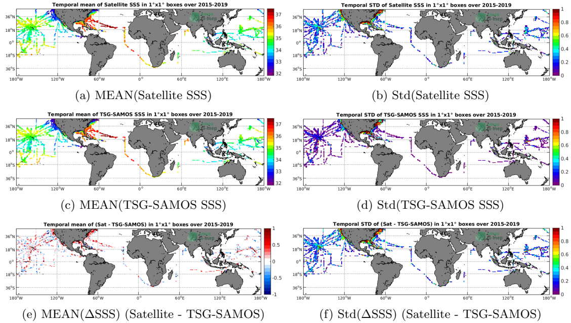
Figure 6: Temporal mean (left) and Std (right) of SSS from SMAP-L2-RSS-V4 (top), TSG-SAMOS (middle), and of \Delta SSS (Satellite - TSG-SAMOS). Only match-up pairs are used to generate these maps.
