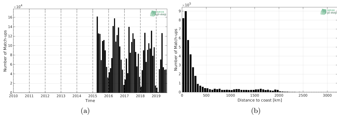
Figure 1: Number of match-ups between TSG-SAMOS and SMAP-L2-RSS-V4 SSS as a function of time (a) and as function of the distance to coast (b) over the Mid-Low Latitudes 45N-45S Pi-MEP region and for the full satellite product period.
