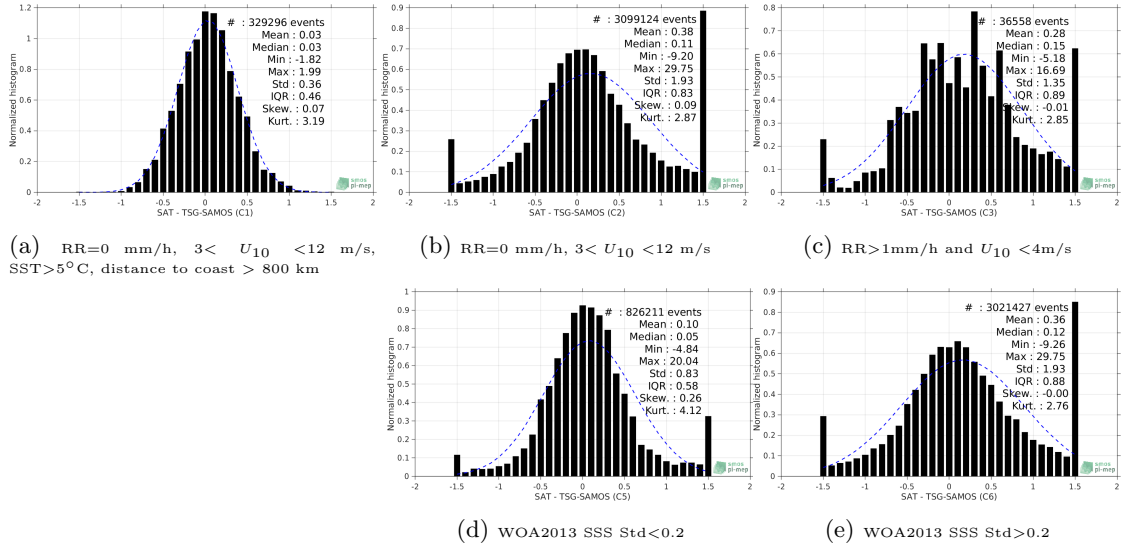
Figure 13: Normalized histogram of \Delta SSS (SMAP-L2-RSS-V4 - TSG-SAMOS) for 5 different subdatasets corresponding to: RR=0 mm/h, 3 < U_{10} < 12 m/s, SST >5^\circ\text{C} , distance to coast > 800 km (a), RR=0 mm/h, 3 < U_{10} < 12 m/s (b), RR >1 mm/h and U_{10} < 4 m/s (c), WOA2013 SSS Std <0.2 (d), WOA2013 SSS Std >0.2 (e).
