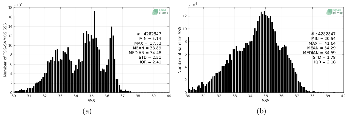
Figure 2: Histograms of SSS from TSG-SAMOS (a) and SMAP-L2-RSS-V4 (b) considering all match-up pairs per bins of 0.1 over the Mid-Low Latitudes 45N-45S Pi-MEP region and for the full satellite product period.
