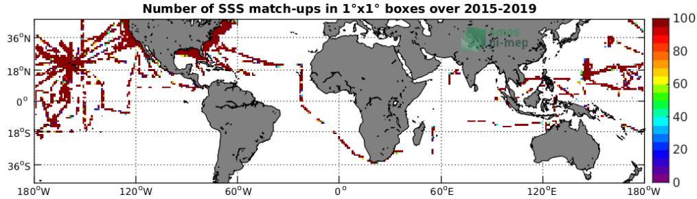
Figure 4: Number of SSS match-ups between TSG-SAMOS SSS and the SMAP-L2-RSS-V4 SSS product for the Mid-Low Latitudes 45N-45S Pi-MEP region over 1^\circ \times 1^\circ boxes and for the full satellite product period.
