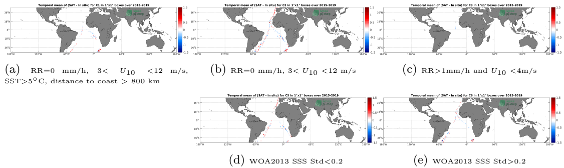
Figure 12: Temporal mean gridded over spatial boxes of size 1^\circ \times 1^\circ of \Delta\text{SSS} (SMAP SSS L2 v4 (RSS) - TSG (Polarstern)) for 5 different subdatasets corresponding to: RR=0 mm/h, 3 < U_{10} < 12 m/s, SST>5°C, distance to coast > 800 km (a), RR=0 mm/h, 3 < U_{10} < 12 m/s (b), RR>1mm/h and U_{10} < 4 m/s (c), WOA2013 SSS Std<0.2 (d), WOA2013 SSS Std>0.2 (e).
