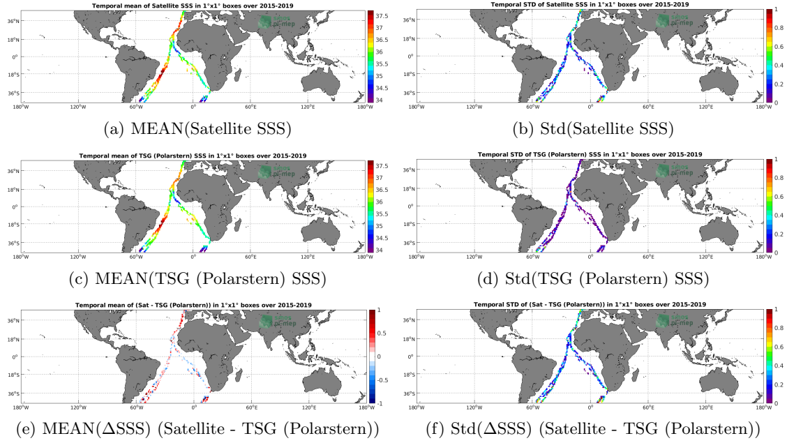
Figure 6: Temporal mean (left) and Std (right) of SSS from SMAP SSS L2 v4 (RSS) (top), TSG (Polarstern) (middle), and of \Delta SSS (Satellite - TSG (Polarstern)). Only match-up pairs are used to generate these maps.
