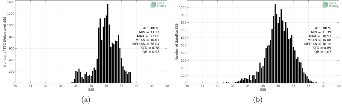
Figure 2: Histograms of SSS from TSG (Polarstern) (a) and SMAP SSS L2 v4 (RSS) (b) considering all match-up pairs per bins of 0.1 over the Mid-Low Latitudes 45N-45S Pi-MEP region and for the full satellite product period.
