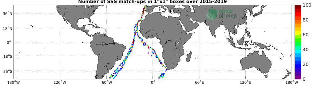
Figure 4: Number of SSS match-ups between TSG (Polarstern) SSS and the SMAP SSS L2 v4 (RSS) SSS product for the Mid-Low Latitudes 45N-45S Pi-MEP region over 1^\circ \times 1^\circ boxes and for the full satellite product period.
