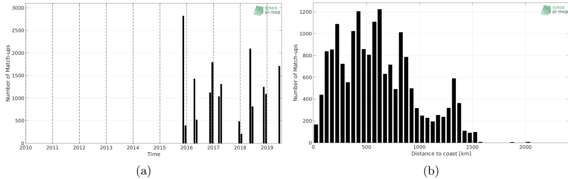
Figure 1: Number of match-ups between TSG (Polarstern) and SMAP SSS L2 v4 (RSS) SSS as a function of time (a) and as function of the distance to coast (b) over the Mid-Low Latitudes 45N-45S Pi-MEP region and for the full satellite product period.
