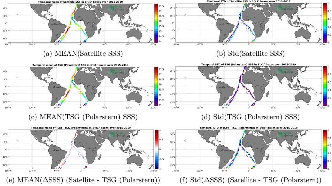
Figure 6: Temporal mean (left) and Std (right) of SSS from SMAP SSS L2 v4 (RSS) (top), TSG (Polarstern) (middle), and of \Delta SSS (Satellite - TSG (Polarstern)). Only match-up pairs are used to generate these maps.
