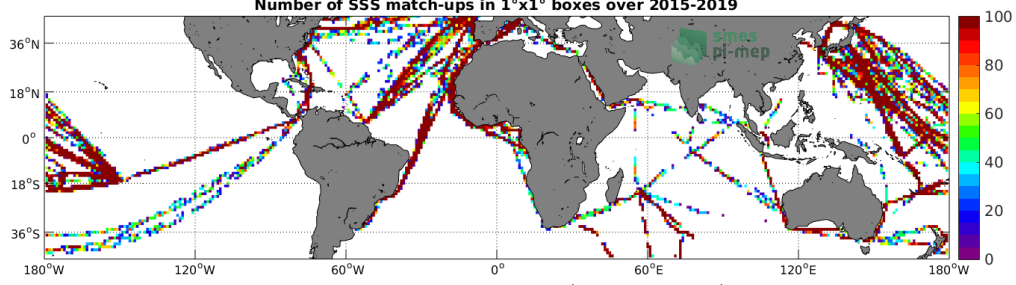
Figure 4: Number of SSS match-ups between TSG (LEGOS-DM) SSS and the SMAP SSS L2 v4 (RSS) SSS product for the Mid-Low Latitudes 45N-45S Pi-MEP region over 1^\circ \times 1^\circ boxes and for the full satellite product period.
