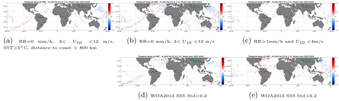
Figure 12: Temporal mean gridded over spatial boxes of size 1^\circ \times 1^\circ of \Delta SSS (SMAP SSS L2 v4 (RSS) - TSG (LEGOS-DM)) for 5 different subdatasets corresponding to: RR=0 mm/h, 3 < U_{10} < 12 m/s, SST > 5^\circ C , distance to coast > 800 km (a), RR=0 mm/h, 3 < U_{10} < 12 m/s (b), RR > 1 mm/h and U_{10} < 4 m/s (c), WOA2013 SSS Std < 0.2 (d), WOA2013 SSS Std > 0.2 (e).
