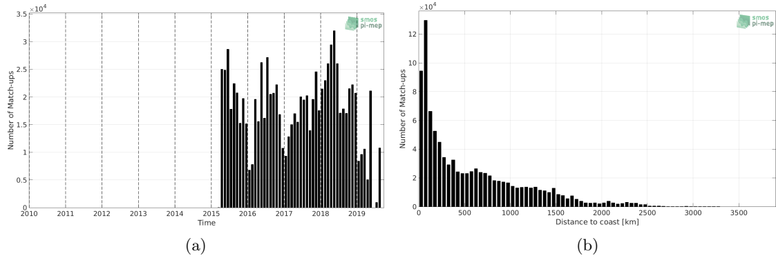
Figure 1: Number of match-ups between TSG (LEGOS-DM) and SMAP SSS L2 v4 (RSS) SSS as a function of time (a) and as function of the distance to coast (b) over the Mid-Low Latitudes 45N-45S Pi-MEP region and for the full satellite product period.
