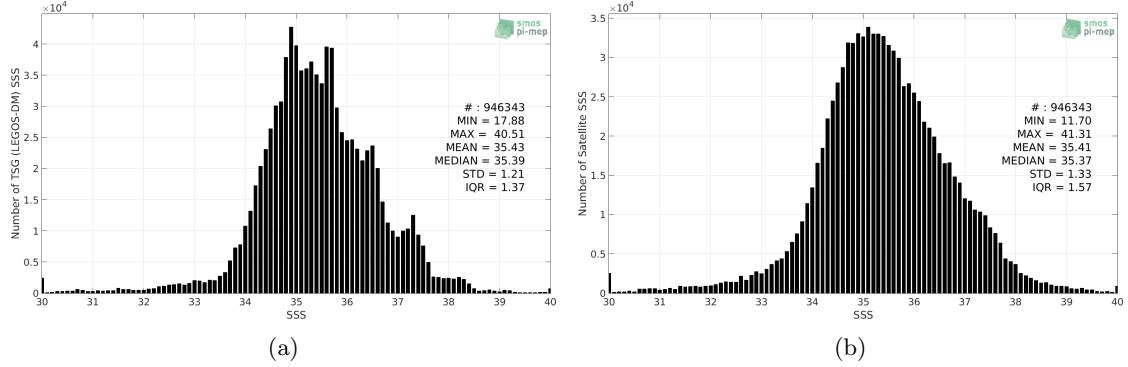
Figure 2: Histograms of SSS from TSG (LEGOS-DM) (a) and SMAP SSS L2 v4 (RSS) (b) considering all match-up pairs per bins of 0.1 over the Mid-Low Latitudes 45N-45S Pi-MEP region and for the full satellite product period.
