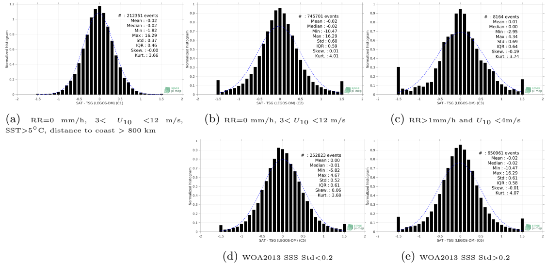
Figure 13: Normalized histogram of \Delta SSS (SMAP SSS L2 v4 (RSS) - TSG (LEGOS-DM)) for 5 different subdatasets corresponding to: RR=0 mm/h, 3 < U_{10} < 12 m/s, SST > 5^\circ C , distance to coast > 800 km (a), RR=0 mm/h, 3 < U_{10} < 12 m/s (b), RR > 1 mm/h and U_{10} < 4 m/s (c), WOA2013 SSS Std < 0.2 (d), WOA2013 SSS Std > 0.2 (e).
