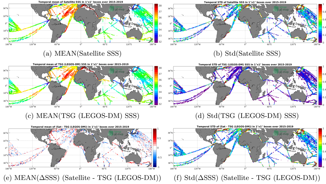
Figure 6: Temporal mean (left) and Std (right) of SSS from SMAP SSS L2 v4 (RSS) (top), TSG (LEGOS-DM) (middle), and of \Delta SSS (Satellite - TSG (LEGOS-DM)). Only match-up pairs are used to generate these maps.
