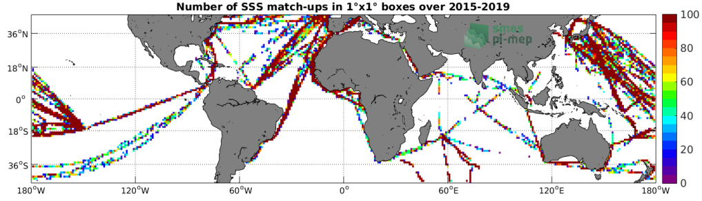
Figure 4: Number of SSS match-ups between TSG-LEGOS-DM SSS and the SMAP-L2-RSS-V4 SSS product for the Mid-Low Latitudes 45N-45S Pi-MEP region over 1^\circ \times 1^\circ boxes and for the full satellite product period.
