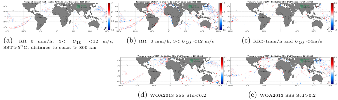
Figure 12: Temporal mean gridded over spatial boxes of size 1^\circ \times 1^\circ of \Delta SSS (SMAP-L2-RSS-V4 - TSG-LEGOS-DM) for 5 different subdatasets corresponding to:RR=0 mm/h, 3 < U_{10} < 12 m/s, SST >5^\circ\text{C} , distance to coast > 800 km (a), RR=0 mm/h, 3 < U_{10} < 12 m/s (b), RR >1 mm/h and U_{10} < 4 m/s (c), WOA2013 SSS Std <0.2 (d), WOA2013 SSS Std >0.2 (e).
