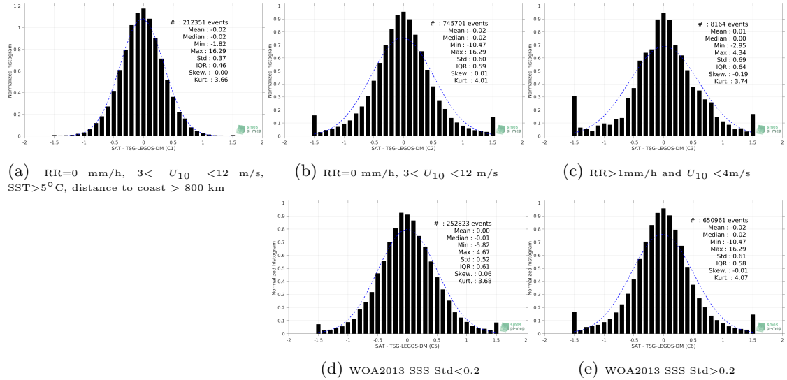
Figure 13: Normalized histogram of \Delta SSS (SMAP-L2-RSS-V4 - TSG-LEGOS-DM) for 5 different subdatasets corresponding to: RR=0 mm/h, 3 < U_{10} < 12 m/s, SST >5^\circ\text{C} , distance to coast > 800 km (a), RR=0 mm/h, 3 < U_{10} < 12 m/s (b), RR >1 mm/h and U_{10} < 4 m/s (c), WOA2013 SSS Std <0.2 (d), WOA2013 SSS Std >0.2 (e).
