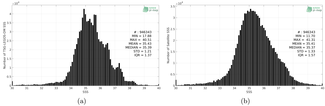
Figure 2: Histograms of SSS from TSG-LEGOS-DM (a) and SMAP-L2-RSS-V4 (b) considering all match-up pairs per bins of 0.1 over the Mid-Low Latitudes 45N-45S Pi-MEP region and for the full satellite product period.
