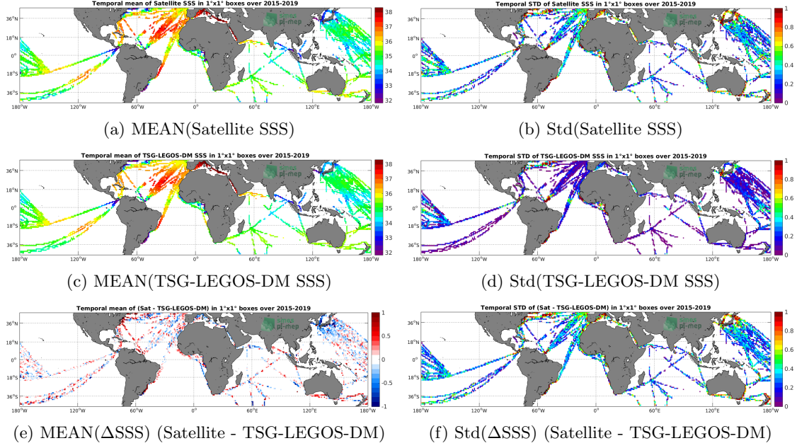
Figure 6: Temporal mean (left) and Std (right) of SSS from SMAP-L2-RSS-V4 (top), TSG-LEGOS-DM (middle), and of \Delta SSS (Satellite - TSG-LEGOS-DM). Only match-up pairs are used to generate these maps.
