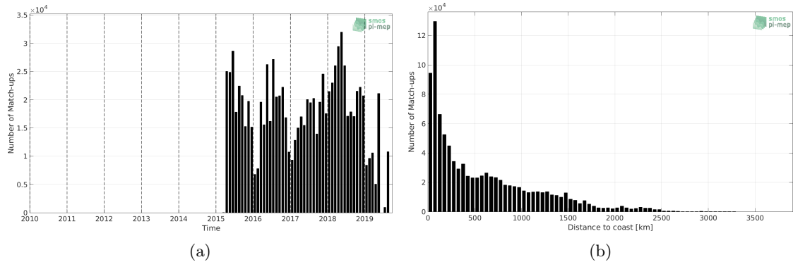
Figure 1: Number of match-ups between TSG-LEGOS-DM and SMAP-L2-RSS-V4 SSS as a function of time (a) and as function of the distance to coast (b) over the Mid-Low Latitudes 45N-45S Pi-MEP region and for the full satellite product period.
