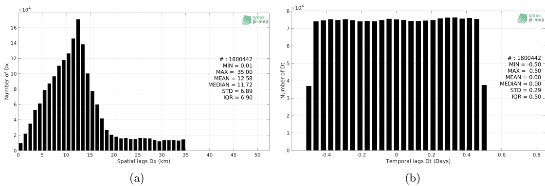
Figure 5: Histograms of the spatial (a) and temporal (b) lags between the location/time of the TSG (GOSUD-Research-vessel) measurement and the date of the corresponding SMAP SSS L2 v4 (RSS) SSS pixel.
