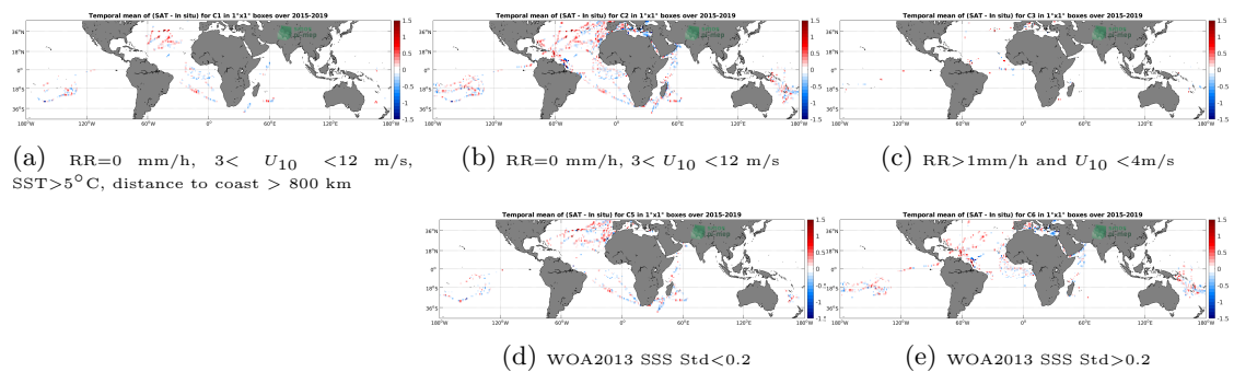
Figure 12: Temporal mean gridded over spatial boxes of size 1^\circ \times 1^\circ of \Delta\text{SSS} (SMAP SSS L2 v4 (RSS) - TSG (GOSUD-Research-vessel)) for 5 different subdatasets corresponding to:RR=0 mm/h, 3 < U_{10} < 12 m/s, SST>5°C, distance to coast > 800 km (a), RR=0 mm/h, 3 < U_{10} < 12 m/s (b), RR>1mm/h and U_{10} < 4 m/s (c), WOA2013 SSS Std<0.2 (d), WOA2013 SSS Std>0.2 (e).
