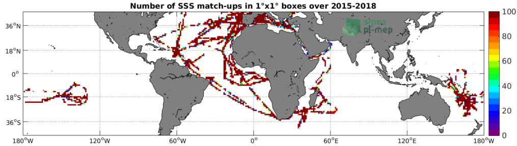
Figure 4: Number of SSS match-ups between TSG-GOSUD-Research-vessel SSS and the SMAP-L2-RSS-V4 SSS product for the Mid-Low Latitudes 45N-45S Pi-MEP region over 1^\circ \times 1^\circ boxes and for the full satellite product period.
