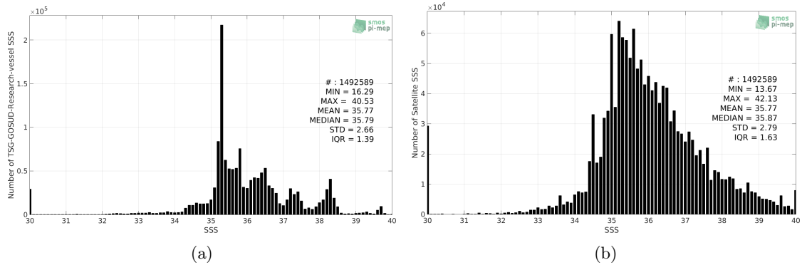
Figure 2: Histograms of SSS from TSG-GOSUD-Research-vessel (a) and SMAP-L2-RSS-V4 (b) considering all match-up pairs per bins of 0.1 over the Mid-Low Latitudes 45N-45S Pi-MEP region and for the full satellite product period.
