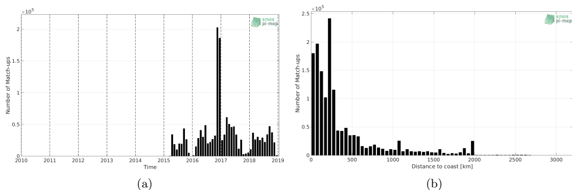
Figure 1: Number of match-ups between TSG-GOSUD-Research-vessel and SMAP-L2-RSS-V4 SSS as a function of time (a) and as function of the distance to coast (b) over the Mid-Low Latitudes 45N-45S Pi-MEP region and for the full satellite product period.
