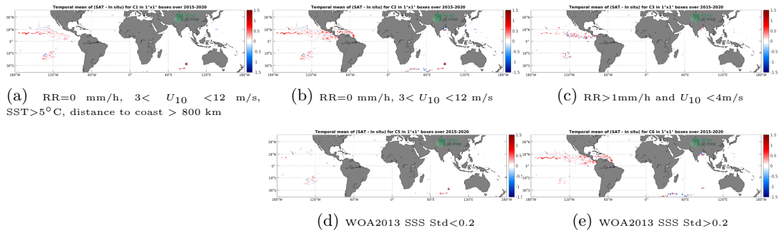
Figure 11: Temporal mean gridded over spatial boxes of size 1^\circ \times 1^\circ of \Delta SSS (SMAP SSS L2 v4 (RSS) - Surface drifters) for 5 different subdatasets corresponding to:RR=0 mm/h, 3 < U_{10} < 12 m/s, SST>5°C, distance to coast > 800 km (a), RR=0 mm/h, 3 < U_{10} < 12 m/s (b), RR>1mm/h and U_{10} < 4 m/s (c), WOA2013 SSS Std<0.2 (d), WOA2013 SSS Std>0.2 (e).
