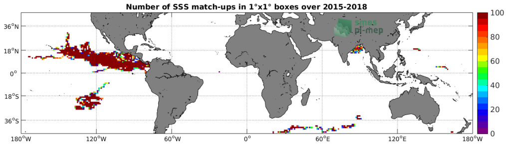
Figure 3: Number of SSS match-ups between Surface drifters SSS and the SMAP SSS L2 v4 (RSS) SSS product for the Mid-Low Latitudes 45N-45S Pi-MEP region over 1^\circ \times 1^\circ boxes and for the full satellite product period.
