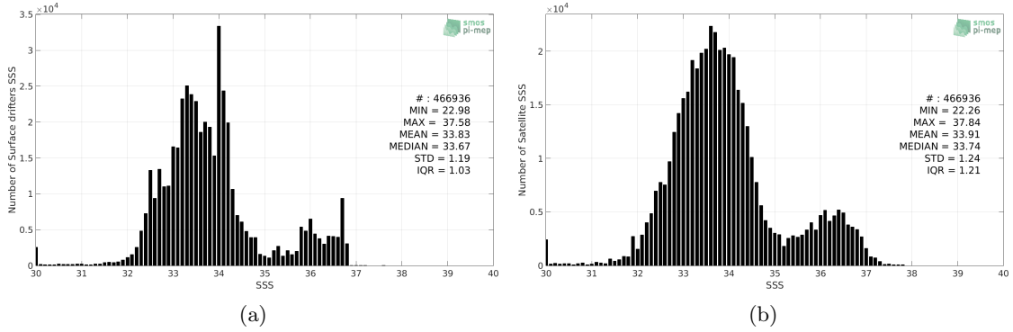
Figure 2: Histograms of SSS from Surface drifters (a) and SMAP SSS L2 v4 (RSS) (b) considering all match-up pairs per bins of 0.1 over the Mid-Low Latitudes 45N-45S Pi-MEP region and for the full satellite product period.
