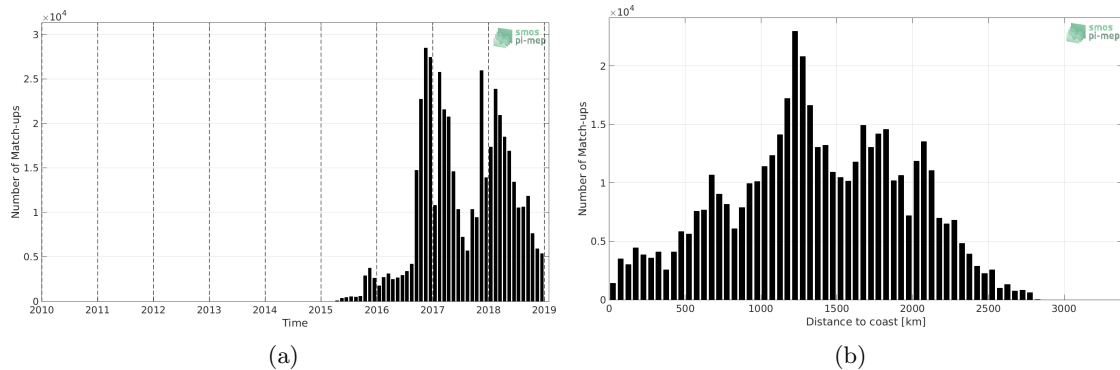
Figure 1: Number of match-ups between Surface drifters and SMAP SSS L2 v4 (RSS) SSS as a function of time (a) and as function of the distance to coast (b) over the Mid-Low Latitudes 45N-45S Pi-MEP region and for the full satellite product period.
