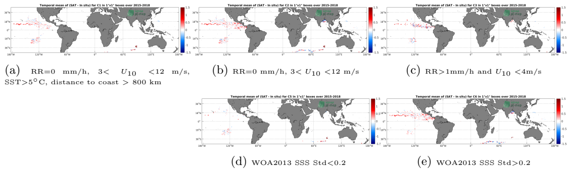
Figure 11: Temporal mean gridded over spatial boxes of size 1°x1° of \Delta SSS (SMAP SSS L2 v4 (RSS) - Surface drifters) for 5 different subdatasets corresponding to:RR=0 mm/h, 3 < U_{10} < 12 m/s, SST>5°C, distance to coast > 800 km (a), RR=0 mm/h, 3 < U_{10} < 12 m/s (b), RR>1mm/h and U_{10} <4m/s (c), WOA2013 SSS Std<0.2 (d), WOA2013 SSS Std>0.2 (e).
