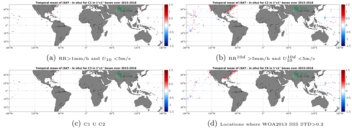
Figure 12: Temporal mean gridded over spatial boxes of size 1^\circ \times 1^\circ of \Delta SSS (SMAP-L2-RSS-V3-70KM - TSG-SAMOS) for 4 different subdatasets corresponding to: RR > 1\text{mm/h} and U_{10} < 5\text{m/s} (a), RR^{10d} > 5\text{mm/h} and U_{10}^{10d} < 5\text{m/s} (b), C1 U C2 (c), Locations where WOA2013 SSS STD > 0.2 (d).
