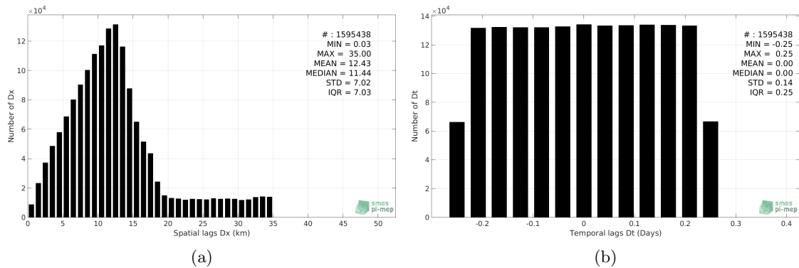
Figure 5: Histograms of the spatial (a) and temporal (b) lags between the time of the TSG-SAMOS measurements and the date of the corresponding SMAP-L2-RSS-V3-70KM SSS product.
