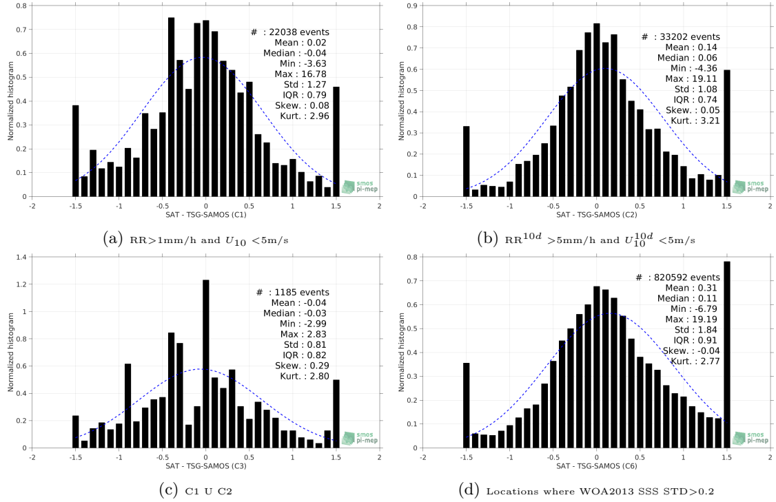
Figure 13: Normalized histogram of \Delta\text{SSS} (SMAP-L2-RSS-V3-70KM - TSG-SAMOS) for 6 different subdatasets corresponding to: RR > 1\text{mm/h} and U_{10} < 5\text{m/s} (a), RR^{10d} > 5\text{mm/h} and U_{10}^{10d} < 5\text{m/s} (b), C1 U C2 (c), Locations where WOA2013 SSS STD > 0.2 (d).
