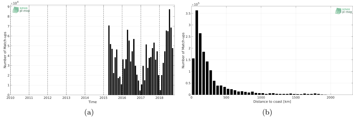
Figure 1: Number of match-ups between TSG-SAMOS and SMAP-L2-RSS-V3-70KM SSS as a function of time (a) and as function of the distance to coast (b) over the Mid-Low Latitudes 45N-45S Pi-MEP region and for the full satellite product period.
