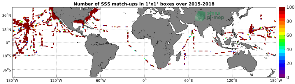
Figure 4: Number of SSS match-ups between TSG-SAMOS SSS and the SMAP-L2-RSS-V3-70KM SSS product for the Mid-Low Latitudes 45N-45S Pi-MEP region over 1^\circ \times 1^\circ boxes and for the full satellite product period.
