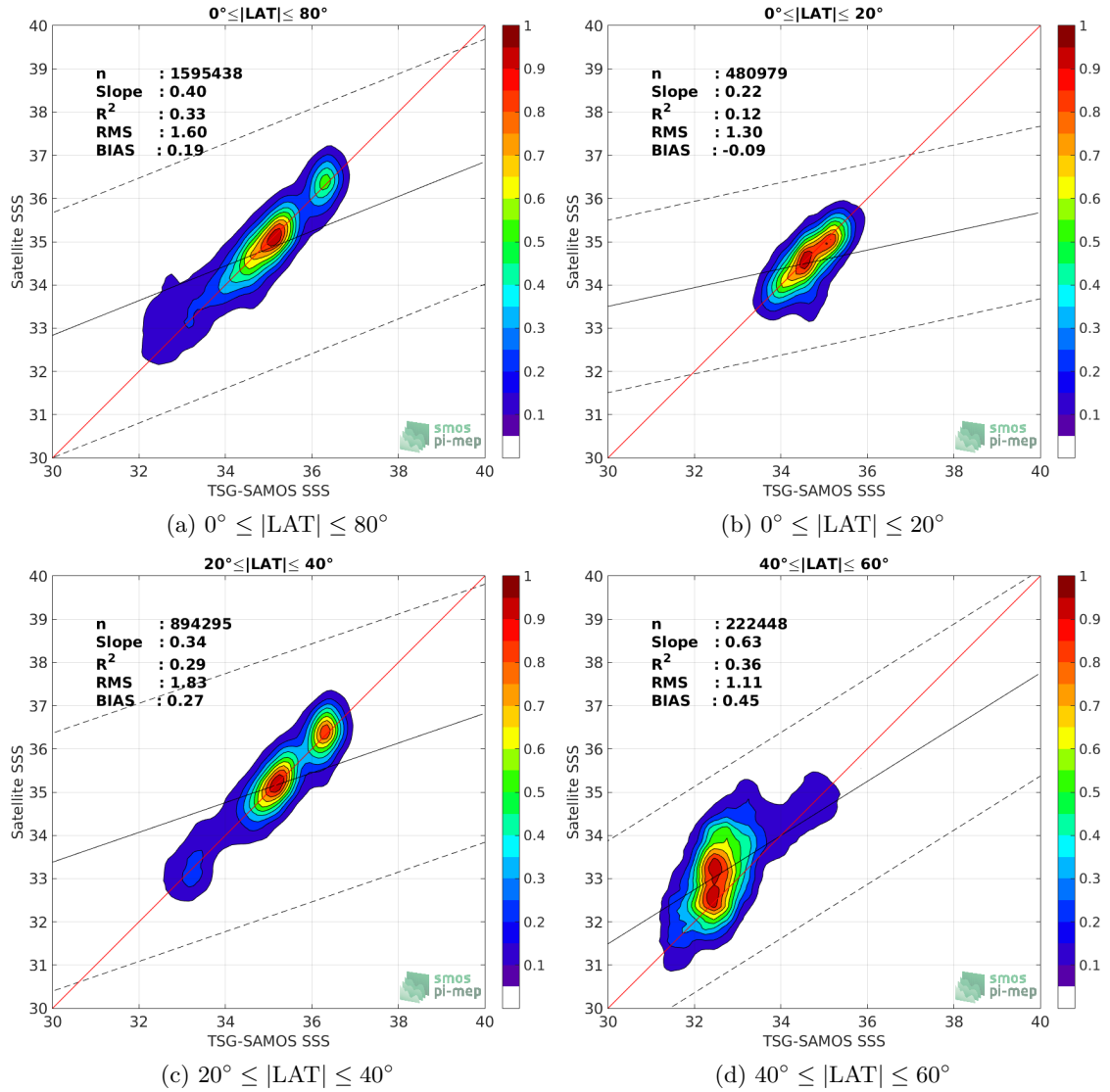
Figure 9: Contour maps of the concentration of SMAP-L2-RSS-V3-70KM SSS (y-axis) versus TSG-SAMOS SSS (x-axis) at match-up pairs for different latitude bands. For each plot, the red line shows x=y . The black thin and dashed lines indicate a linear fit through the data cloud and the \pm 95\% confidence levels, respectively. The number match-up pairs n , the slope and R^2 coefficient of the linear fit, the root mean square (RMS) and the mean bias between satellite and in situ data are indicated for each latitude band in each plots.
