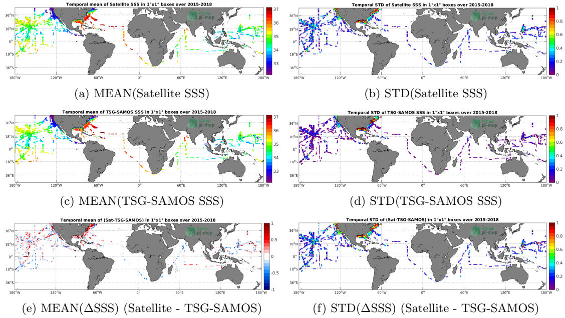
Figure 6: Temporal mean (left) and STD (right) of SSS from SMAP-L2-RSS-V3-70KM (top), TSG-SAMOS (middle), and of \Delta SSS (Satellite - TSG-SAMOS). Only match-up pairs are used to generate these maps.
