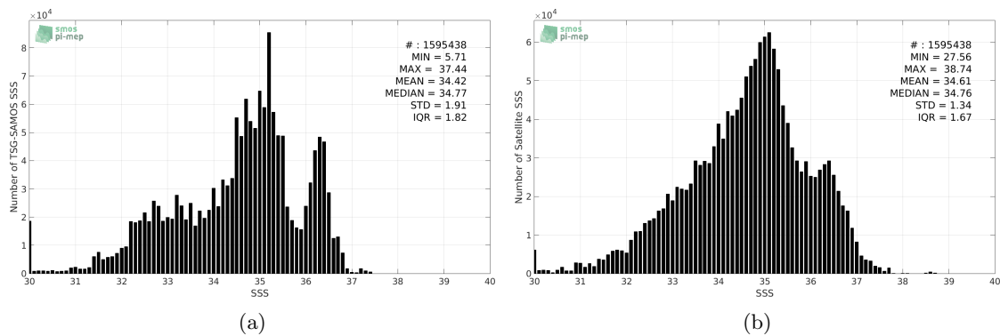
Figure 2: Histograms of SSS from TSG-SAMOS (a) and SMAP-L2-RSS-V3-70KM (b) considering all match-up pairs per bins of 0.1 over the Mid-Low Latitudes 45N-45S Pi-MEP region and for the full satellite product period.
