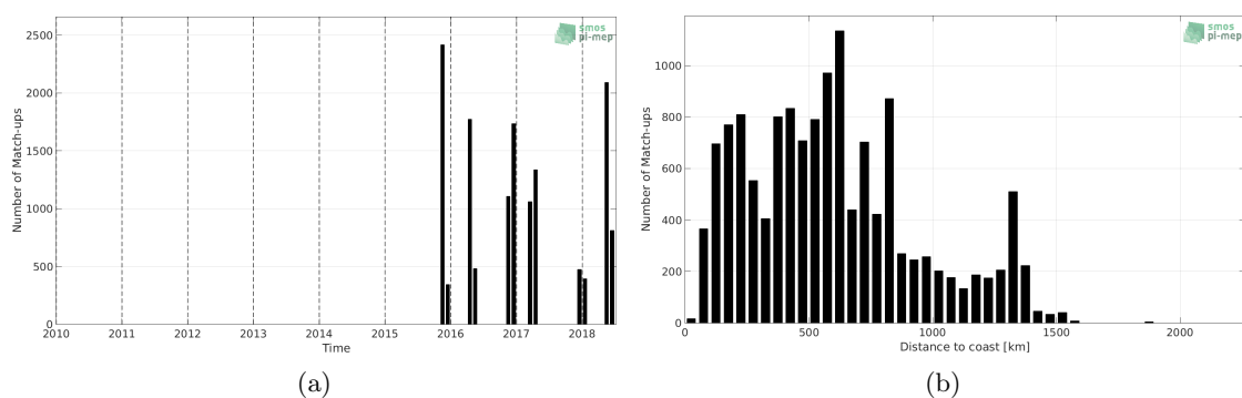
Figure 1: Number of match-ups between TSG-POLARSTERN and SMAP-L2-RSS-V3-70KM SSS as a function of time (a) and as function of the distance to coast (b) over the Mid-Low Latitudes 45N-45S Pi-MEP region and for the full satellite product period.
