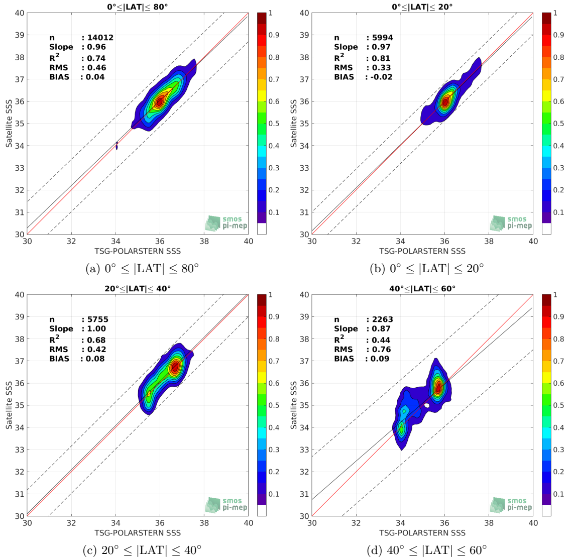
Figure 9: Contour maps of the concentration of SMAP-L2-RSS-V3-70KM SSS (y-axis) versus TSG-POLARSTERN SSS (x-axis) at match-up pairs for different latitude bands. For each plot, the red line shows x=y . The black thin and dashed lines indicate a linear fit through the data cloud and the \pm 95\% confidence levels, respectively. The number match-up pairs n , the slope and R^2 coefficient of the linear fit, the root mean square (RMS) and the mean bias between satellite and in situ data are indicated for each latitude band in each plots.
