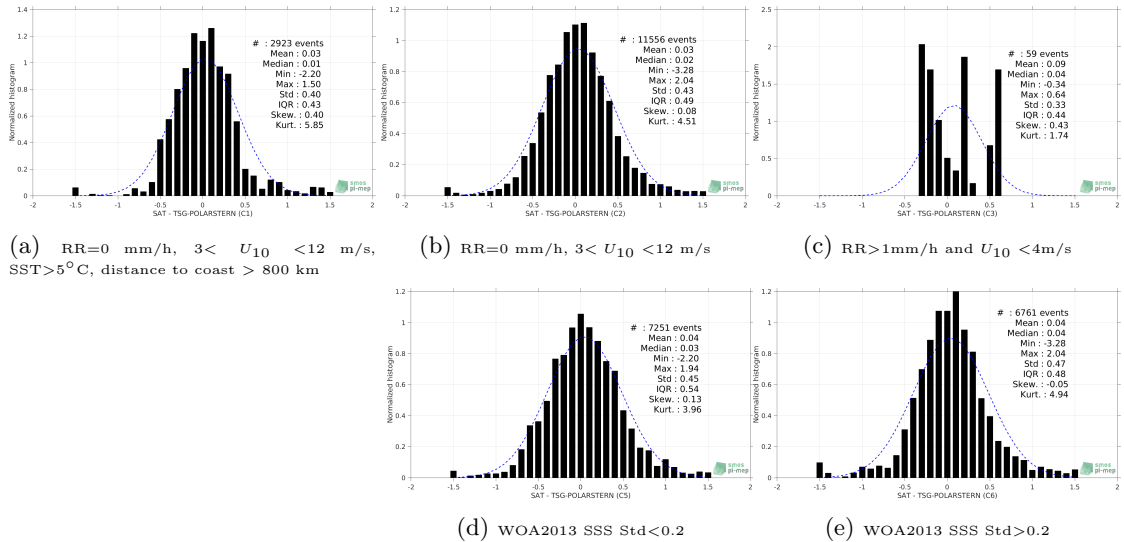
Figure 13: Normalized histogram of \Delta SSS (SMAP-L2-RSS-V3-70KM - TSG-POLARSTERN) for 5 different subdatasets corresponding to: RR=0 mm/h, 3 < U_{10} < 12 m/s, SST > 5^\circ\text{C} , distance to coast > 800 km (a), RR=0 mm/h, 3 < U_{10} < 12 m/s (b), RR >1 mm/h and U_{10} < 4 m/s (c), WOA2013 SSS Std <0.2 (d), WOA2013 SSS Std >0.2 (e).
