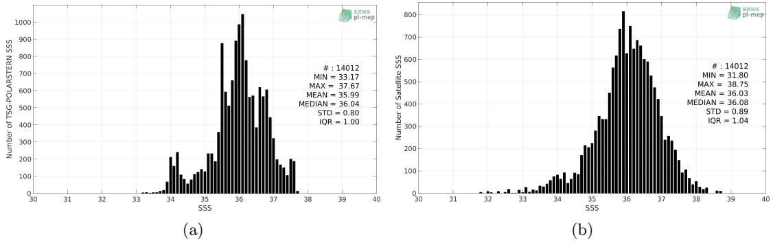
Figure 2: Histograms of SSS from TSG-POLARSTERN (a) and SMAP-L2-RSS-V3-70KM (b) considering all match-up pairs per bins of 0.1 over the Mid-Low Latitudes 45N-45S Pi-MEP region and for the full satellite product period.
