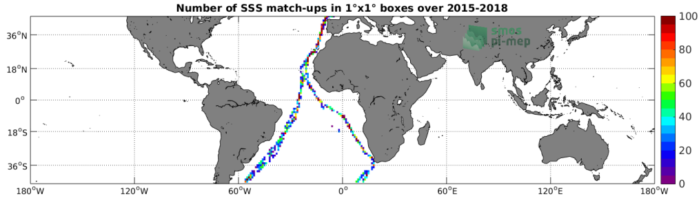
Figure 4: Number of SSS match-ups between TSG-POLARSTERN SSS and the SMAP-L2-RSS-V3-70KM SSS product for the Mid-Low Latitudes 45N-45S Pi-MEP region over 1°x1° boxes and for the full satellite product period.
