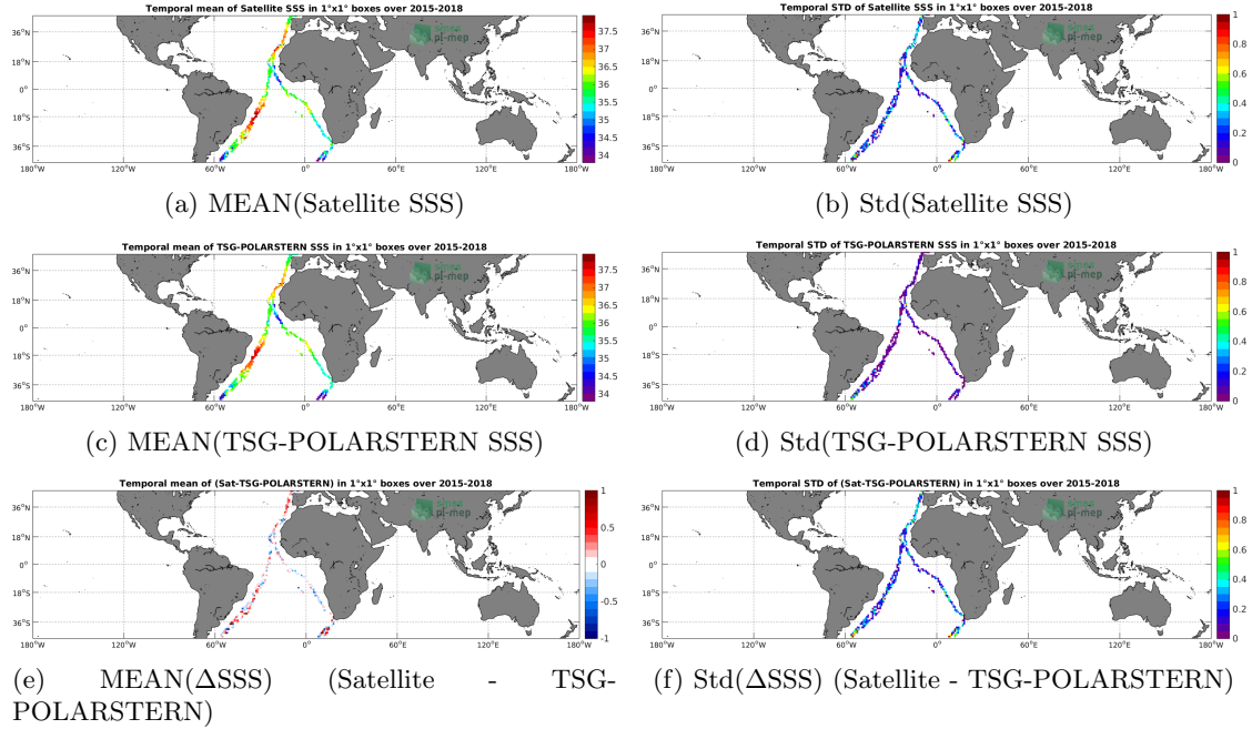
Figure 6: Temporal mean (left) and Std (right) of SSS from SMAP-L2-RSS-V3-70KM (top), TSG-POLARSTERN (middle), and of \Delta SSS (Satellite - TSG-POLARSTERN). Only match-up pairs are used to generate these maps.
