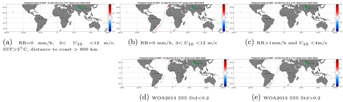
Figure 12: Temporal mean gridded over spatial boxes of size 1^\circ \times 1^\circ of \Delta SSS (SMAP-L2-RSS-V3-70KM - TSG-POLARSTERN) for 5 different subdatasets corresponding to:RR=0 mm/h, 3 < U_{10} < 12 m/s, SST > 5^\circ\text{C} , distance to coast > 800 km (a), RR=0 mm/h, 3 < U_{10} < 12 m/s (b), RR >1 mm/h and U_{10} < 4 m/s (c), WOA2013 SSS Std <0.2 (d), WOA2013 SSS Std >0.2 (e).
