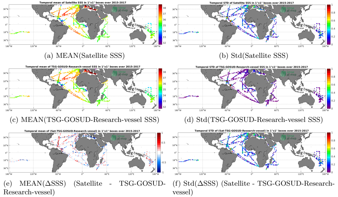
Figure 6: Temporal mean (left) and Std (right) of SSS from SMAP-L2-RSS-V3-70KM (top), TSG-GOSUD-Research-vessel (middle), and of \Delta SSS (Satellite - TSG-GOSUD-Research-vessel). Only match-up pairs are used to generate these maps.
