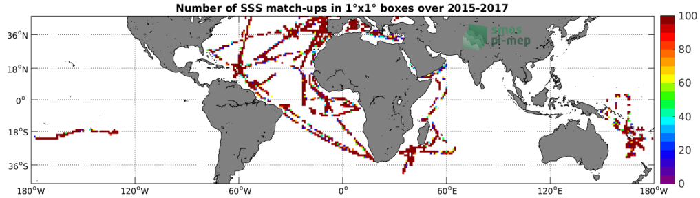
Figure 4: Number of SSS match-ups between TSG-GOSUD-Research-vessel SSS and the SMAP-L2-RSS-V3-70KM SSS product for the Mid-Low Latitudes 45N-45S Pi-MEP region over 1^\circ \times 1^\circ boxes and for the full satellite product period.
