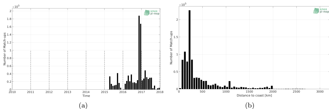
Figure 1: Number of match-ups between TSG-GOSUD-Research-vessel and SMAP-L2-RSS-V3-70KM SSS as a function of time (a) and as function of the distance to coast (b) over the Mid-Low Latitudes 45N-45S Pi-MEP region and for the full satellite product period.
