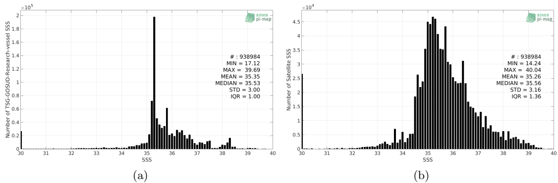
Figure 2: Histograms of SSS from TSG-GOSUD-Research-vessel (a) and SMAP-L2-RSS-V3-70KM (b) considering all match-up pairs per bins of 0.1 over the Mid-Low Latitudes 45N-45S Pi-MEP region and for the full satellite product period.
