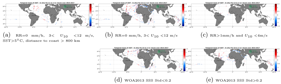
Figure 12: Temporal mean gridded over spatial boxes of size 1^\circ \times 1^\circ of \Delta SSS (SMAP-L2-RSS-V3-70KM - TSG-GOSUD-Research-vessel) for 5 different subdatasets corresponding to:RR=0 mm/h, 3 < U_{10} < 12 m/s, SST > 5^\circ\text{C} , distance to coast > 800 km (a), RR=0 mm/h, 3 < U_{10} < 12 m/s (b), RR > 1 mm/h and U_{10} < 4 m/s (c), WOA2013 SSS Std < 0.2 (d), WOA2013 SSS Std > 0.2 (e).
