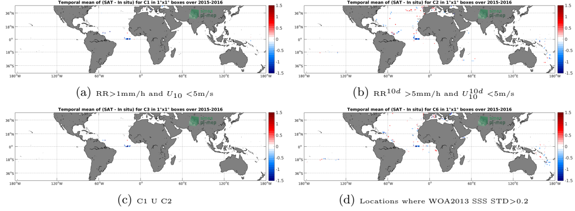
Figure 12: Temporal mean gridded over spatial boxes of size 1^\circ \times 1^\circ of \Delta SSS (SMAP-L2-RSS-V3-70KM - TSG-GOSUD-Research-vessel) for 4 different subdatasets corresponding to: RR > 1\text{mm/h} and U_{10} < 5\text{m/s} (a), RR^{10d} > 5\text{mm/h} and U_{10}^{10d} < 5\text{m/s} (b), C1 U C2 (c), Locations where WOA2013 SSS STD > 0.2 (d).
