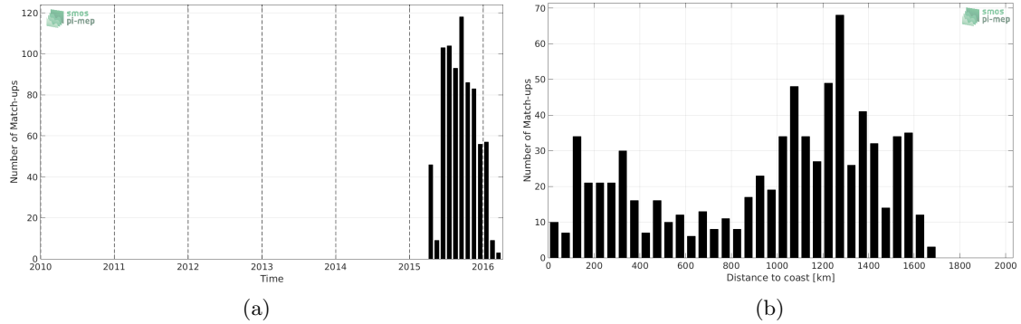
Figure 1: Number of match-ups between Sea mammals and SMAP-L2-RSS-V3-70KM SSS as a function of time (a) and as function of the distance to coast (b) over the Mid-Low Latitudes 45N-45S Pi-MEP region and for the full satellite product period.
