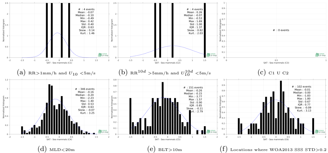
Figure 13: Normalized histogram of \Delta SSS (SMAP-L2-RSS-V3-70KM - Sea mammals) for 6 different subdatasets corresponding to: RR>1mm/h and U_{10} < 5m/s (a), RR^{10d} > 5mm/h and U_{10}^{10d} < 5m/s (b), C1 U C2 (c),MLD<20m (d),BLT>10m (e),Locations where WOA2013 SSS STD>0.2 (f).
