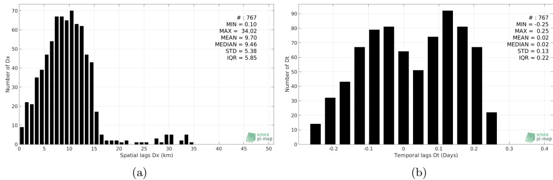
Figure 5: Histograms of the spatial (a) and temporal (b) lags between the time of the Sea mammals measurements and the date of the corresponding SMAP-L2-RSS-V3-70KM SSS product.
