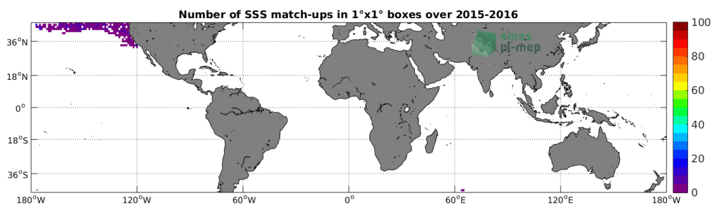
Figure 4: Number of SSS match-ups between Sea mammals SSS and the SMAP-L2-RSS-V3-70KM SSS product for the Mid-Low Latitudes 45N-45S Pi-MEP region over 1^\circ \times 1^\circ boxes and for the full satellite product period.
