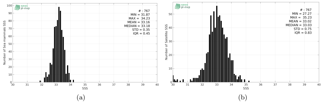
Figure 2: Histograms of SSS from Sea mammals (a) and SMAP-L2-RSS-V3-70KM (b) considering all match-up pairs per bins of 0.1 over the Mid-Low Latitudes 45N-45S Pi-MEP region and for the full satellite product period.
