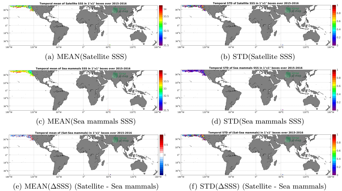
Figure 6: Temporal mean (left) and STD (right) of SSS from SMAP-L2-RSS-V3-70KM (top), Sea mammals (middle), and of \Delta SSS (Satellite - Sea mammals). Only match-up pairs are used to generate these maps.
