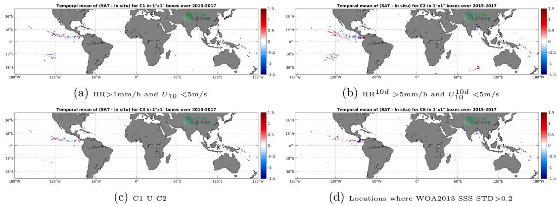
Figure 11: Temporal mean gridded over spatial boxes of size 1^\circ \times 1^\circ of \Delta SSS (SMAP-L2-RSS-V3-70KM - Surface drifters) for 4 different subdatasets corresponding to: RR > 1\text{mm/h} and U_{10} < 5\text{m/s} (a), RR^{10d} > 5\text{mm/h} and U_{10}^{10d} < 5\text{m/s} (b), C1 U C2 (c), Locations where WOA2013 SSS STD > 0.2 (d).
