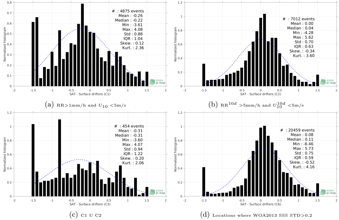
Figure 12: Normalized histogram of \Delta\text{SSS} (SMAP-L2-RSS-V3-70KM - Surface drifters) for 6 different subdatasets corresponding to: \text{RR} > 1\text{mm/h} and U_{10} < 5\text{m/s} (a), \text{RR}^{10d} > 5\text{mm/h} and U_{10}^{10d} < 5\text{m/s} (b), C1 U C2 (c), Locations where WOA2013 SSS STD > 0.2 (d).
