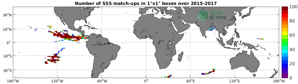
Figure 3: Number of SSS match-ups between Surface drifters SSS and the SMAP-L2-RSS-V3-70KM SSS product for the Mid-Low Latitudes 45N-45S Pi-MEP region over 1°x1° boxes and for the full satellite product period.
