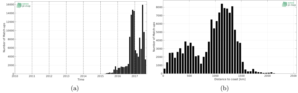
Figure 1: Number of match-ups between Surface drifters and SMAP-L2-RSS-V3-70KM SSS as a function of time (a) and as function of the distance to coast (b) over the Mid-Low Latitudes 45N-45S Pi-MEP region and for the full satellite product period.
