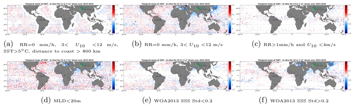
Figure 12: Temporal mean gridded over spatial boxes of size 1^\circ \times 1^\circ of \Delta SSS (SMAP-L2-RSS-V3-70KM - Argo) for 6 different subdatasets corresponding to:RR=0 mm/h, 3 < U_{10} < 12 m/s, SST >5^\circ C, distance to coast > 800 km (a), RR=0 mm/h, 3 < U_{10} < 12 m/s (b), RR >1 mm/h and U_{10} < 4 m/s (c),MLD <20 m (d),WOA2013 SSS Std <0.2 (e),WOA2013 SSS Std >0.2 (f).
