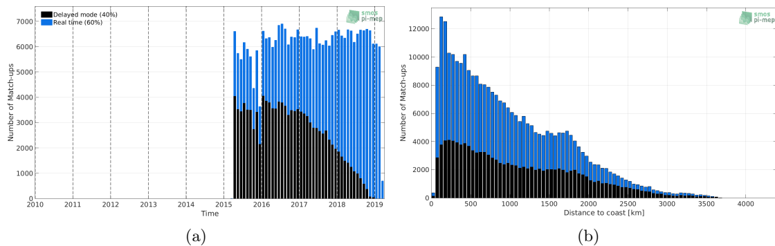
Figure 1: Number of match-ups between Argo and SMAP-L2-RSS-V3-70KM SSS as a function of time (a) and as function of the distance to coast (b) over the Mid-Low Latitudes 45N-45S Pi-MEP region and for the full satellite product period.
