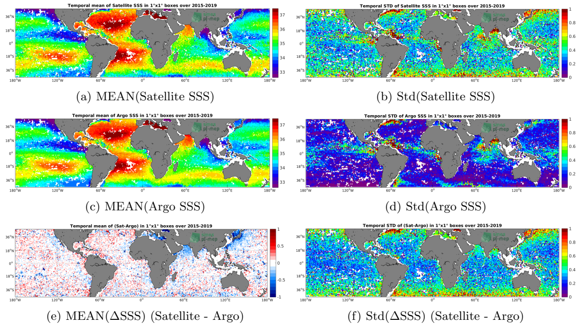
Figure 6: Temporal mean (left) and Std (right) of SSS from SMAP-L2-RSS-V3-70KM (top), Argo (middle), and of \Delta SSS (Satellite - Argo). Only match-up pairs are used to generate these maps.
