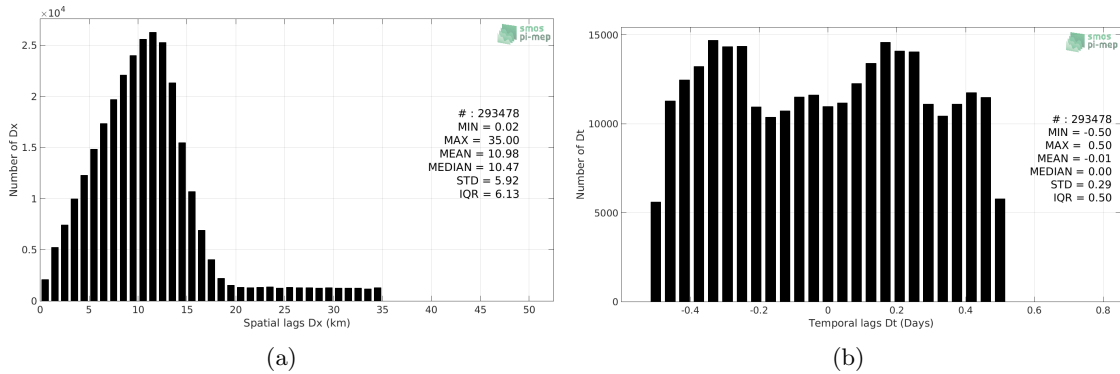
Figure 5: Histograms of the spatial (a) and temporal (b) lags between the time of the Argo measurements and the date of the corresponding SMAP-L2-RSS-V3-70KM SSS product.
