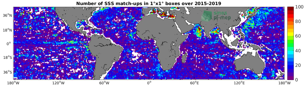
Figure 4: Number of SSS match-ups between Argo SSS and the SMAP-L2-RSS-V3-70KM SSS product for the Mid-Low Latitudes 45N-45S Pi-MEP region over 1^\circ \times 1^\circ boxes and for the full satellite product period.
