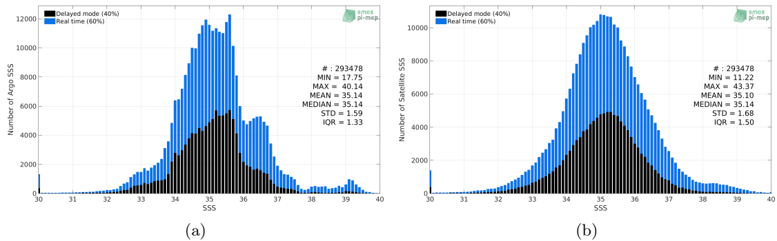
Figure 2: Histograms of SSS from Argo (a) and SMAP-L2-RSS-V3-70KM (b) considering all match-up pairs per bins of 0.1 over the Mid-Low Latitudes 45N-45S Pi-MEP region and for the full satellite product period.
