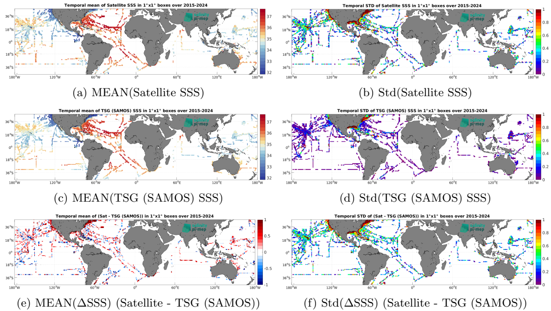
Figure 7: Temporal mean (left) and Std (right) of SSS from SMAP SSS L2 v5.0 (JPL) (top), TSG (SAMOS) (middle), and of \Delta SSS (Satellite - TSG (SAMOS)). Only match-up pairs are used to generate these maps.
