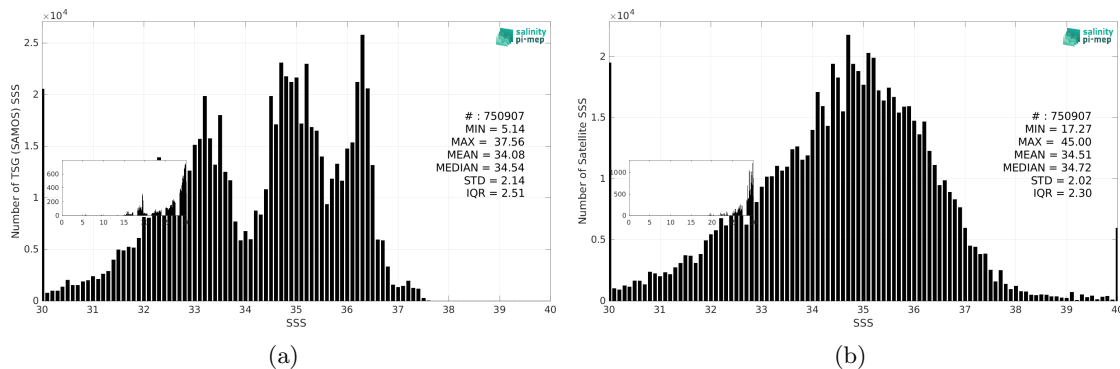
Figure 3: Histograms of SSS from TSG (SAMOS) (a) and SMAP SSS L2 v5.0 (JPL) (b) considering all match-up pairs per bins of 0.1 over the Mid-Low Latitudes 45N-45S Pi-MEP region and for the full satellite product period.
