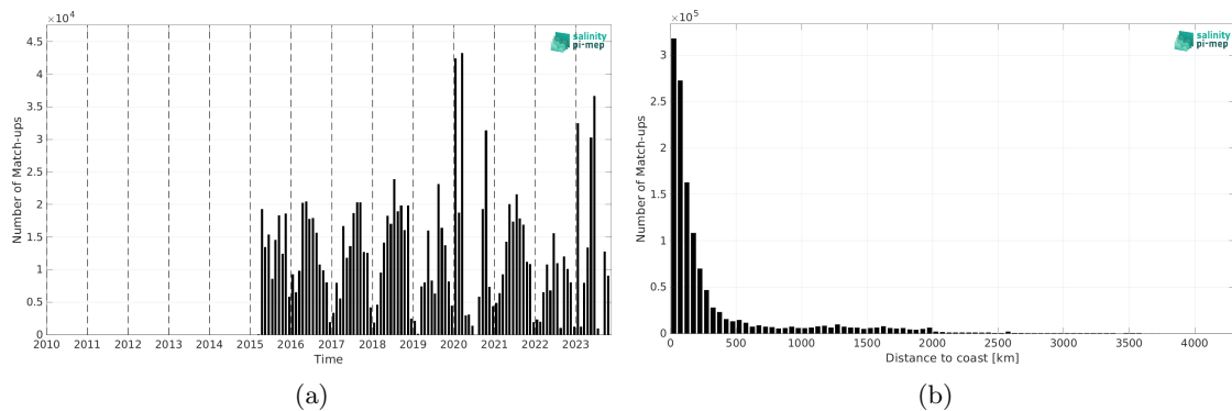
Figure 1: Number of match-ups between TSG (SAMOS) and SMAP SSS L2 v5.0 (JPL) SSS as a function of time (a) and as function of the distance to coast (b) over the Mid-Low Latitudes 45N-45S Pi-MEP region and for the full satellite product period.
