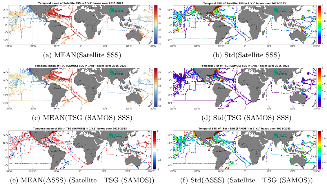
Figure 6: Temporal mean (left) and Std (right) of SSS from SMAP SSS L2 v5.0 (JPL) (top), TSG (SAMOS) (middle), and of \Delta SSS (Satellite - TSG (SAMOS)). Only match-up pairs are used to generate these maps.
