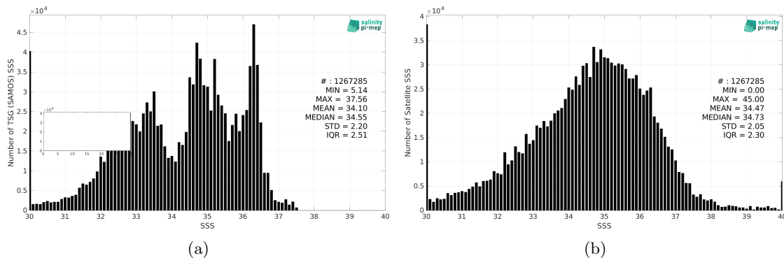
Figure 2: Histograms of SSS from TSG (SAMOS) (a) and SMAP SSS L2 v5.0 (JPL) (b) considering all match-up pairs per bins of 0.1 over the Mid-Low Latitudes 45N-45S Pi-MEP region and for the full satellite product period.
