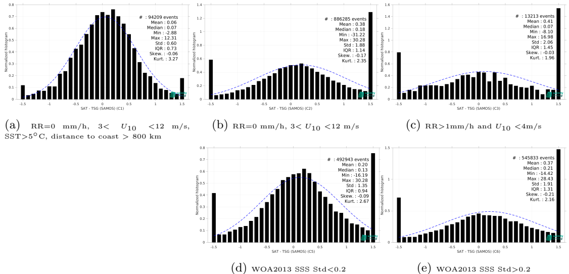
Figure 13: Normalized histogram of \Delta SSS (SMAP SSS L2 v5.0 (JPL) - TSG (SAMOS)) for 5 different subdatasets corresponding to: RR=0 mm/h, 3 < U_{10} < 12 m/s, SST >5^\circ\text{C} , distance to coast > 800 km (a), RR=0 mm/h, 3 < U_{10} < 12 m/s (b), RR >1 mm/h and U_{10} < 4 m/s (c), WOA2013 SSS Std <0.2 (d), WOA2013 SSS Std >0.2 (e).
