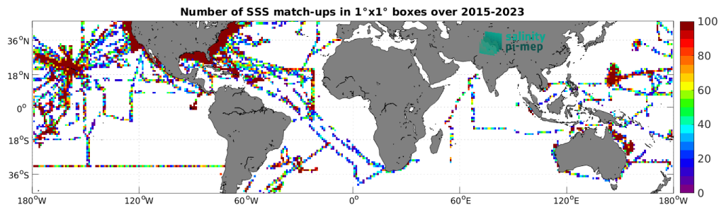
Figure 4: Number of SSS match-ups between TSG (SAMOS) SSS and the SMAP SSS L2 v5.0 (JPL) SSS product for the Mid-Low Latitudes 45N-45S Pi-MEP region over 1^\circ \times 1^\circ boxes and for the full satellite product period.
