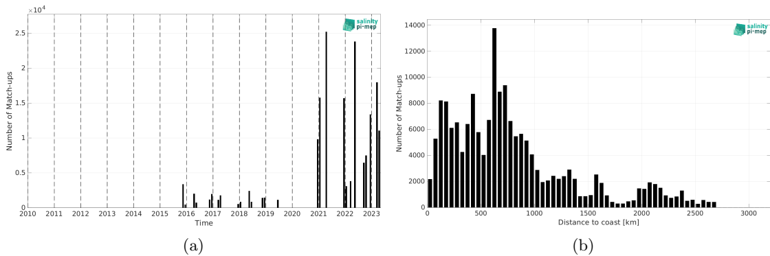
Figure 2: Number of match-ups between TSG (Polarstern) and SMAP SSS L2 v5.0 (JPL) SSS as a function of time (a) and as function of the distance to coast (b) over the Mid-Low Latitudes 45N-45S Pi-MEP region and for the full satellite product period.
