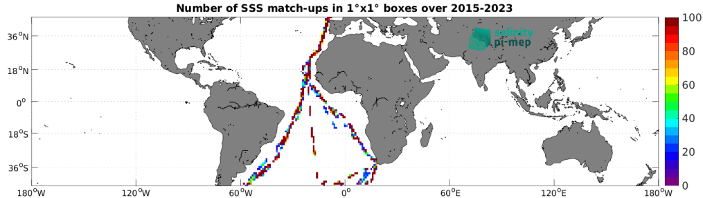
Figure 5: Number of SSS match-ups between TSG (Polarstern) SSS and the SMAP SSS L2 v5.0 (JPL) SSS product for the Mid-Low Latitudes 45N-45S Pi-MEP region over 1^\circ \times 1^\circ boxes and for the full satellite product period.
