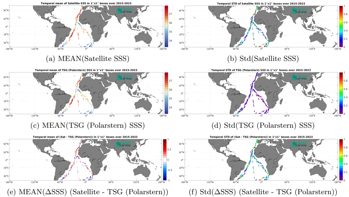
Figure 7: Temporal mean (left) and Std (right) of SSS from SMAP SSS L2 v5.0 (JPL) (top), TSG (Polarstern) (middle), and of \Delta SSS (Satellite - TSG (Polarstern)). Only match-up pairs are used to generate these maps.
