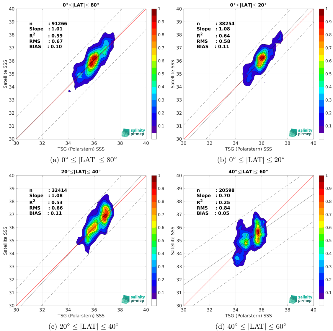
Figure 10: Contour maps of the concentration of SMAP SSS L2 v5.0 (JPL) SSS (y-axis) versus TSG (Polarstern) SSS (x-axis) at match-up pairs for different latitude bands. For each plot, the red line shows x=y . The black thin and dashed lines indicate a linear fit through the data cloud and the \pm 95\% confidence levels, respectively. The number match-up pairs n , the slope and R^2 coefficient of the linear fit, the root mean square (RMS) and the mean bias between satellite and in situ data are indicated for each latitude band in each plots.
