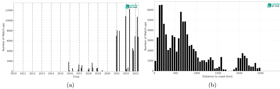
Figure 2: Number of match-ups between TSG (Polarstern) and SMAP SSS L2 v5.0 (JPL) SSS as a function of time (a) and as function of the distance to coast (b) over the Mid-Low Latitudes 45N-45S Pi-MEP region and for the full satellite product period.
