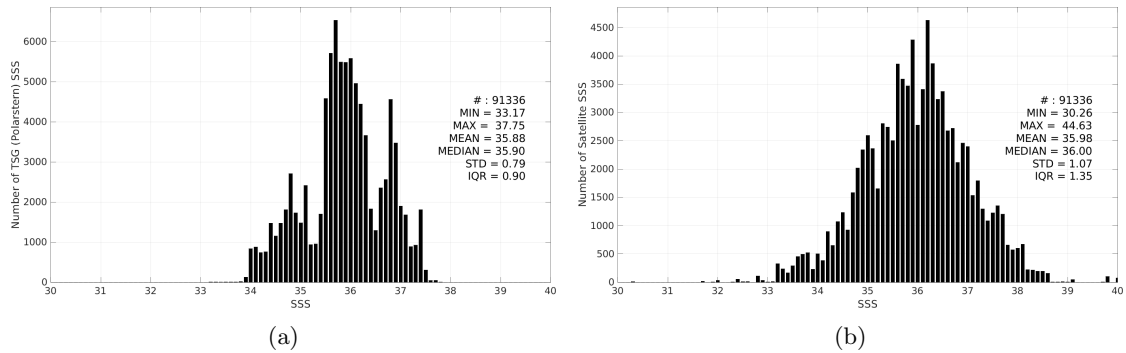
Figure 3: Histograms of SSS from TSG (Polarstern) (a) and SMAP SSS L2 v5.0 (JPL) (b) considering all match-up pairs per bins of 0.1 over the Mid-Low Latitudes 45N-45S Pi-MEP region and for the full satellite product period.
