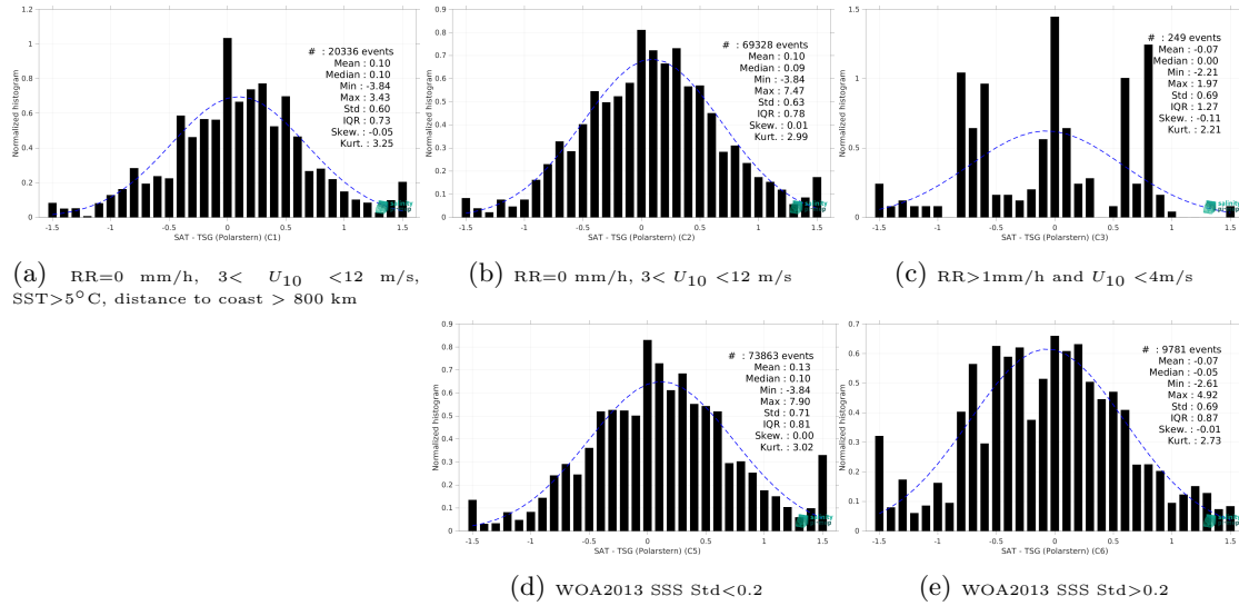
Figure 15: Normalized histogram of \Delta\text{SSS} (SMAP SSS L2 v5.0 (JPL) - TSG (Polarstern)) for 5 different subdatasets corresponding to: RR=0 mm/h, 3 < U_{10} < 12 m/s, SST>5°C, distance to coast > 800 km (a), RR=0 mm/h, 3 < U_{10} < 12 m/s (b), RR>1mm/h and U_{10} < 4 m/s (c), WOA2013 SSS Std<0.2 (d), WOA2013 SSS Std>0.2 (e).
