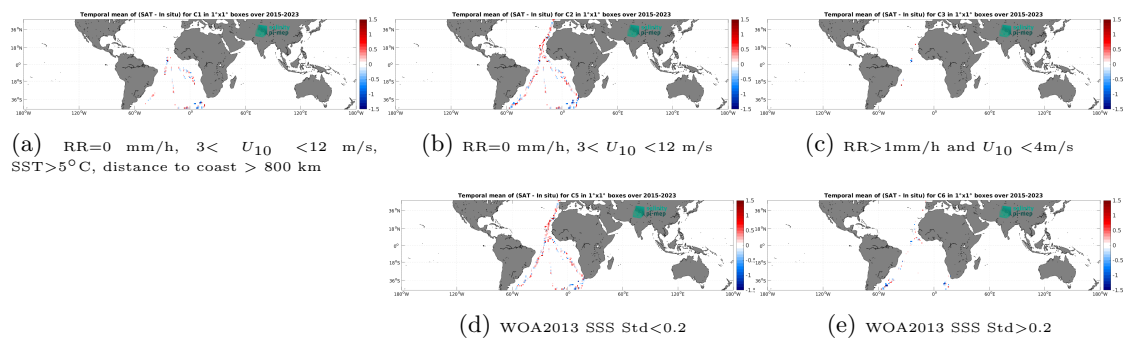
Figure 14: Temporal mean gridded over spatial boxes of size 1^\circ \times 1^\circ of \Delta SSS (SMAP SSS L2 v5.0 (JPL) - TSG (Polarstern)) for 5 different subdatasets corresponding to: RR=0 mm/h, 3 < U_{10} < 12 m/s, SST > 5°C, distance to coast > 800 km (a), RR=0 mm/h, 3 < U_{10} < 12 m/s (b), RR > 1mm/h and U_{10} < 4 m/s (c), WOA2013 SSS Std < 0.2 (d), WOA2013 SSS Std > 0.2 (e).
