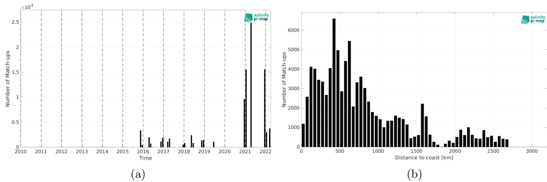
Figure 1: Number of match-ups between TSG (Polarstern) and SMAP SSS L2 v5.0 (JPL) SSS as a function of time (a) and as function of the distance to coast (b) over the Mid-Low Latitudes 45N-45S Pi-MEP region and for the full satellite product period.
