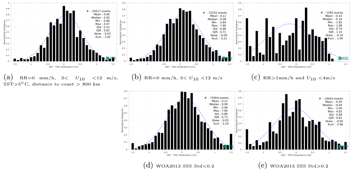
Figure 13: Normalized histogram of \Delta\text{SSS} (SMAP SSS L2 v5.0 (JPL) - TSG (Polarstern)) for 5 different subdatasets corresponding to: RR=0 mm/h, 3 < U_{10} < 12 m/s, SST >5^\circ\text{C} , distance to coast > 800 km (a), RR=0 mm/h, 3 < U_{10} < 12 m/s (b), RR >1 mm/h and U_{10} < 4 m/s (c), WOA2013 SSS Std <0.2 (d), WOA2013 SSS Std >0.2 (e).
