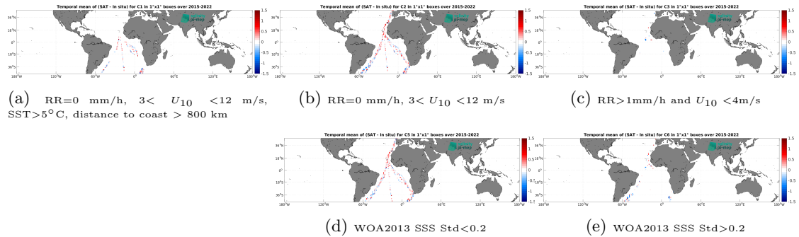
Figure 12: Temporal mean gridded over spatial boxes of size 1^\circ \times 1^\circ of \Delta\text{SSS} (SMAP SSS L2 v5.0 (JPL) - TSG (Polarstern)) for 5 different subdatasets corresponding to:RR=0 mm/h, 3 < U_{10} < 12 m/s, SST >5^\circ\text{C} , distance to coast > 800 km (a), RR=0 mm/h, 3 < U_{10} < 12 m/s (b), RR >1 mm/h and U_{10} < 4 m/s (c), WOA2013 SSS Std <0.2 (d), WOA2013 SSS Std >0.2 (e).
