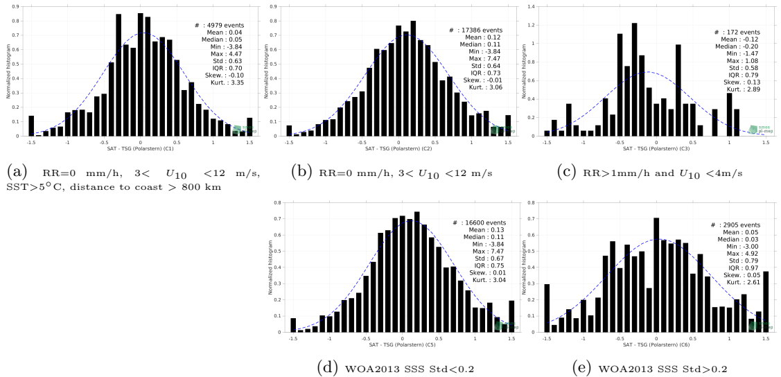
Figure 13: Normalized histogram of \Delta SSS (SMAP SSS L2 v5.0 (JPL) - TSG (Polarstern)) for 5 different subdatasets corresponding to: RR=0 mm/h, 3 < U_{10} < 12 m/s, SST >5^\circ\text{C} , distance to coast > 800 km (a), RR=0 mm/h, 3 < U_{10} < 12 m/s (b), RR >1 mm/h and U_{10} < 4 m/s (c), WOA2013 SSS Std <0.2 (d), WOA2013 SSS Std >0.2 (e).
