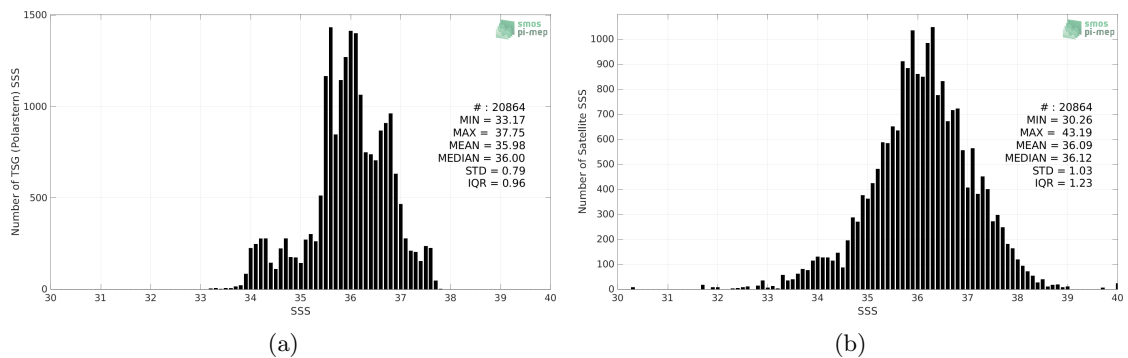
Figure 2: Histograms of SSS from TSG (Polarstern) (a) and SMAP SSS L2 v5.0 (JPL) (b) considering all match-up pairs per bins of 0.1 over the Mid-Low Latitudes 45N-45S Pi-MEP region and for the full satellite product period.
