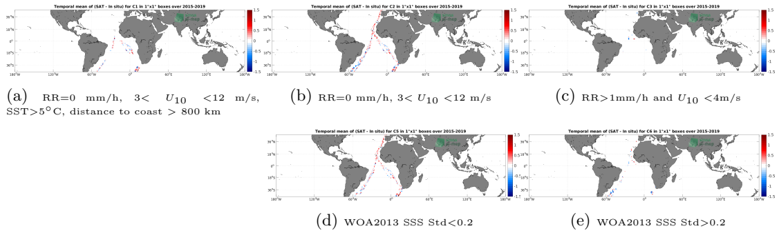
Figure 12: Temporal mean gridded over spatial boxes of size 1^\circ \times 1^\circ of \Delta SSS (SMAP SSS L2 v5.0 (JPL) - TSG (Polarstern)) for 5 different subdatasets corresponding to:RR=0 mm/h, 3 < U_{10} < 12 m/s, SST >5^\circ\text{C} , distance to coast > 800 km (a), RR=0 mm/h, 3 < U_{10} < 12 m/s (b), RR >1 mm/h and U_{10} < 4 m/s (c), WOA2013 SSS Std <0.2 (d), WOA2013 SSS Std >0.2 (e).
