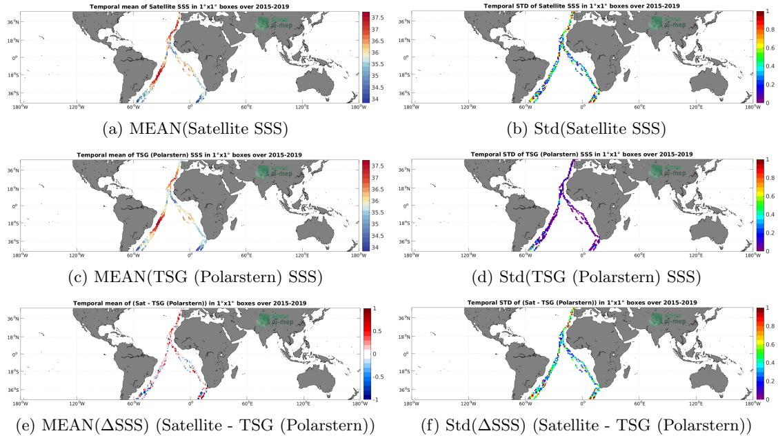
Figure 6: Temporal mean (left) and Std (right) of SSS from SMAP SSS L2 v5.0 (JPL) (top), TSG (Polarstern) (middle), and of \Delta SSS (Satellite - TSG (Polarstern)). Only match-up pairs are used to generate these maps.
