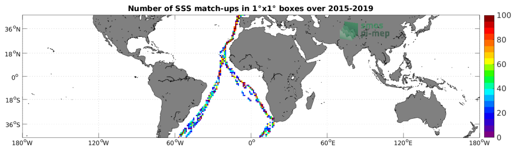
Figure 4: Number of SSS match-ups between TSG (Polarstern) SSS and the SMAP SSS L2 v5.0 (JPL) SSS product for the Mid-Low Latitudes 45N-45S Pi-MEP region over 1^\circ \times 1^\circ boxes and for the full satellite product period.
