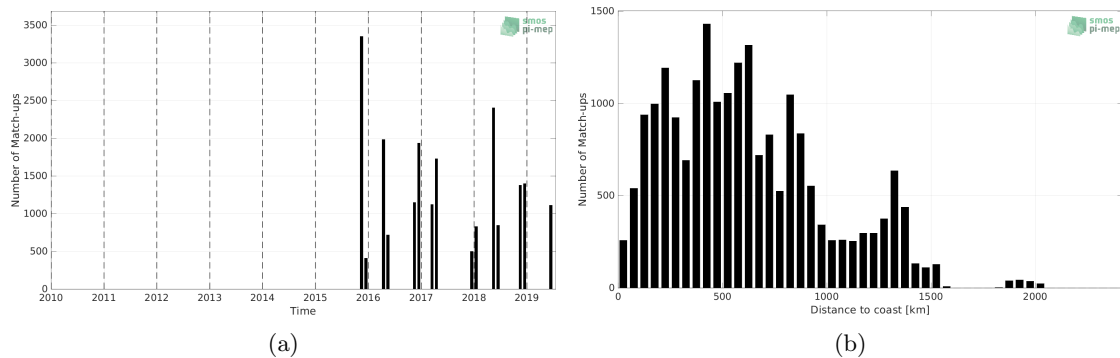
Figure 1: Number of match-ups between TSG (Polarstern) and SMAP SSS L2 v5.0 (JPL) SSS as a function of time (a) and as function of the distance to coast (b) over the Mid-Low Latitudes 45N-45S Pi-MEP region and for the full satellite product period.
