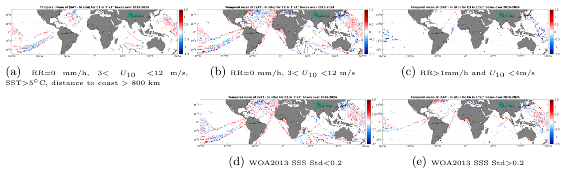
Figure 14: Temporal mean gridded over spatial boxes of size 1^\circ \times 1^\circ of \Delta\text{SSS} (SMAP SSS L2 v5.0 (JPL) - TSG (LEGOS-DM)) for 5 different subdatasets corresponding to: RR=0 mm/h, 3 < U_{10} < 12 m/s, SST > 5°C, distance to coast > 800 km (a), RR=0 mm/h, 3 < U_{10} < 12 m/s (b), RR > 1mm/h and U_{10} < 4 m/s (c), WOA2013 SSS Std < 0.2 (d), WOA2013 SSS Std > 0.2 (e).
