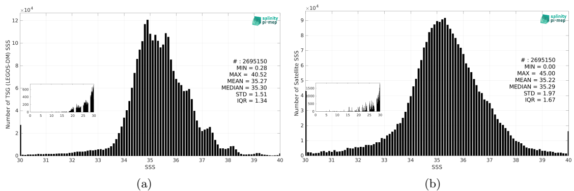
Figure 3: Histograms of SSS from TSG (LEGOS-DM) (a) and SMAP SSS L2 v5.0 (JPL) (b) considering all match-up pairs per bins of 0.1 over the Mid-Low Latitudes 45N-45S Pi-MEP region and for the full satellite product period.
