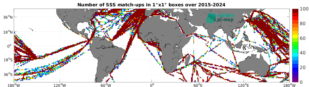
Figure 5: Number of SSS match-ups between TSG (LEGOS-DM) SSS and the SMAP SSS L2 v5.0 (JPL) SSS product for the Mid-Low Latitudes 45N-45S Pi-MEP region over 1^\circ \times 1^\circ boxes and for the full satellite product period.
