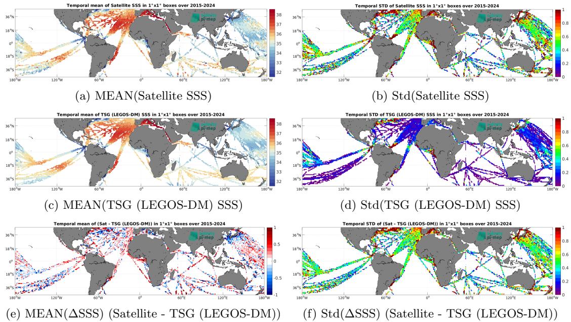
Figure 7: Temporal mean (left) and Std (right) of SSS from SMAP SSS L2 v5.0 (JPL) (top), TSG (LEGOS-DM) (middle), and of \Delta SSS (Satellite - TSG (LEGOS-DM)). Only match-up pairs are used to generate these maps.
