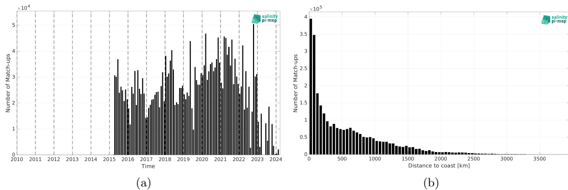
Figure 2: Number of match-ups between TSG (LEGOS-DM) and SMAP SSS L2 v5.0 (JPL) SSS as a function of time (a) and as function of the distance to coast (b) over the Mid-Low Latitudes 45N-45S Pi-MEP region and for the full satellite product period.
