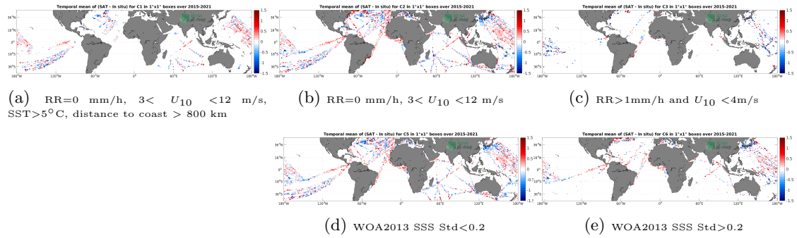
Figure 12: Temporal mean gridded over spatial boxes of size 1^\circ \times 1^\circ of \Delta SSS (SMAP SSS L2 v5.0 (JPL) - TSG (LEGOS-DM)) for 5 different subdatasets corresponding to: RR=0 mm/h, 3 < U_{10} < 12 m/s, SST>5°C, distance to coast > 800 km (a), RR=0 mm/h, 3 < U_{10} < 12 m/s (b), RR>1mm/h and U_{10} < 4 m/s (c), WOA2013 SSS Std<0.2 (d), WOA2013 SSS Std>0.2 (e).
