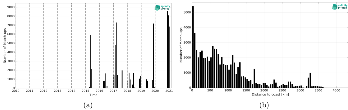
Figure 2: Number of match-ups between TSG (GOSUD-Sailing-ship) and SMAP SSS L2 v5.0 (JPL) SSS as a function of time (a) and as function of the distance to coast (b) over the Mid-Low Latitudes 45N-45S Pi-MEP region and for the full satellite product period.
