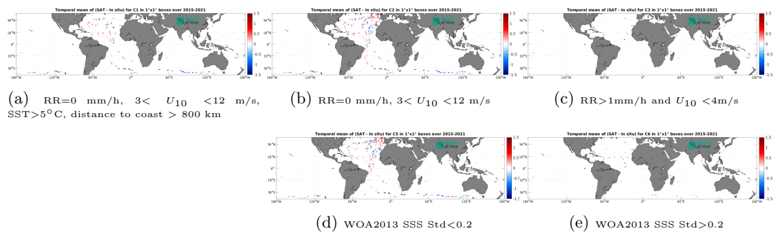
Figure 14: Temporal mean gridded over spatial boxes of size 1^\circ \times 1^\circ of \Delta\text{SSS} (SMAP SSS L2 v5.0 (JPL) - TSG (GOSUD-Sailing-ship)) for 5 different subdatasets corresponding to:RR=0 mm/h, 3 < U_{10} < 12 m/s, SST>5°C, distance to coast > 800 km (a), RR=0 mm/h, 3 < U_{10} < 12 m/s (b), RR>1mm/h and U_{10} < 4 m/s (c), WOA2013 SSS Std<0.2 (d), WOA2013 SSS Std>0.2 (e).
