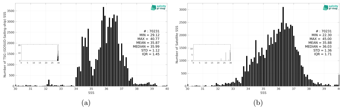
Figure 3: Histograms of SSS from TSG (GOSUD-Sailing-ship) (a) and SMAP SSS L2 v5.0 (JPL) (b) considering all match-up pairs per bins of 0.1 over the Mid-Low Latitudes 45N-45S Pi-MEP region and for the full satellite product period.
