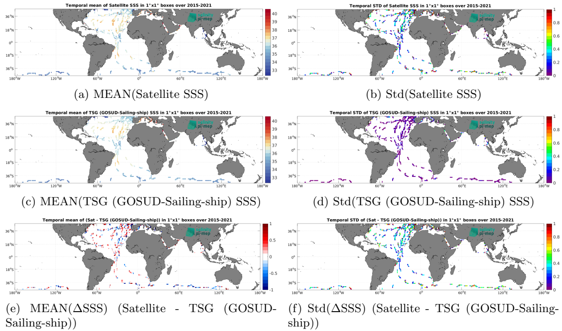
Figure 7: Temporal mean (left) and Std (right) of SSS from SMAP SSS L2 v5.0 (JPL) (top), TSG (GOSUD-Sailing-ship) (middle), and of \Delta SSS (Satellite - TSG (GOSUD-Sailing-ship)). Only match-up pairs are used to generate these maps.
