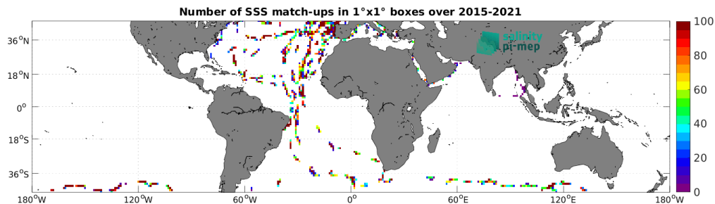
Figure 5: Number of SSS match-ups between TSG (GOSUD-Sailing-ship) SSS and the SMAP SSS L2 v5.0 (JPL) SSS product for the Mid-Low Latitudes 45N-45S Pi-MEP region over 1^\circ \times 1^\circ boxes and for the full satellite product period.
